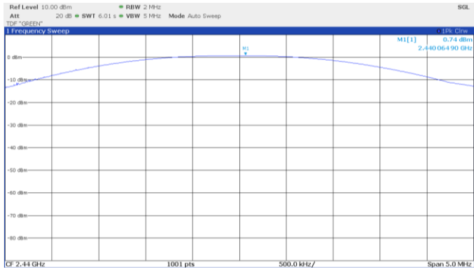
Figure 8.4-2: Conducted output power, 2440 MHz
