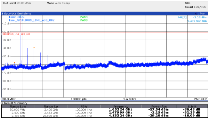
Figure 8.5-8: Antenna port conducted spurious emissions, 2480 MHz
