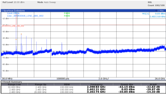
Figure 8.5-4: Antenna port conducted spurious emissions, 2402 MHz
