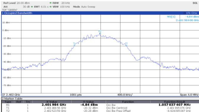
Figure 8.7-1: 99 % occupied bandwidth, 2402 MHz
