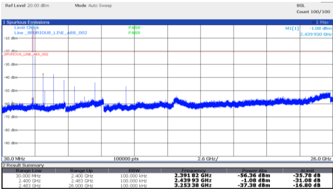
Figure 8.5-6: Antenna port conducted spurious emissions, 2440 MHz
