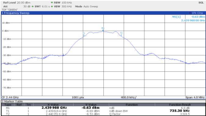
Figure 8.3-2: 6 dB DTS bandwidth, 2440 MHz
