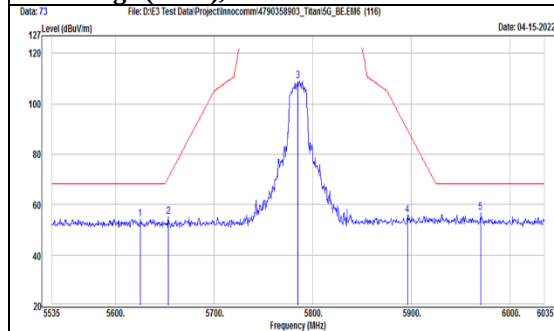
TX, 802.11ac(VHT20) (Ch 157) Band Edge (Peak), Horizontal
