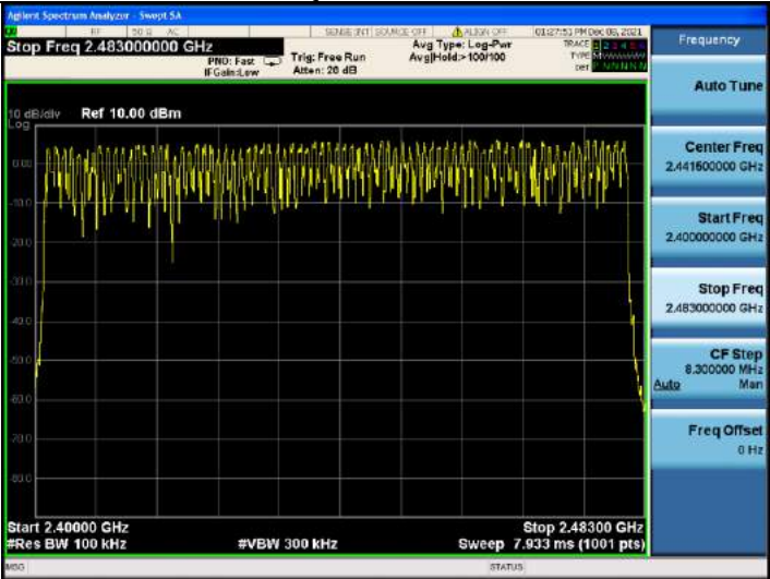
8DPSK Modulation
