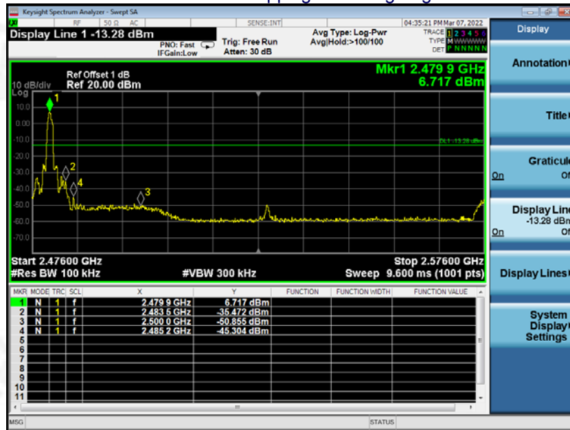
8DPSK No-hopping Band edge-right side
