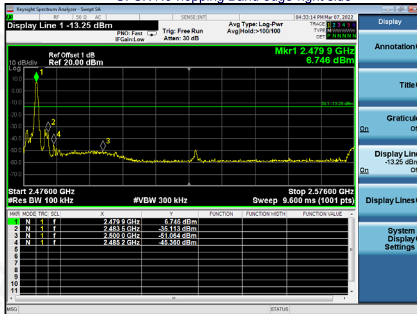
GFSK No-hopping Band edge-right side
