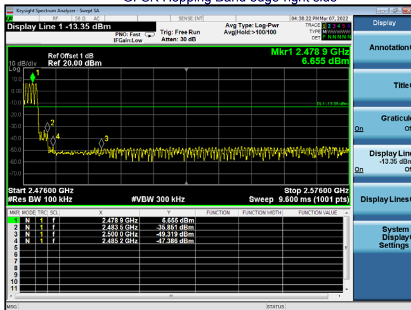
GFSK Hopping Band edge-right side
