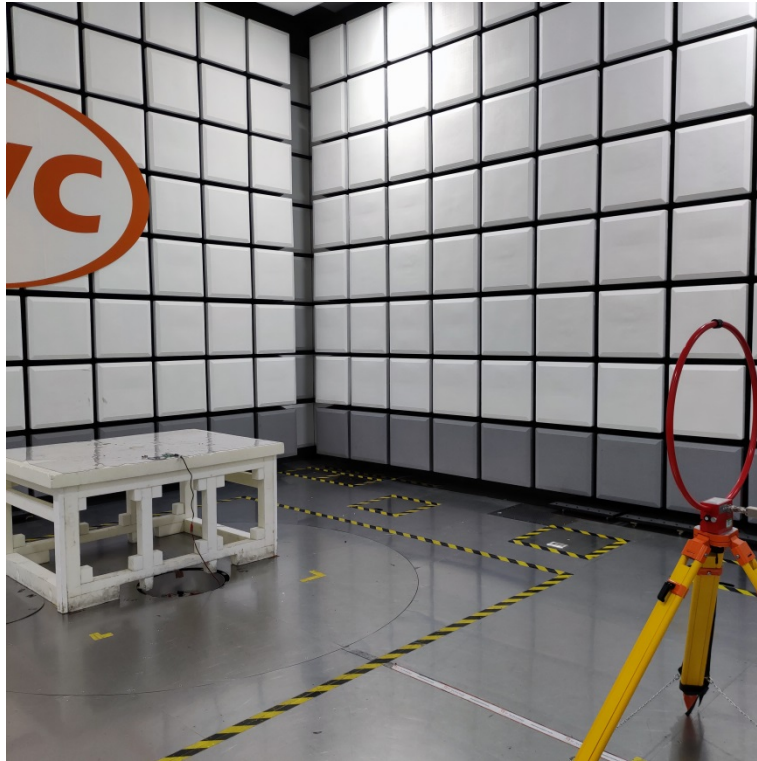
(2) Radiated spurious emission Test Setup(Below 1GHz)
