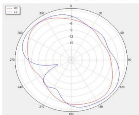
Theta=90 freq=2450MHz
