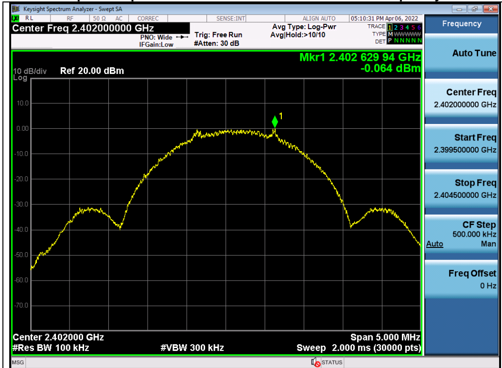
Test_Graph_LE2M_ANT1_2402_2Mbps_Reference Level
