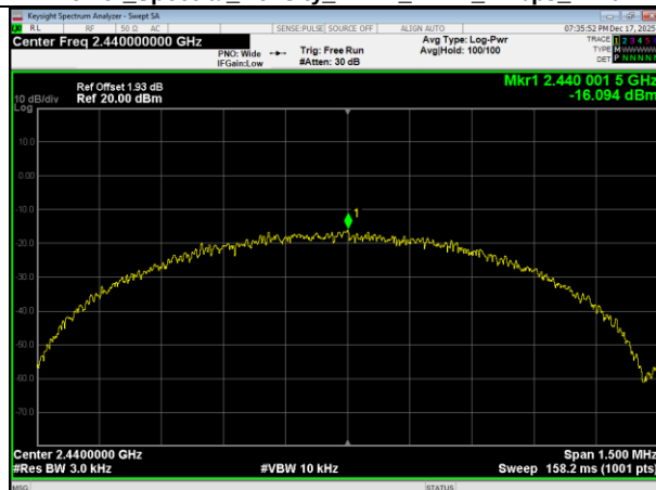
Power Spectral Density NVNT_ANT1_1Mbps_2440
