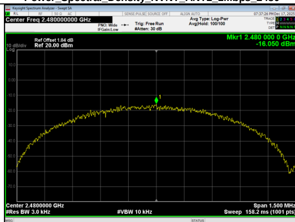
Power Spectral Density NVNT_ANT1_1Mbps_2480
