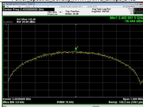
Power Spectral Density NVNT_ANT1_1Mbps_2402
