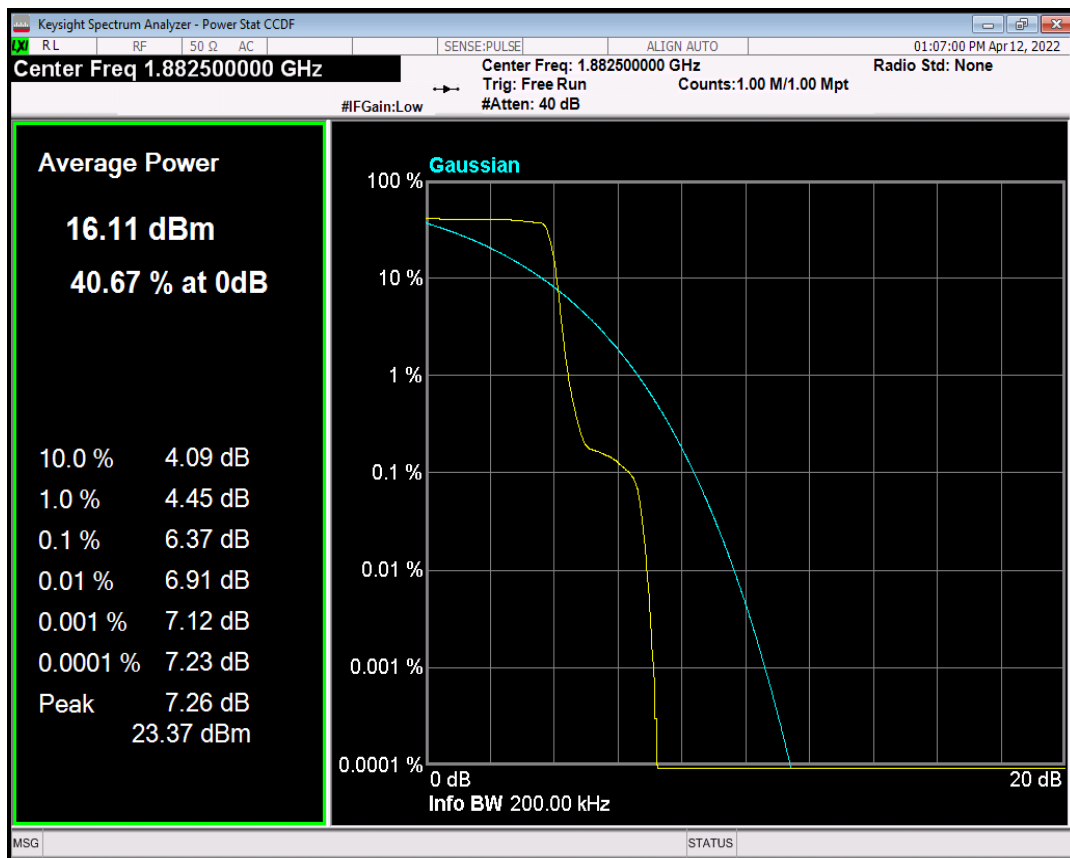
Band25 QPSK Channel=26365 nTones=1@0 Spacing=3.75kHz
