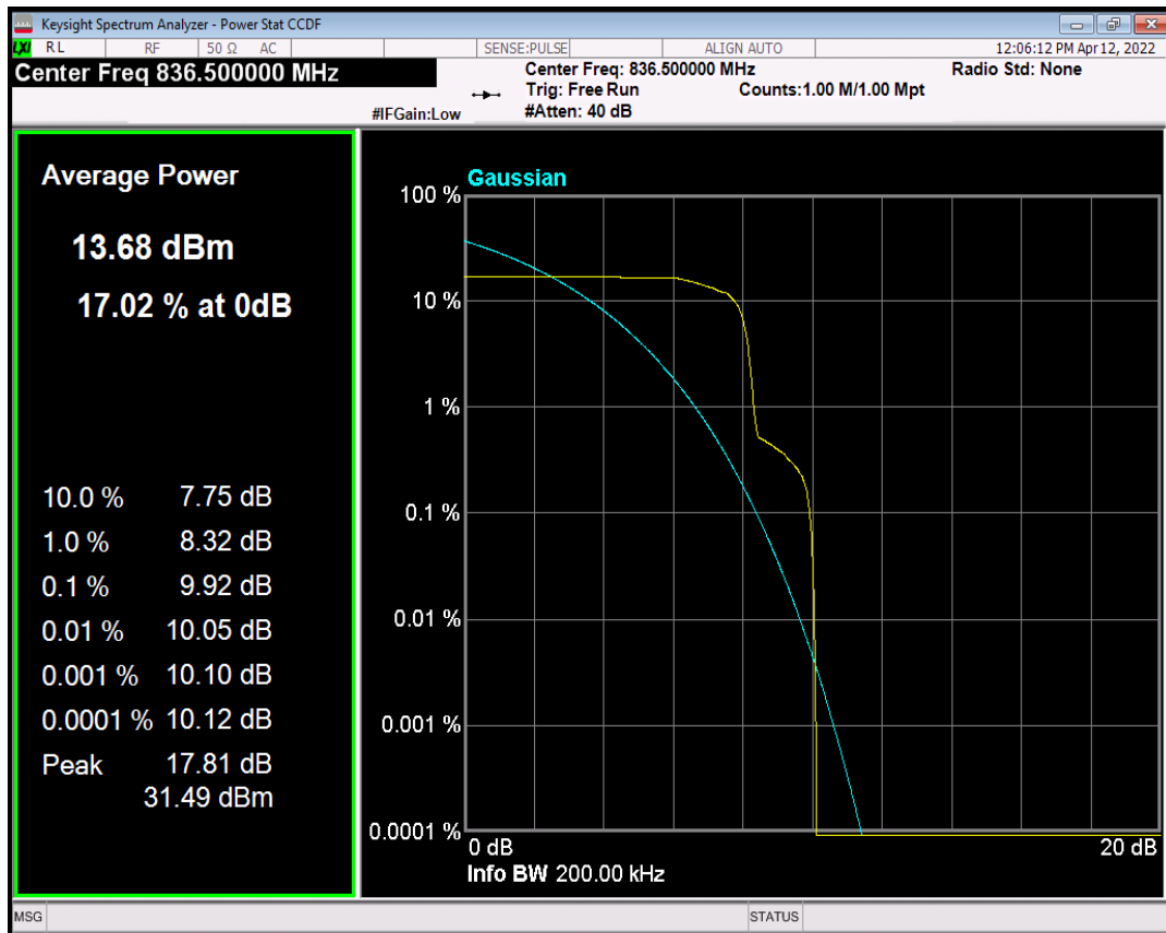
Band5 QPSK Channel=20525 nTones=1@0 Spacing=15kHz
