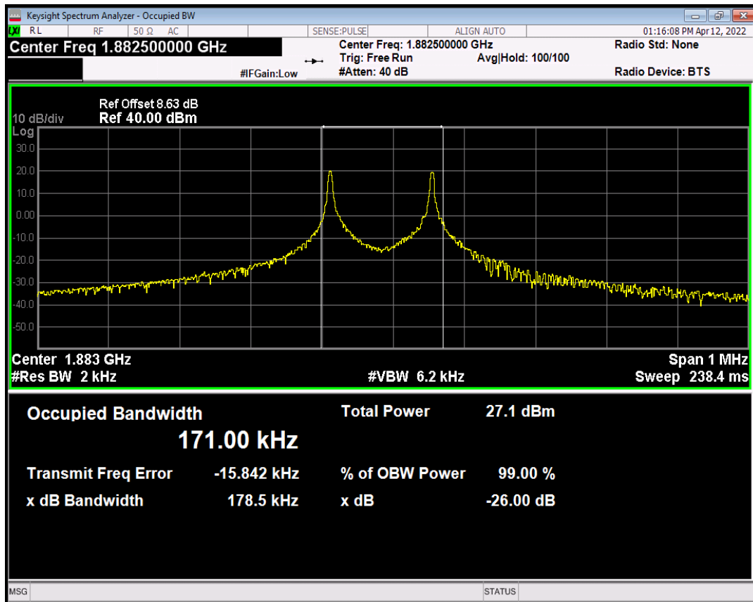
Band25 BPSK Channel=26365 nTones=1@0 Spacing=15kHz
