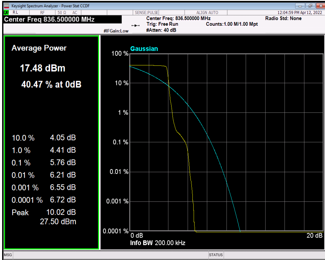
Band5 BPSK Channel=20525 nTones=1@0 Spacing=15kHz
