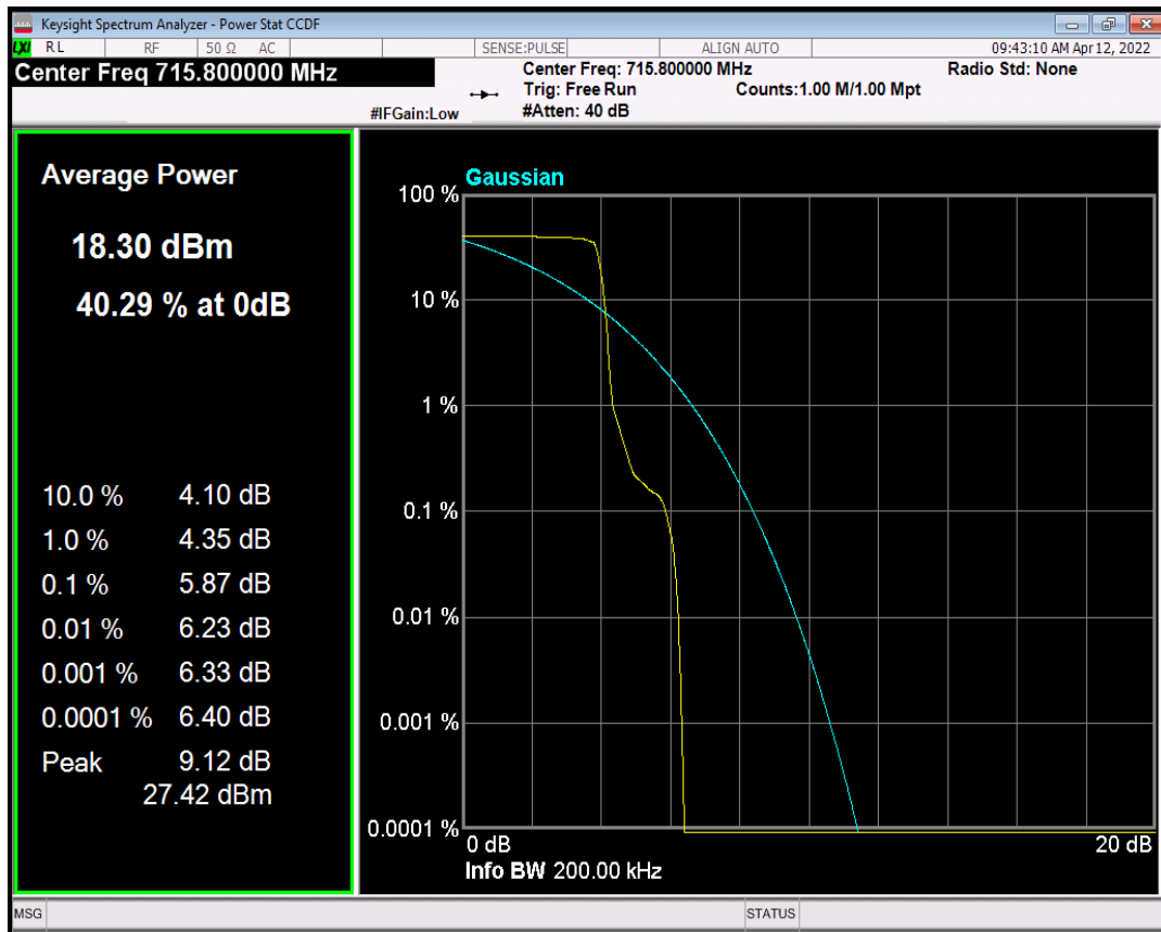
Band12 BPSK Channel=23178 nTones=1@0 Spacing=15kHz
