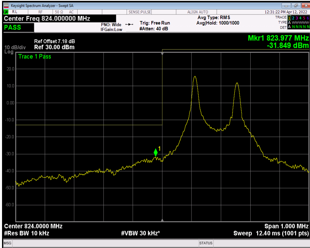
Band5 QPSK Channel=20402 nTones=1@0 Spacing=3.75kHz
