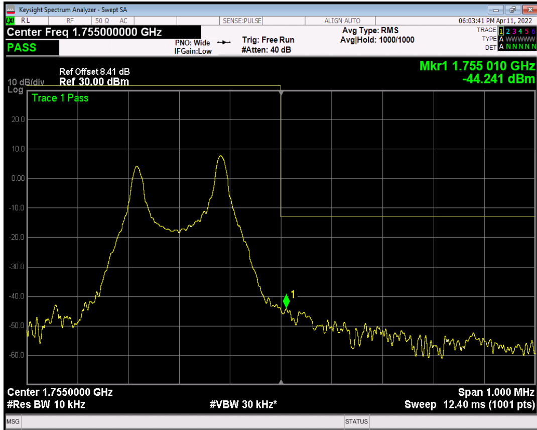
Band4 QPSK Channel=20398 nTones=12@0 Spacing=15kHz
