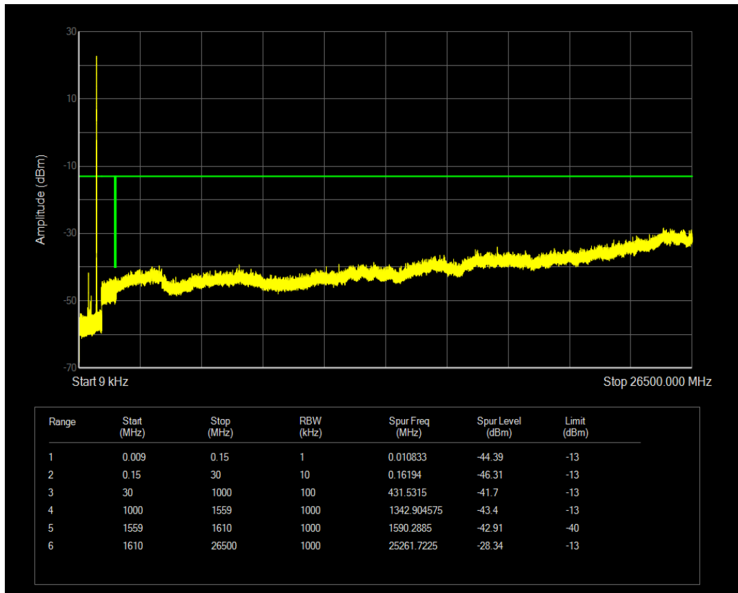
Band13 BPSK Channel=23230 nTones=1@0 Spacing=3.75kHz
