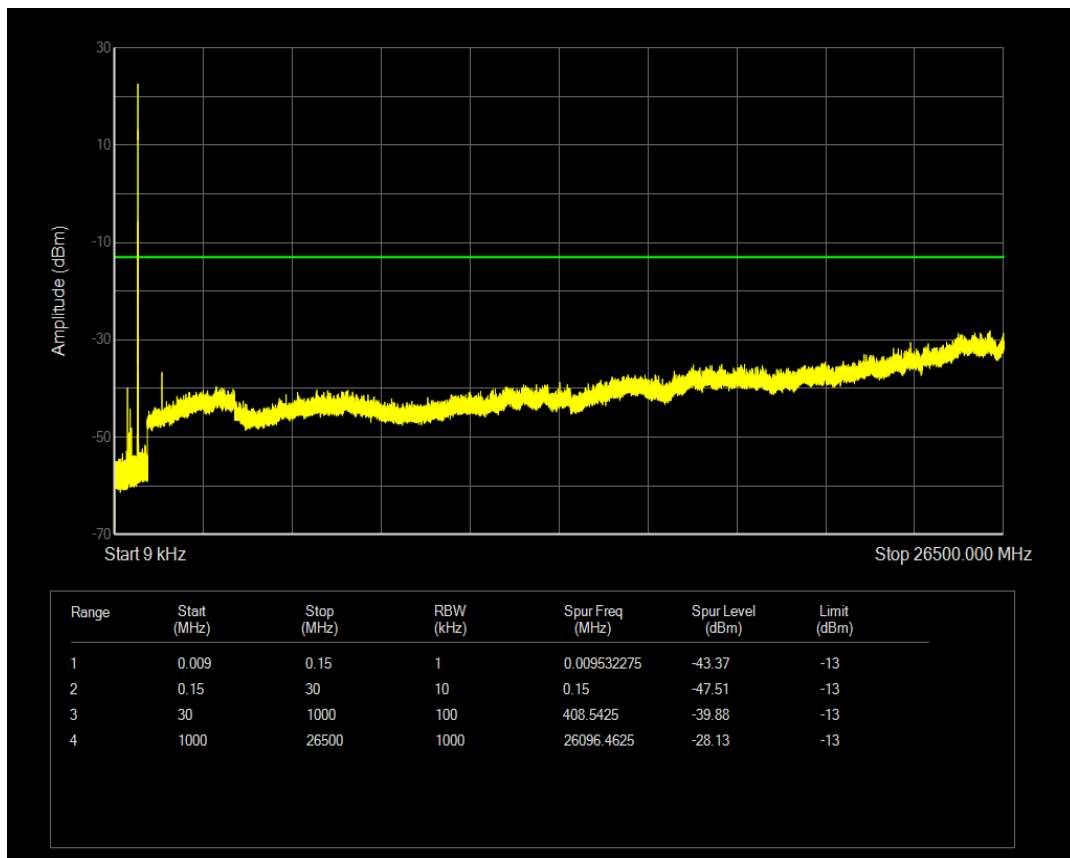
Band13 BPSK Channel=23182 nTones=1@0 Spacing=3.75kHz
