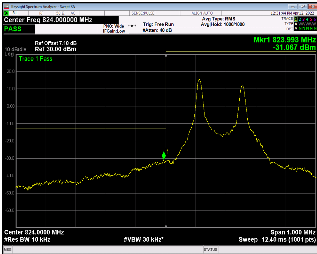
Band5 BPSK Channel=20402 nTones=1@0 Spacing=15kHz
