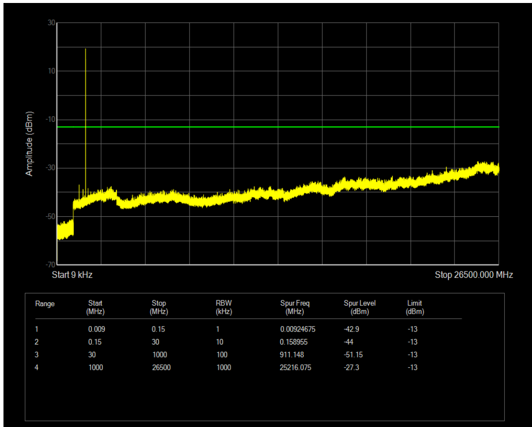
Band4 BPSK Channel=20398 nTones=1@0 Spacing=3.75kHz
