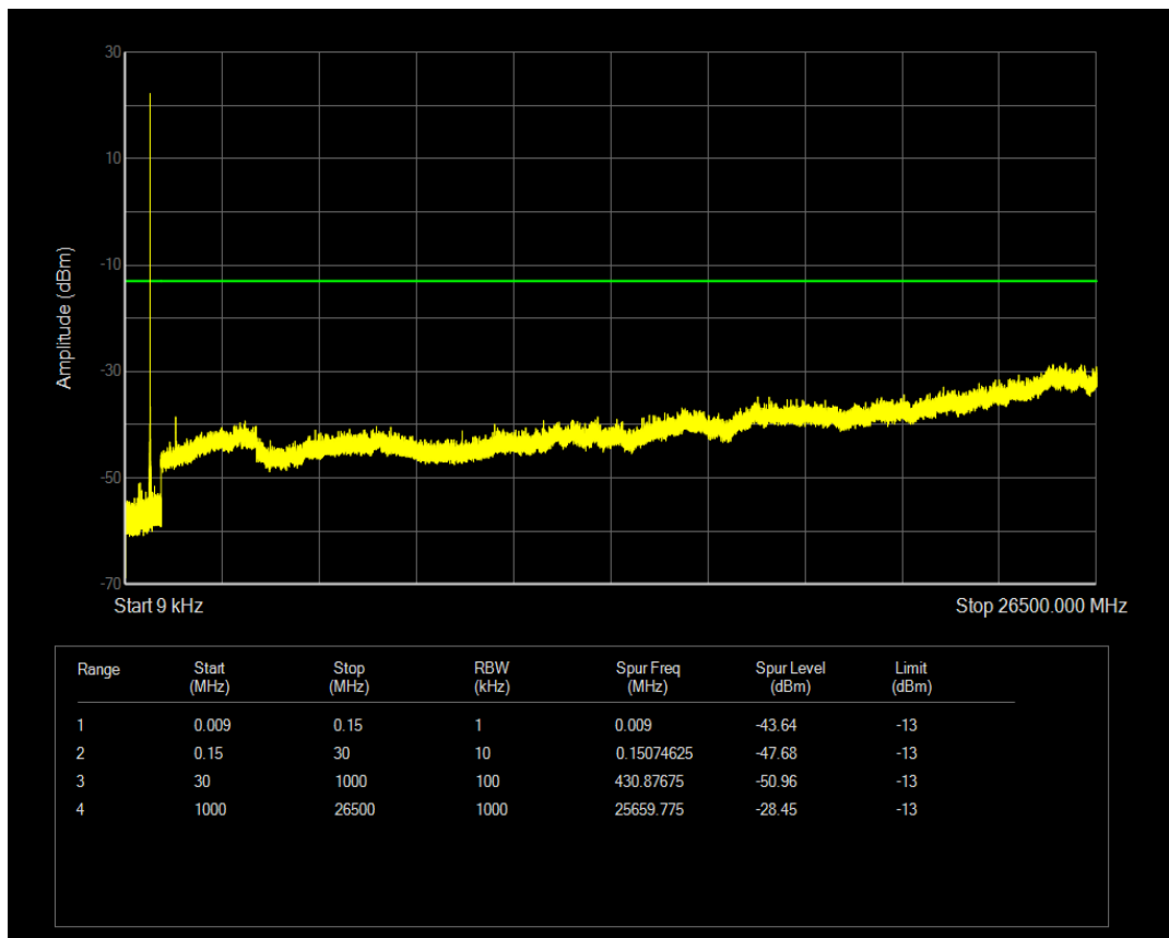
Band12 BPSK Channel=23095 nTones=1@0 Spacing=3.75kHz
