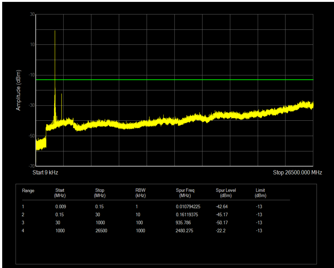
Band25 QPSK Channel=26042 nTones=1@47 Spacing=3.75kHz
