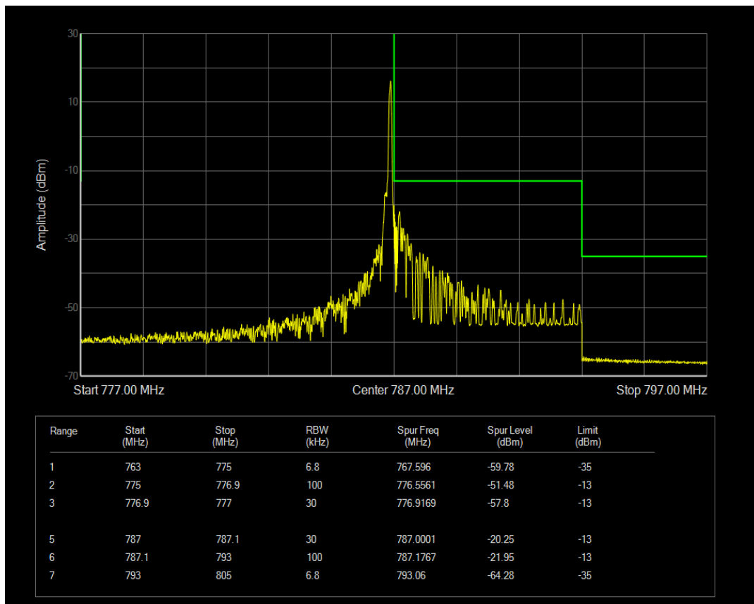
Band13 BPSK Channel=23278 nTones=1@11 Spacing=15kHz
