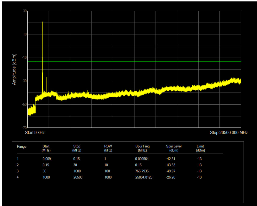
Band2 QPSK Channel=18900 nTones=1@47 Spacing=3.75kHz
