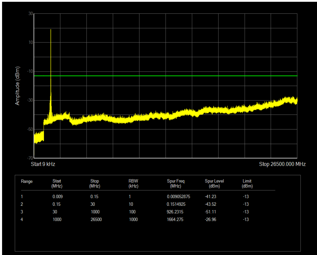
Band4 QPSK Channel=19952 nTones=1@0 Spacing=15kHz
