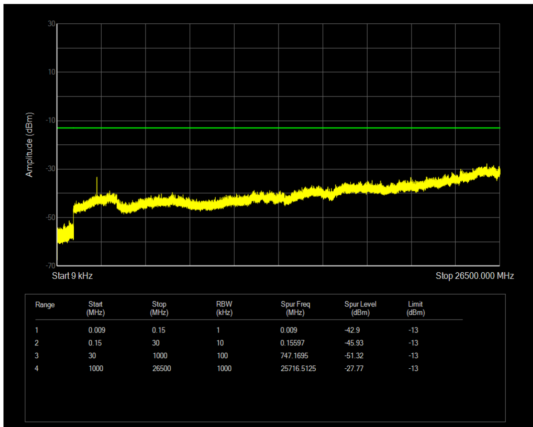
Band5 BPSK Channel=20648 nTones=1@0 Spacing=3.75kHz
