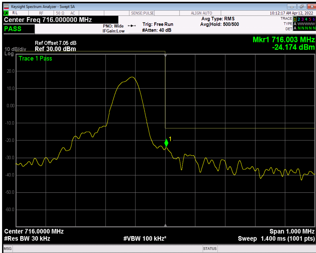
Band12 BPSK Channel=23178 nTones=1@11 Spacing=15kHz
