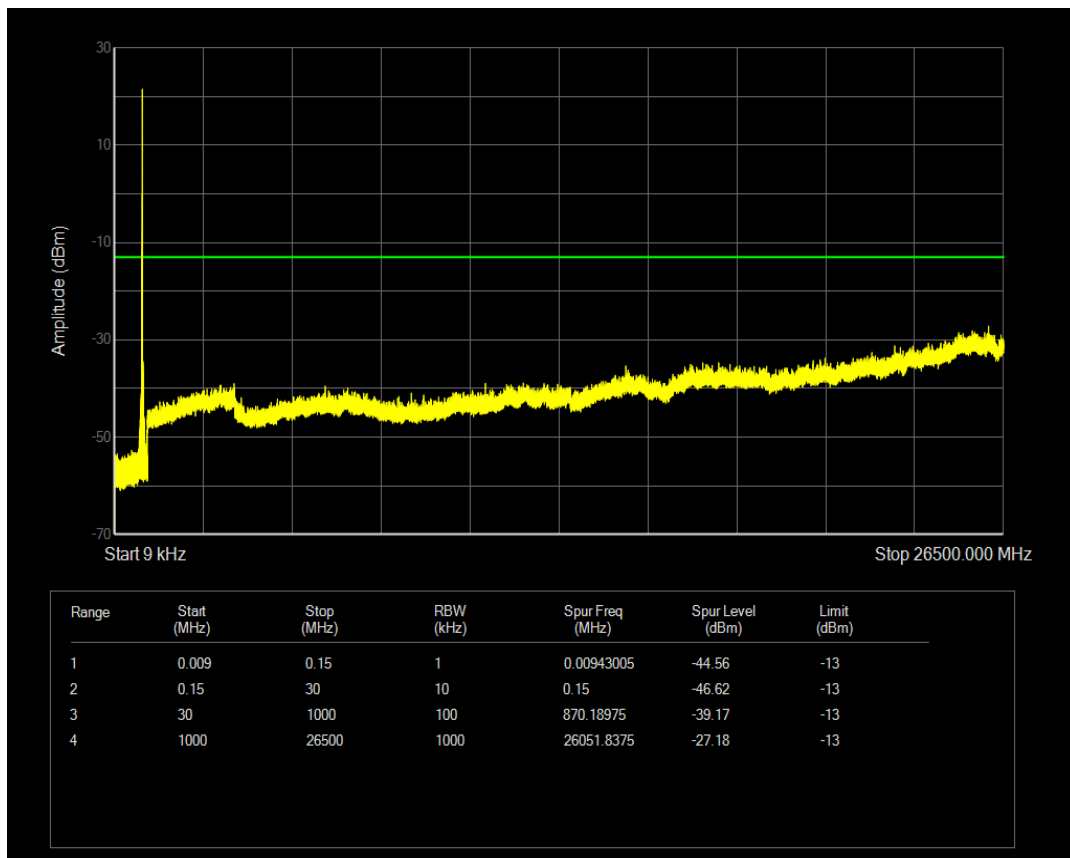
Band5 QPSK Channel=20648 nTones=1@0 Spacing=15kHz
