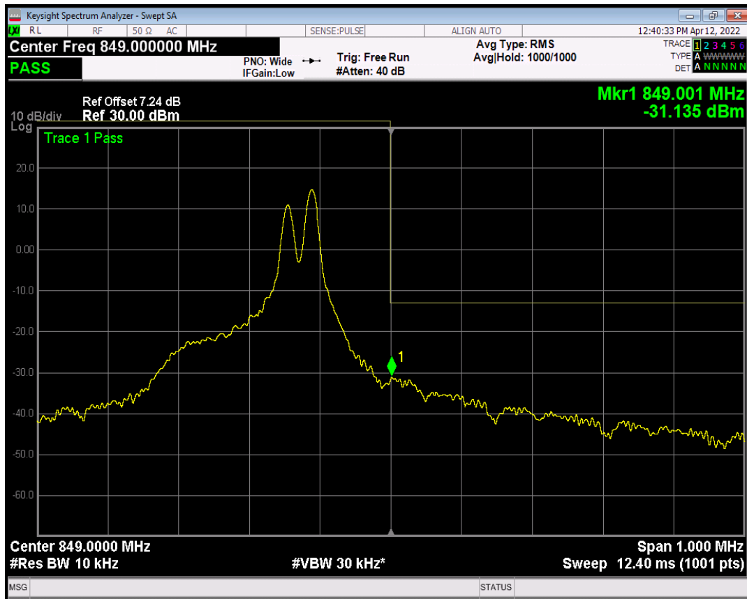
Band5 BPSK Channel=20648 nTones=1@11 Spacing=15kHz
