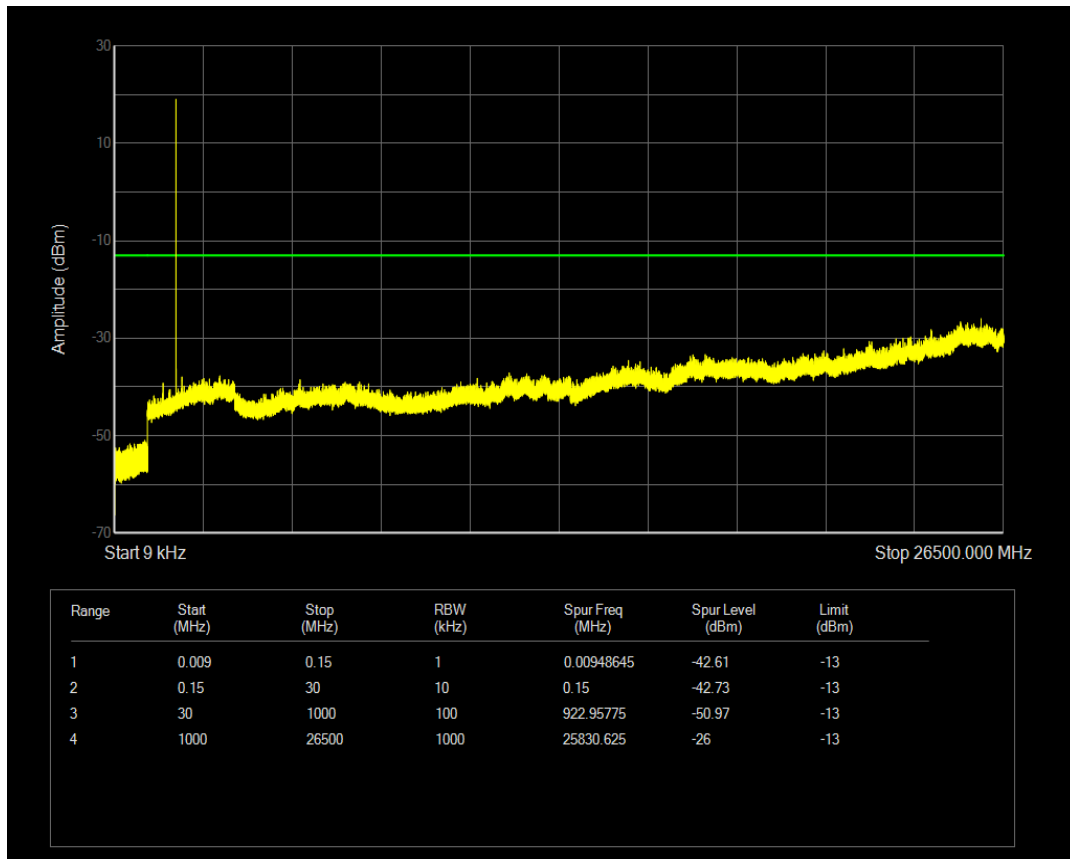
Band25 BPSK Channel=26365 nTones=1@0 Spacing=3.75kHz
