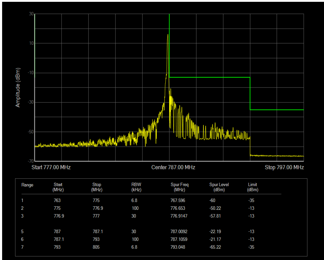
Band13 QPSK Channel=23278 nTones=1@47 Spacing=3.75kHz
