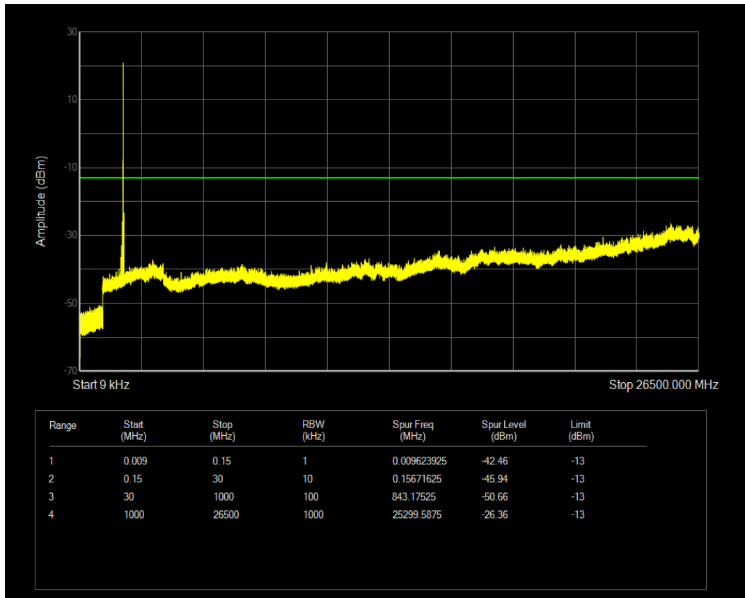
Band2 BPSK Channel=19198 nTones=1@0 Spacing=3.75kHz
