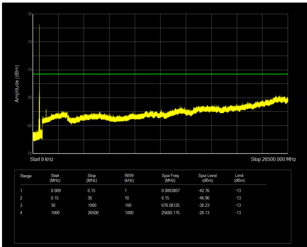
Band12 QPSK Channel=23012 nTones=1@47 Spacing=3.75kHz
