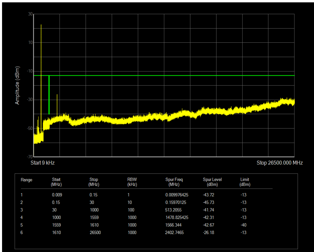
Band13 BPSK Channel=23278 nTones=1@0 Spacing=3.75kHz
