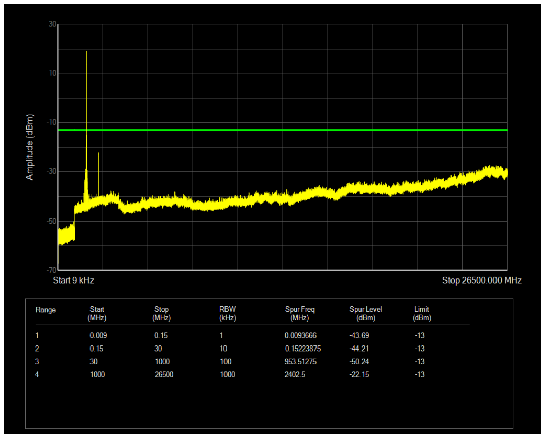
Band4 QPSK Channel=19952 nTones=1@47 Spacing=3.75kHz
