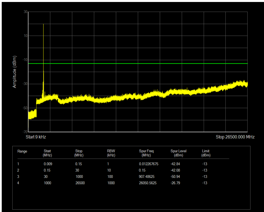
Band2 QPSK Channel=18602 nTones=1@47 Spacing=3.75kHz
