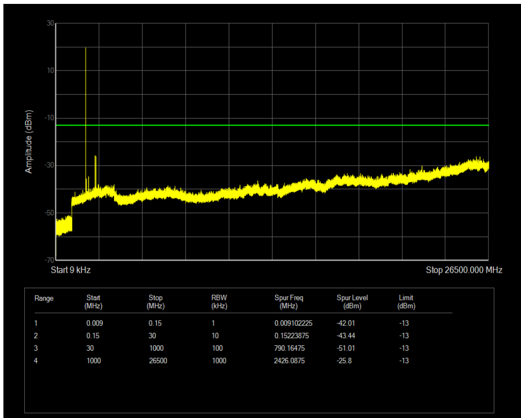
Band2 BPSK Channel=18900 nTones=1@0 Spacing=3.75kHz
