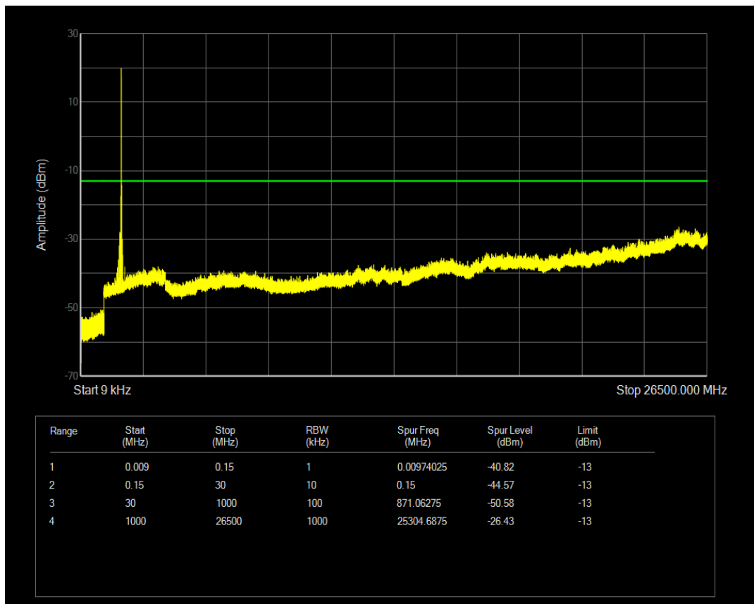
Band4 QPSK Channel=20175 nTones=1@0 Spacing=15kHz
