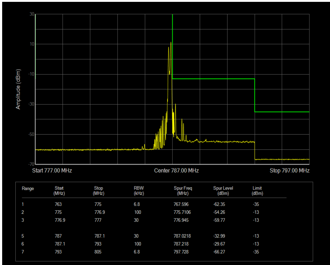
Band13 QPSK Channel=23278 nTones=1@11 Spacing=15kHz
