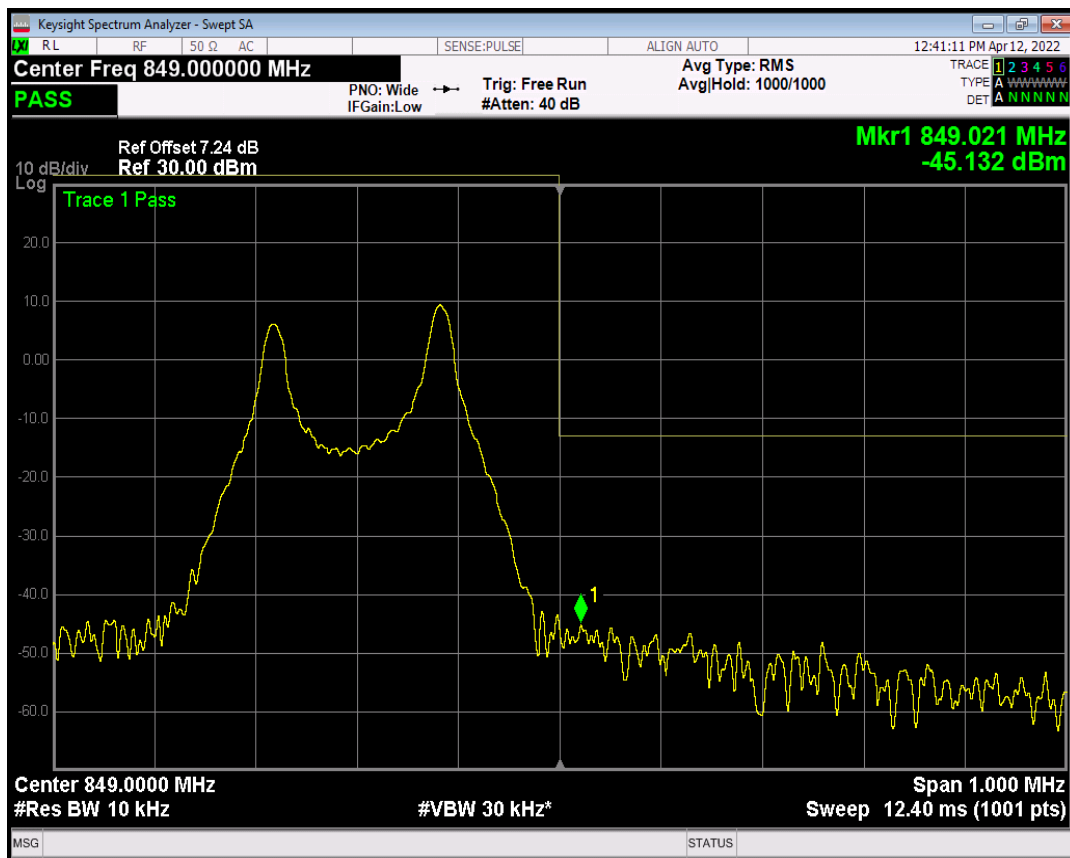
Band5 QPSK Channel=20648 nTones=1@11 Spacing=15kHz
