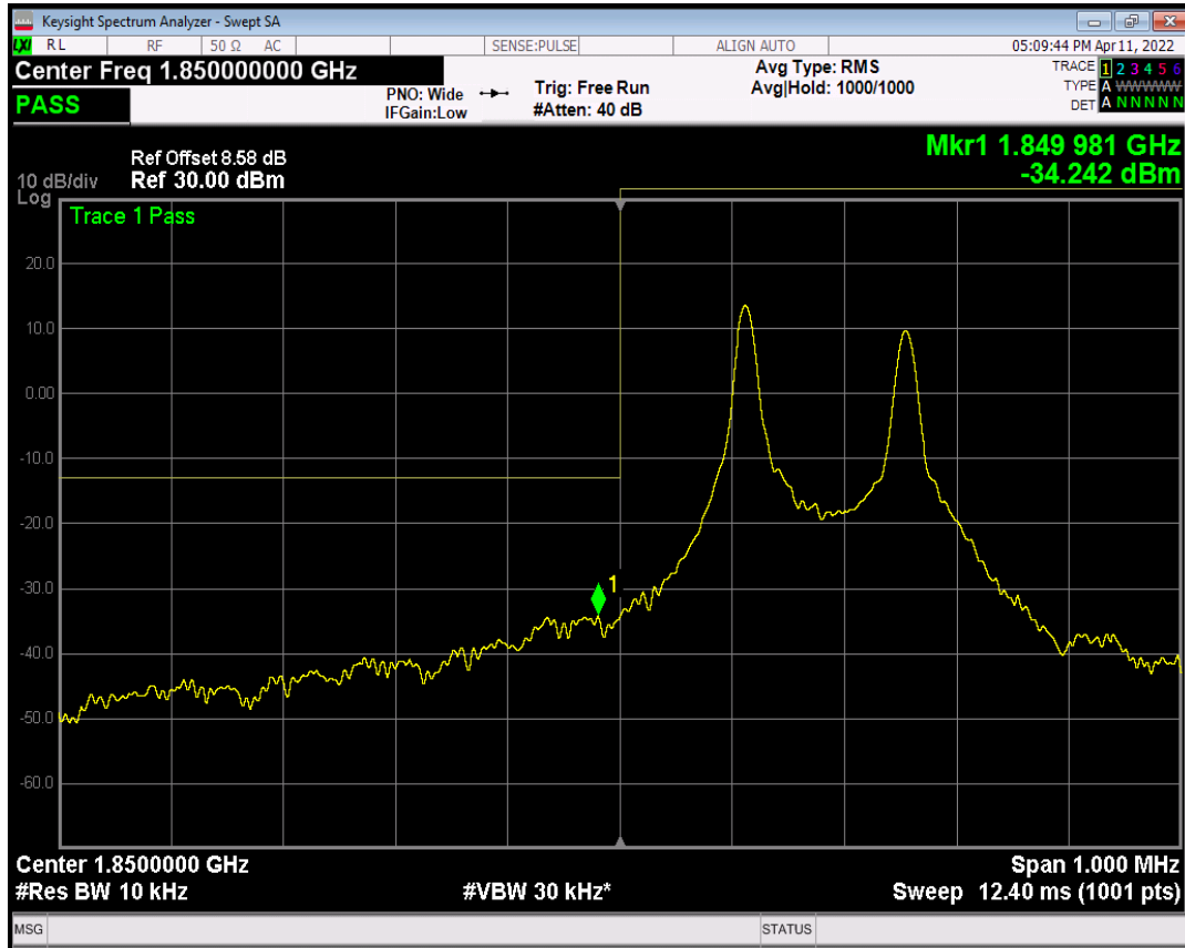
Band2 BPSK Channel=18602 nTones=1@0 Spacing=15kHz
