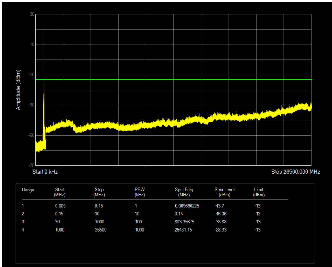
Band5 QPSK Channel=20402 nTones=1@47 Spacing=3.75kHz
