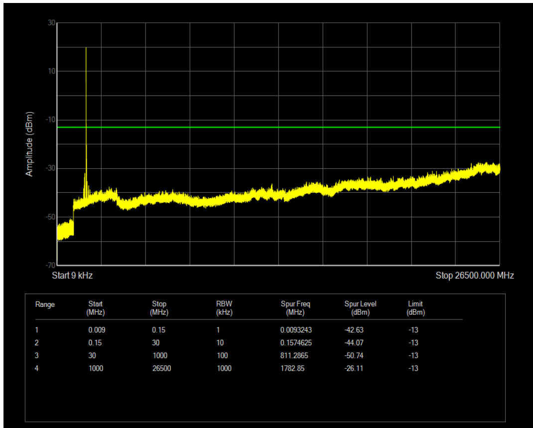
Band4 QPSK Channel=20398 nTones=1@0 Spacing=15kHz
