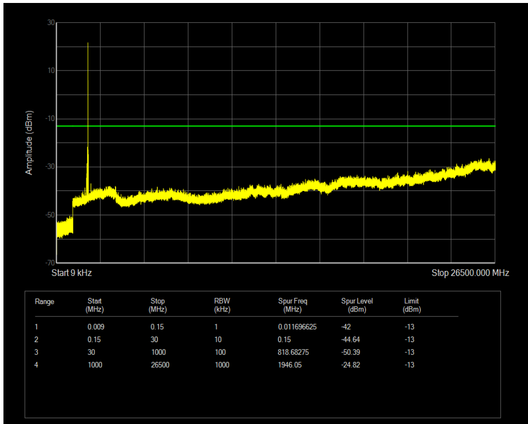
Band25 QPSK Channel=26688 nTones=1@47 Spacing=3.75kHz
