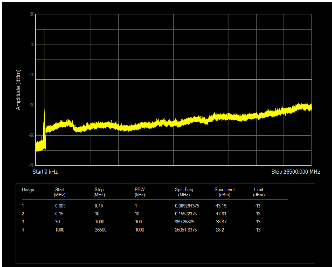
Band5 QPSK Channel=20648 nTones=1@47 Spacing=3.75kHz
