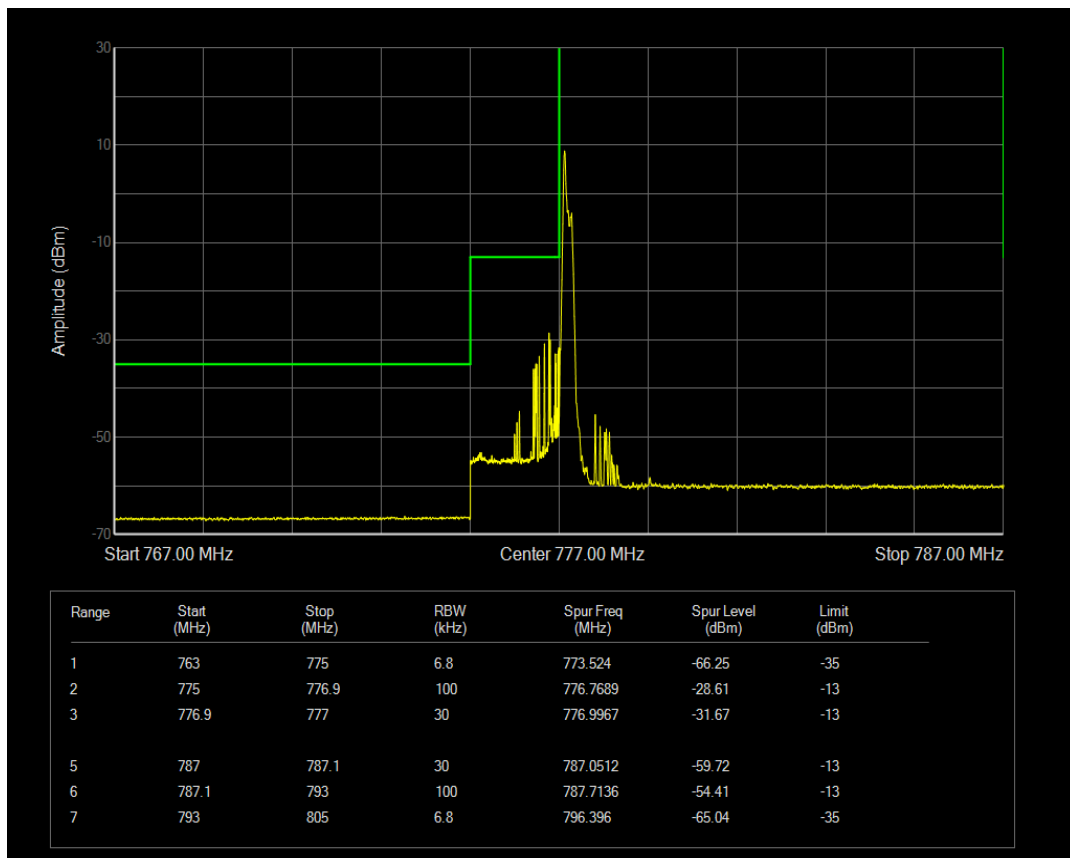
Band13 BPSK Channel=23278 nTones=1@47 Spacing=3.75kHz
