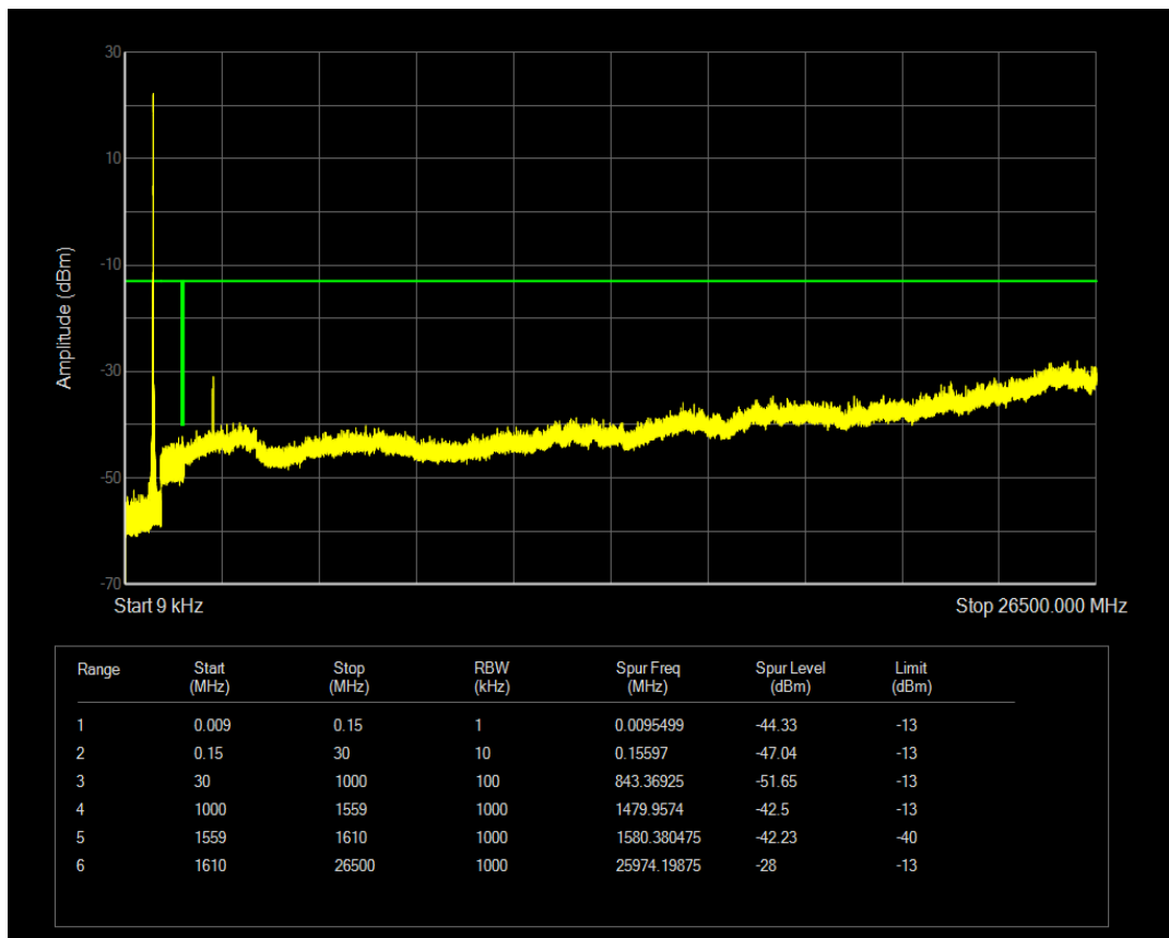
Band13 QPSK Channel=23230 nTones=1@47 Spacing=3.75kHz
