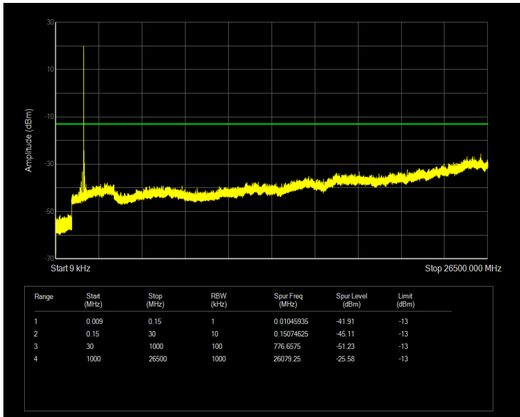
Band4 QPSK Channel=20175 nTones=1@47 Spacing=3.75kHz
