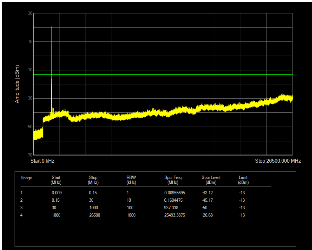
Band25 QPSK Channel=26365 nTones=1@0 Spacing=15kHz
