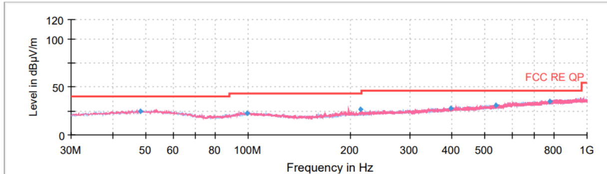
Radiated Emission from 30MHz to 1GHz
