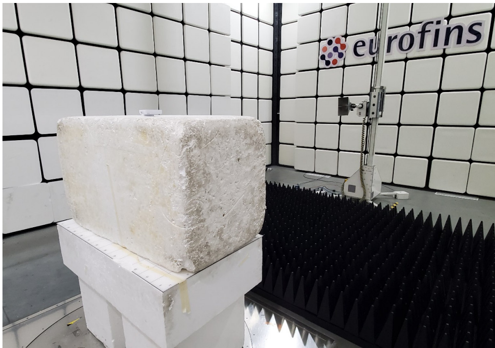
Picture 1 Radiated Emission Test Setup
