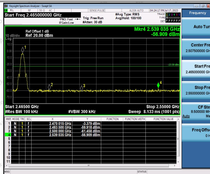
2.4G_Ant1_High_2470
