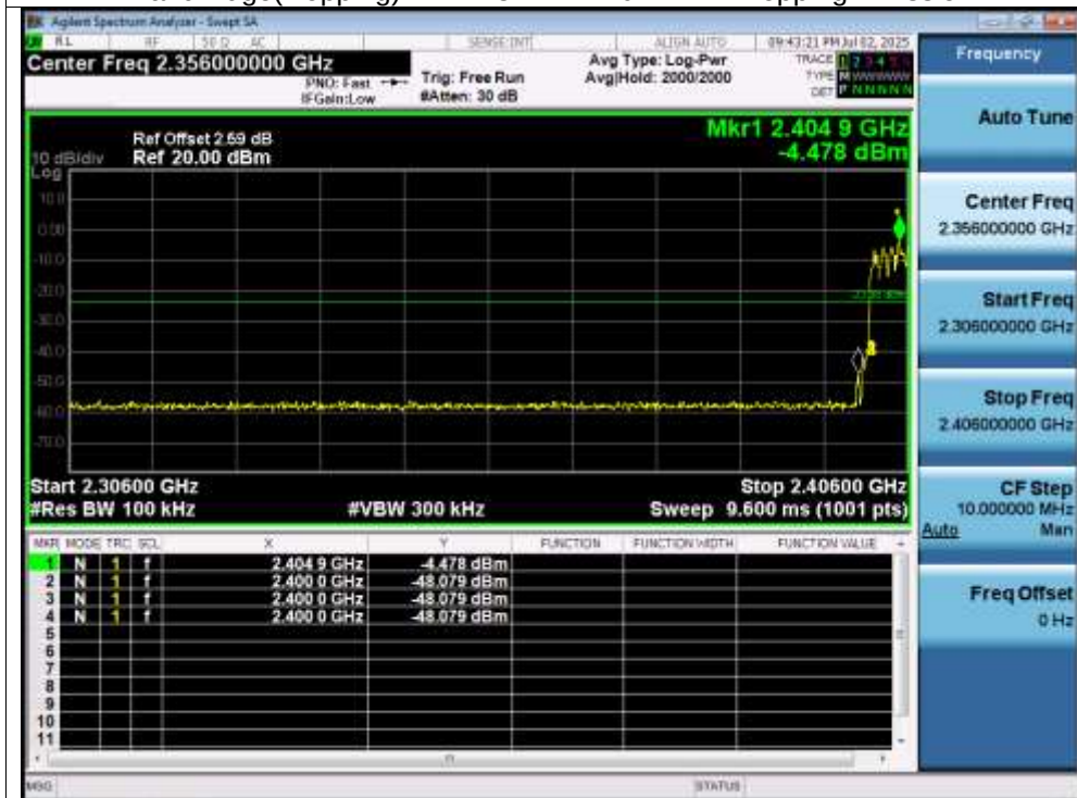
Band Edge(Hopping) NVNT 3-DH1 2402MHz Hopping Emission
