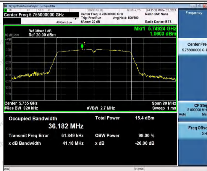
11N40SISO_WiFi 1_5755
