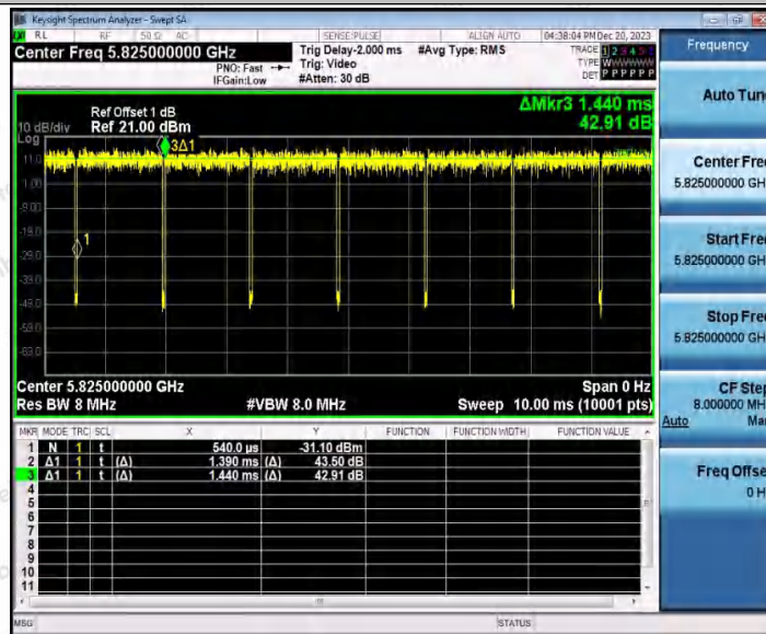
11A_WiFi 1_5825
