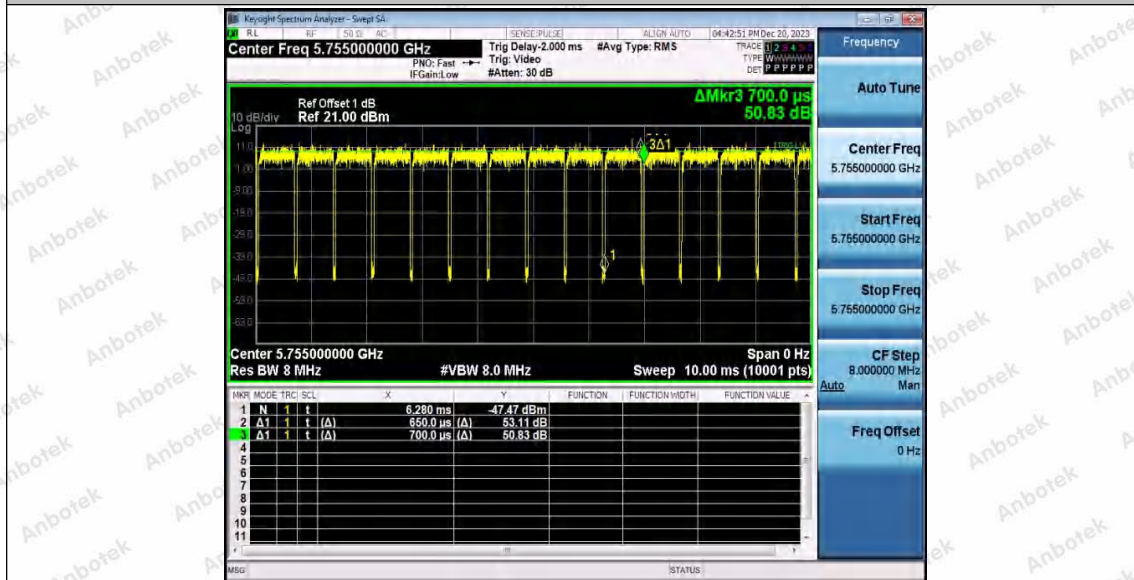
11N40SISO_WiFi 1_5755
