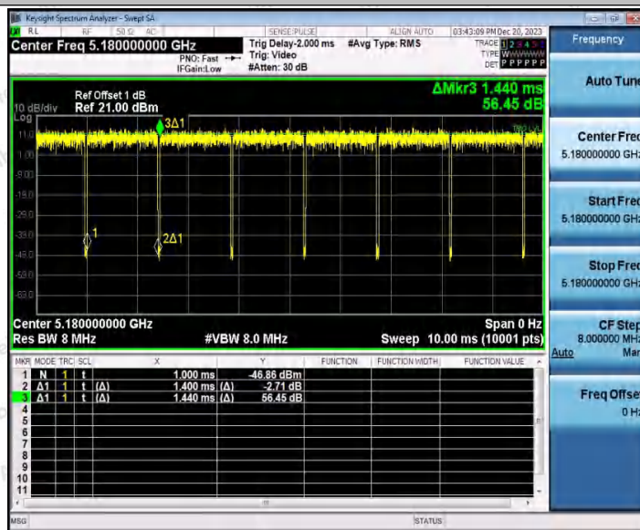
11A_WiFi 1_5180
