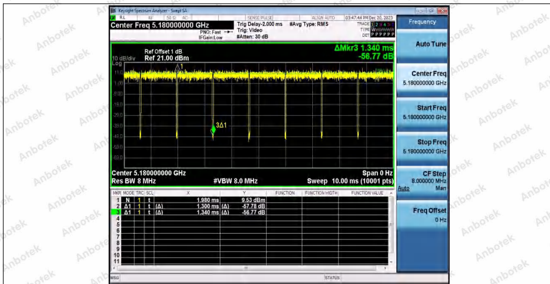
11N20SISO_WiFi 1_5180
