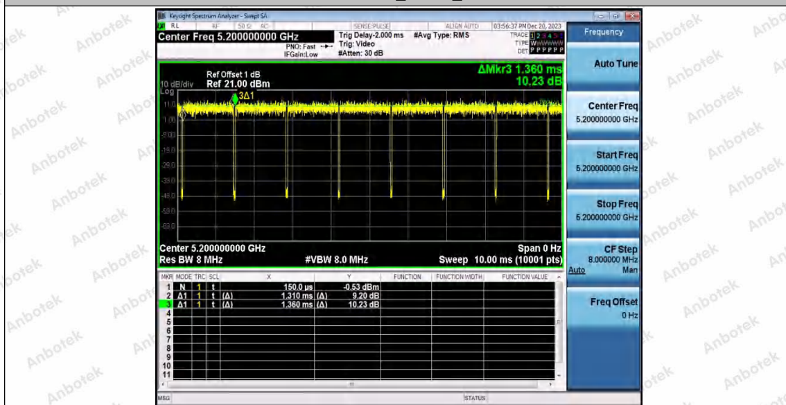
11AC20SISO_WiFi 0_5200
