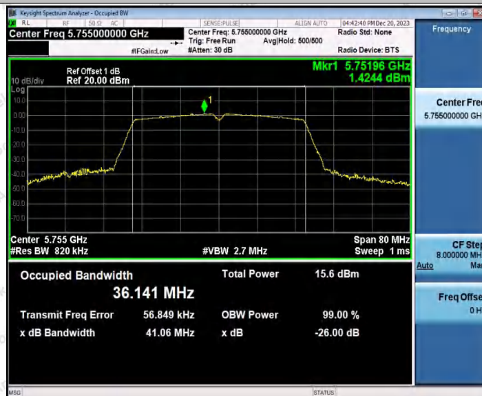
11N40SISO_WiFi 1_5755
