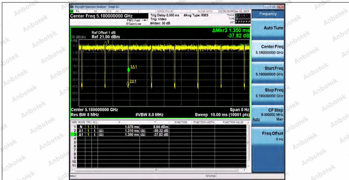
11AC20SISO_WiFi 1_5180
