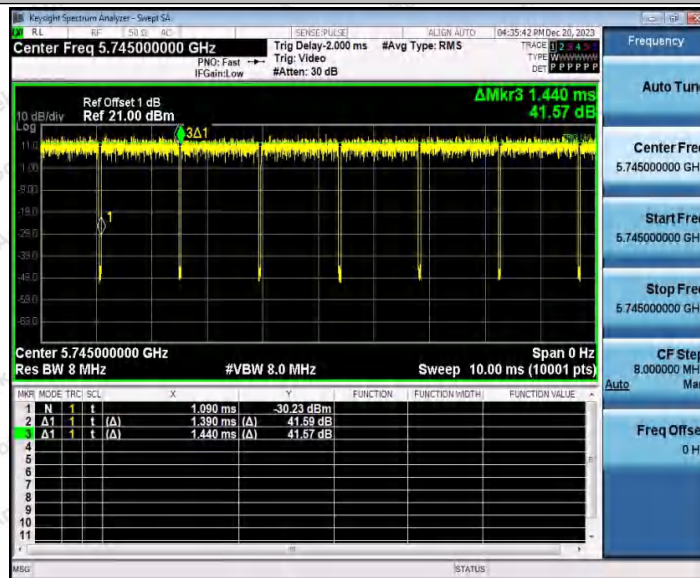
11A_WiFi 1_5745
