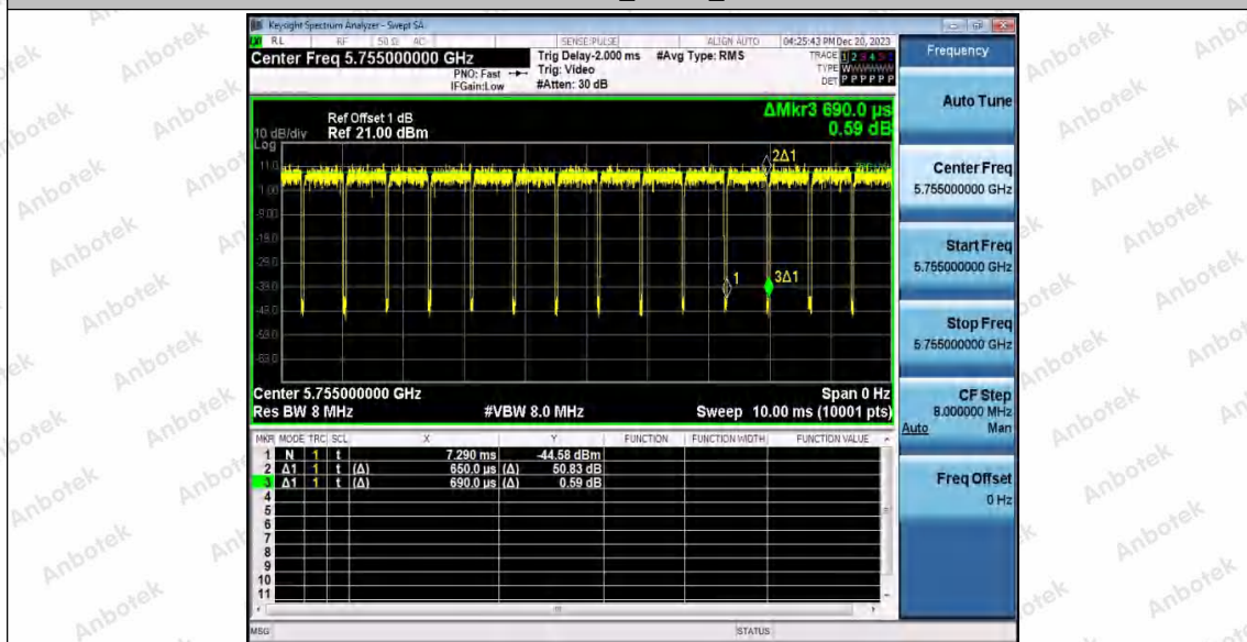
11N40SISO_WiFi 1_5755
