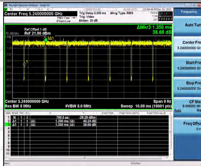
11N20SISO_WiFi 1_5240
