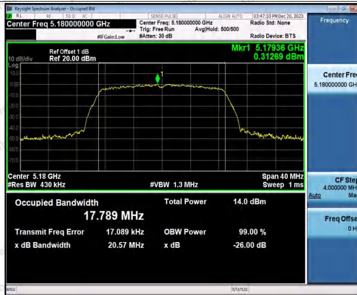
11N20SISO_WiFi 1_5180
