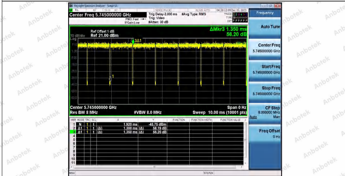
11N20SISO_WiFi 1_5745
