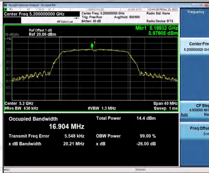
11A_WiFi 1_5200
