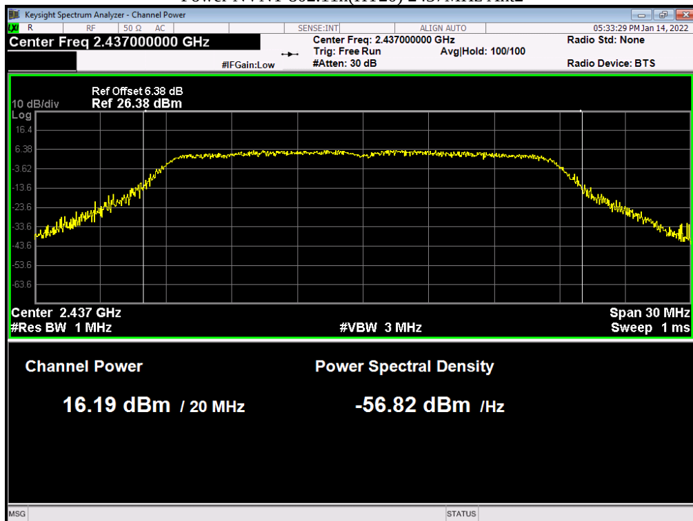
Power NVNT 802.11n(HT20) 2437MHz Ant2
