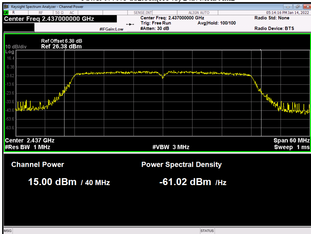
Power NVNT 802.11n(HT40) 2437MHz Ant2
