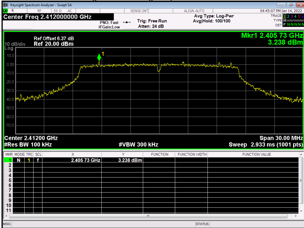
Band Edge NVNT 802.11g 6Mbps 2412MHz Ant2 Emission
