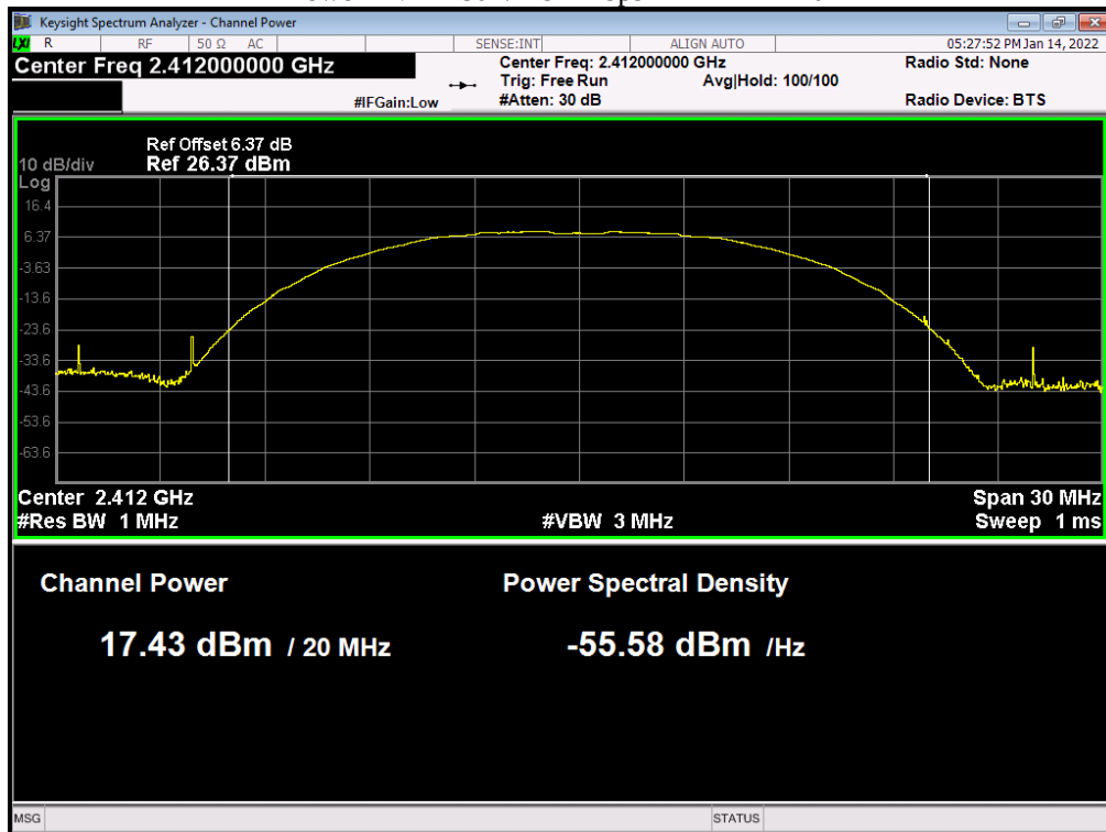
Power NVNT 802.11b 1Mbps 2412MHz Ant2
