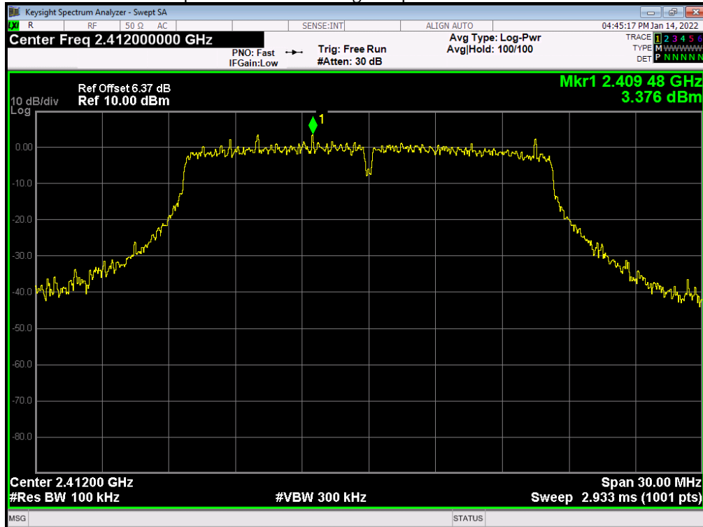
Tx. Spurious NVNT 802.11g 6Mbps 2412MHz Ant2 Emission
