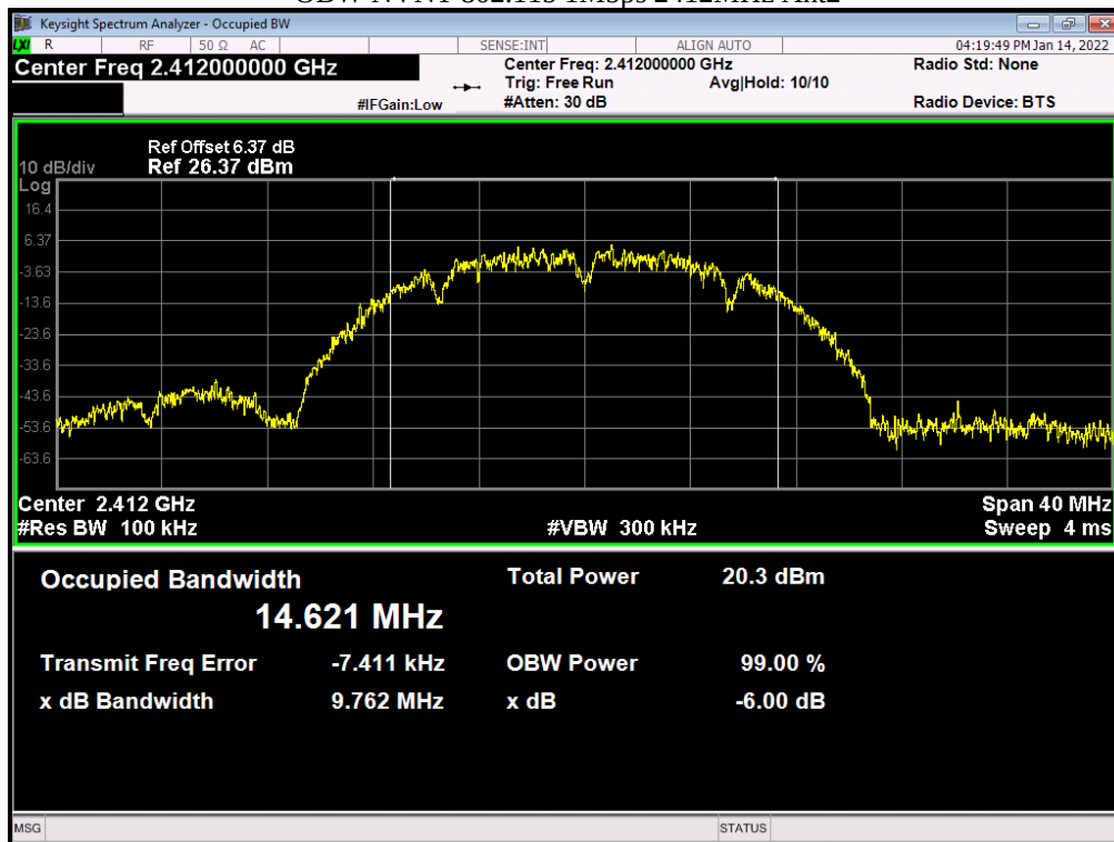
OBW NVNT 802.11b 1Mbps 2412MHz Ant2
