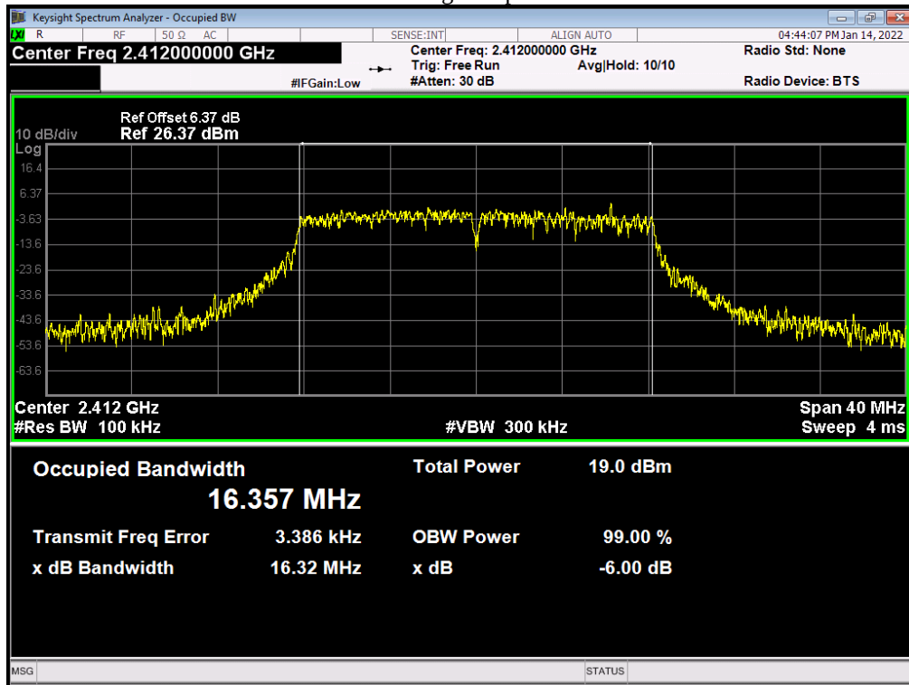
OBW NVNT 802.11g 6Mbps 2412MHz Ant2
