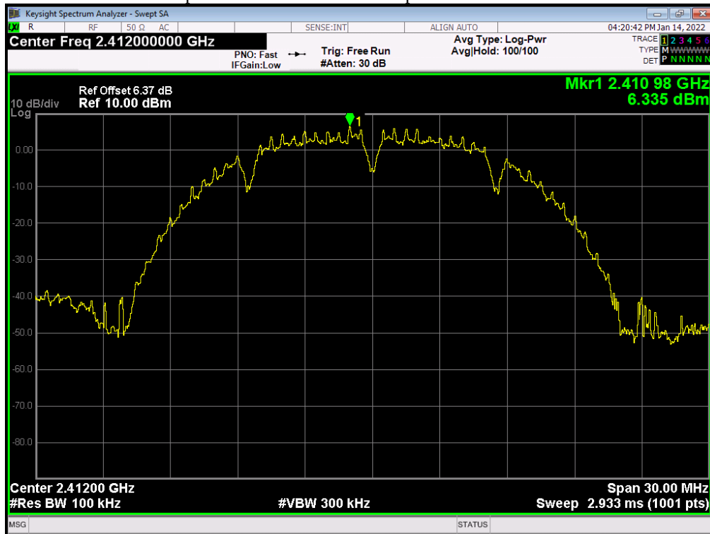
Tx. Spurious NVNT 802.11b 1Mbps 2412MHz Ant2 Ref
