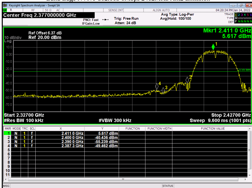
Band Edge NVNT 802.11b 1Mbps 2412MHz Ant2 Emission
