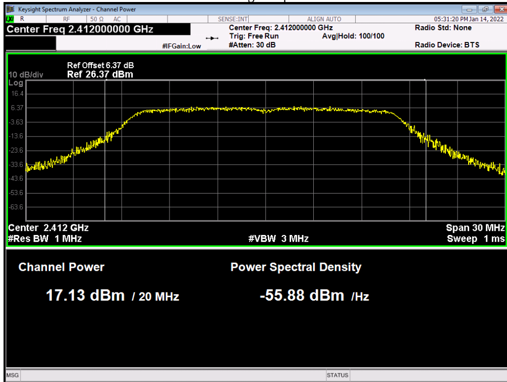
Power NVNT 802.11g 6Mbps 2412MHz Ant2
