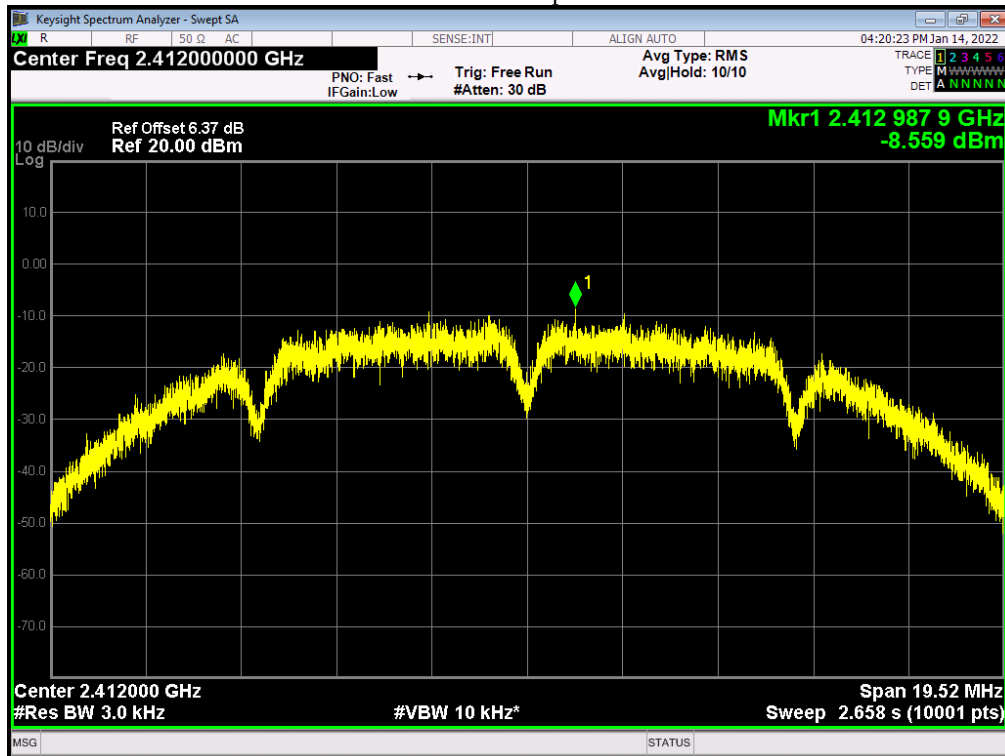
PSD NVNT 802.11b 1Mbps 2412MHz Ant2
