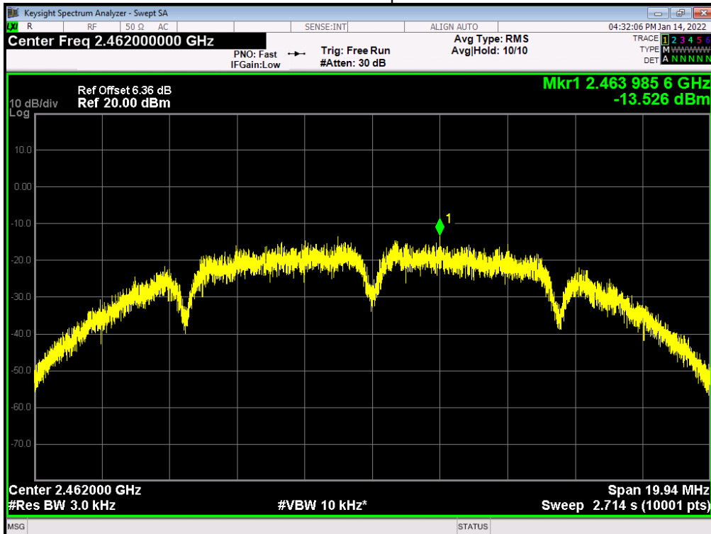
PSD NVNT 802.11b 1Mbps 2462MHz Ant2
