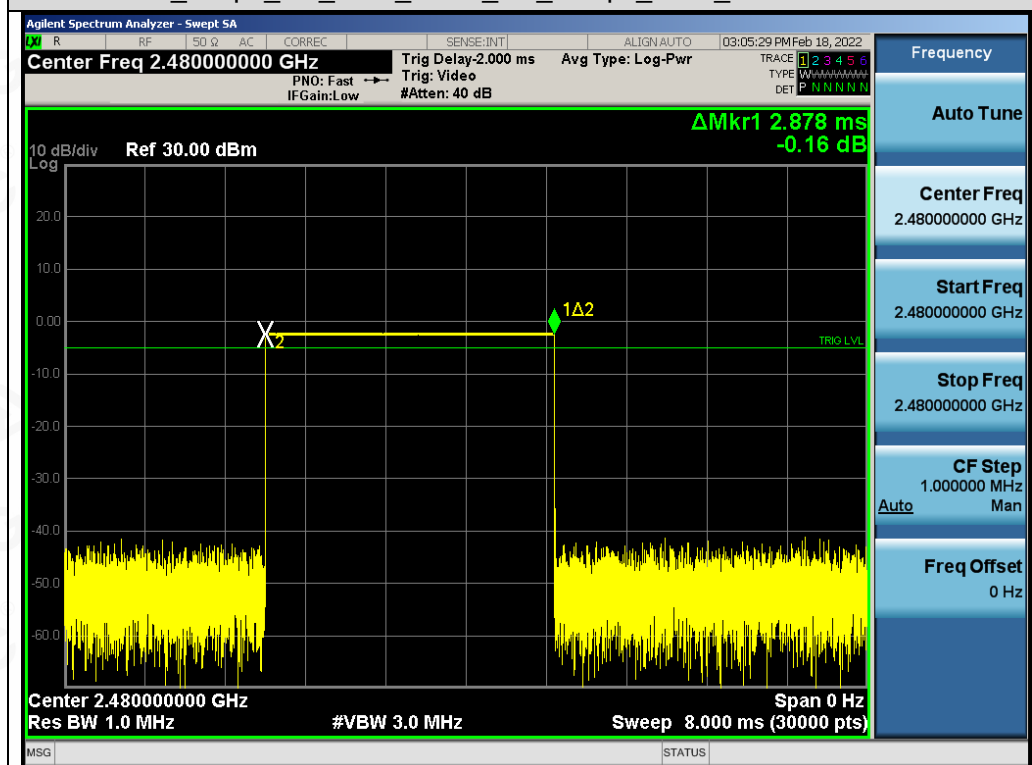
Test Graph BR HOP ANT1 NA 1Mbps 2480 Time per Burst
