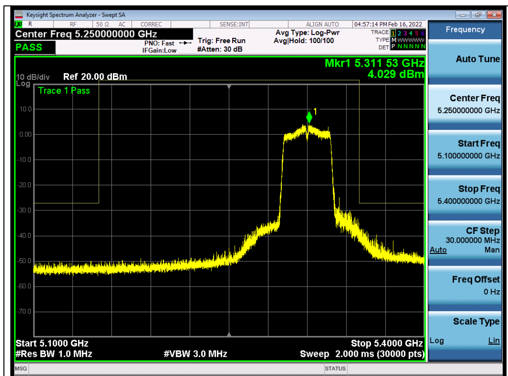
Test_Graph_802.11n40_ANT1_5310_MCS0_Frequency Band 3
