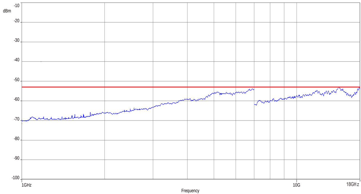
Plot No. 5: 1 GHz – 18 GHz, antenna vertical / horizontal Rx RSP-101
