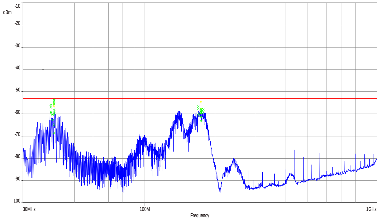
Plot No. 4: 30 MHz – 1 GHz, antenna vertical / horizontal Rx RSP-101
