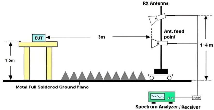
(3) In 3m Anechoic Chamber Test Setup Diagram for frequency above 1GHz
