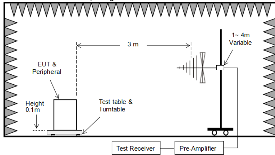
(2) In 3m Anechoic Chamber Test Setup Diagram for below 1GHz
