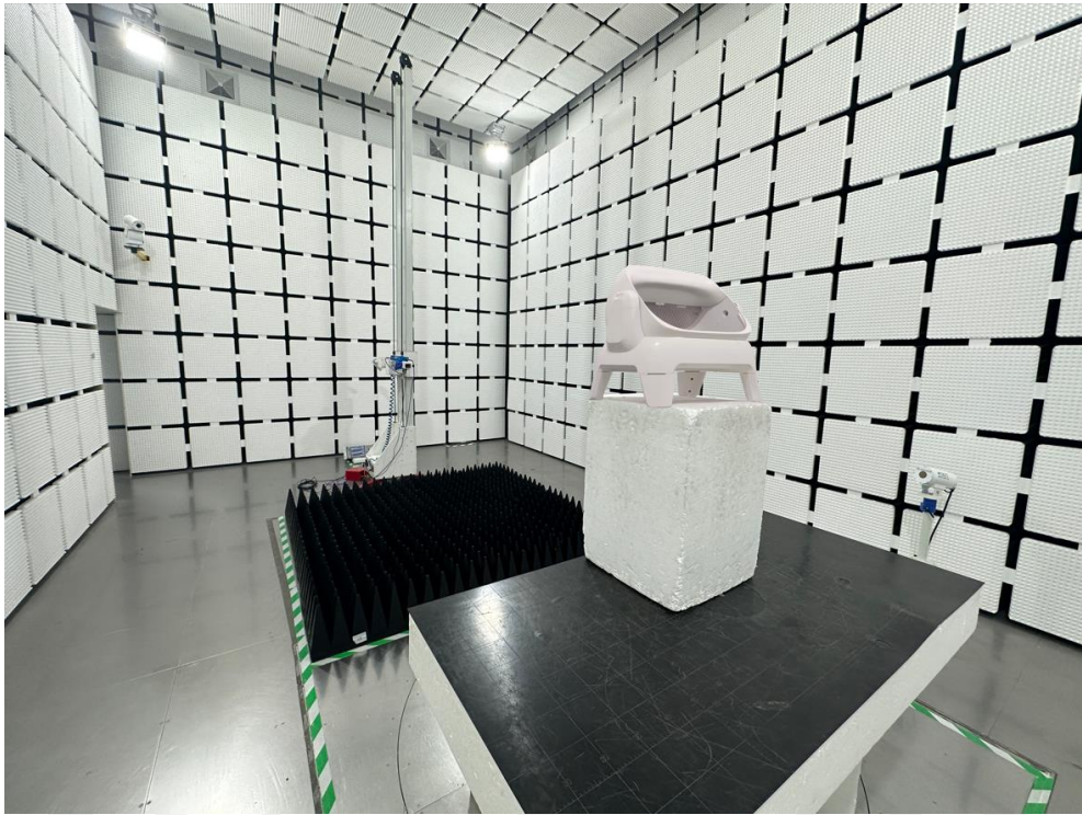
Spurious Radiation Emissions Test (> 18G)
