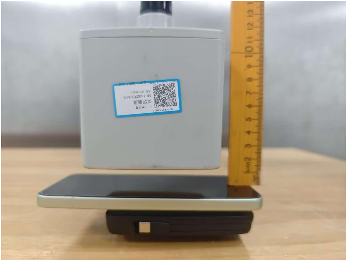
Portable exposure conditions Test Position A (6cm)
