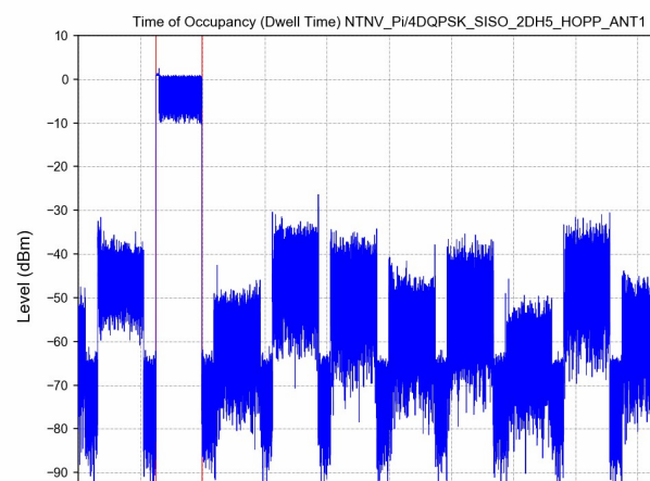
2DH5
