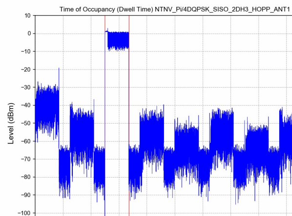
2DH3
