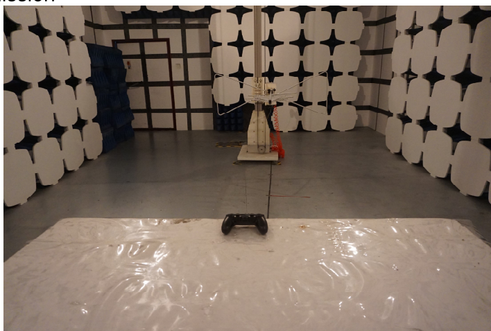
Radiated Emission
