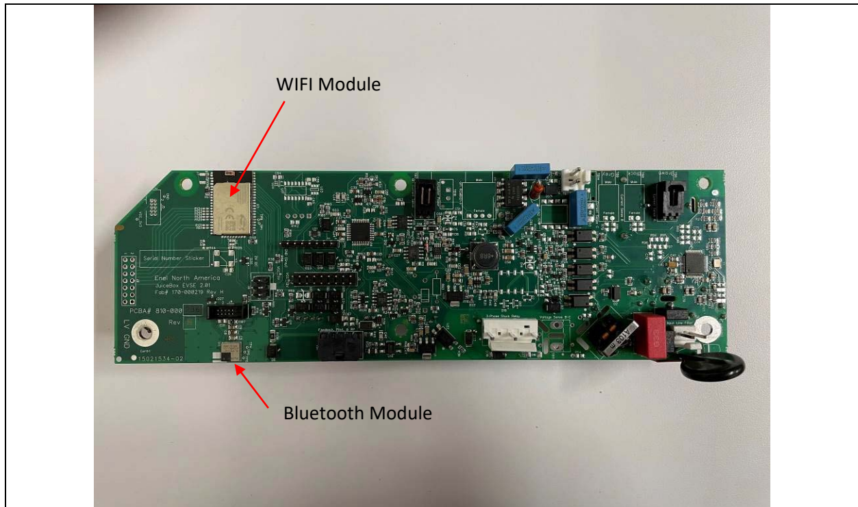
PCB 2 with WLAN module and Bluetooth module Top View
