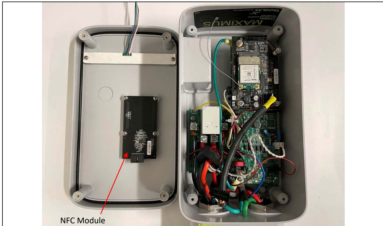
EUT Open The Enclose View
