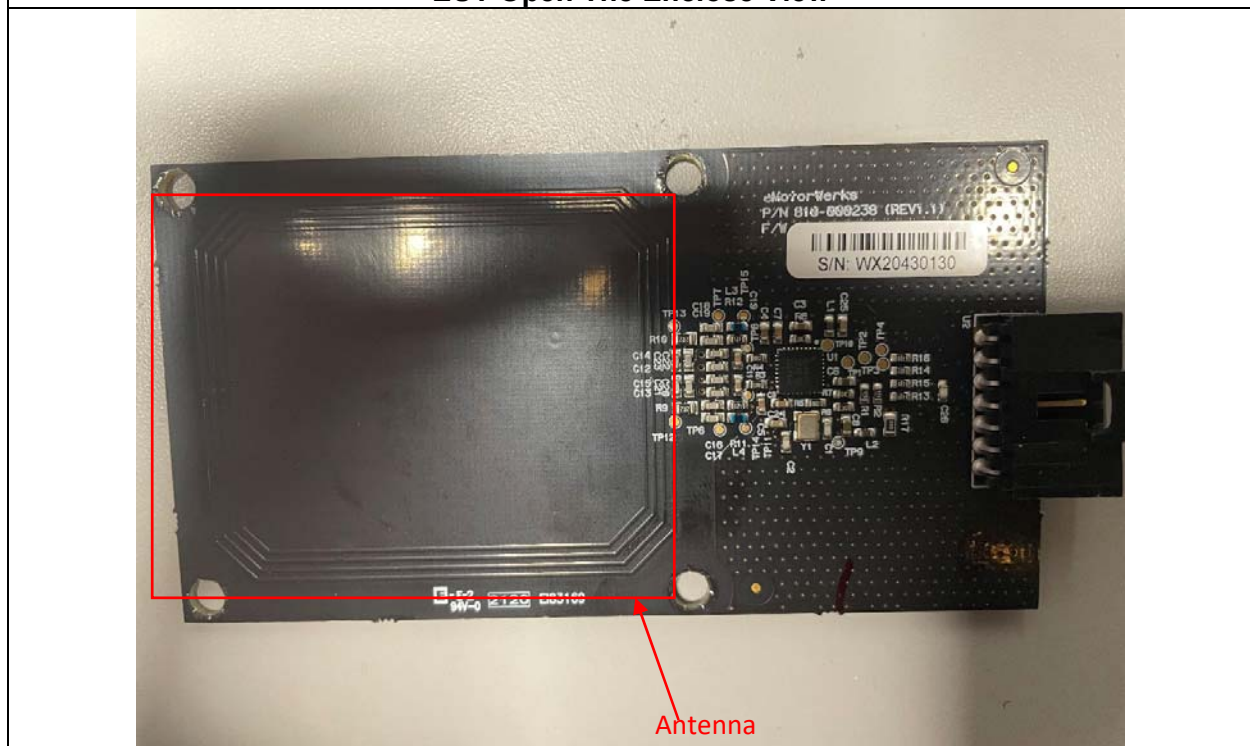
NFC main board with antenna Top View
