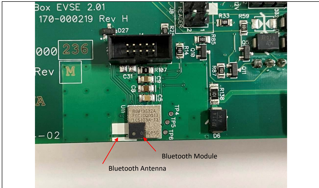
Bluetooth module and Antenna
