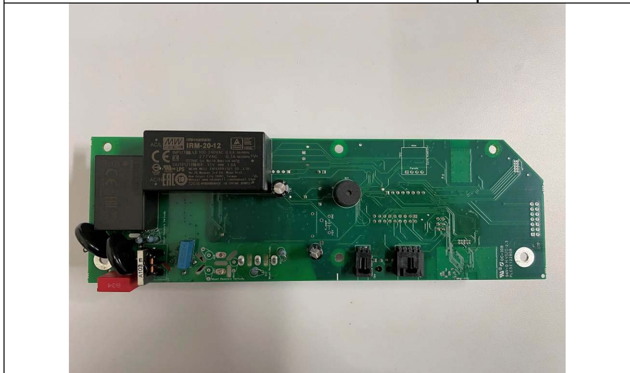
PCB 2 with WLAN module and Bluetooth module Bottom View
