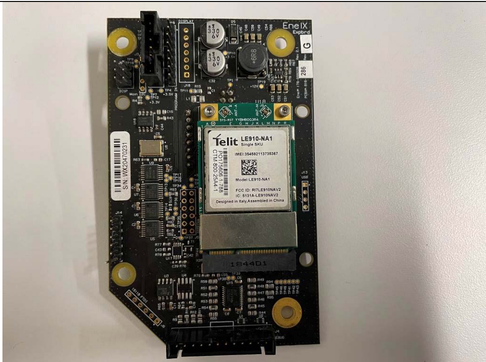
PCB 1 with cellular module Top View
