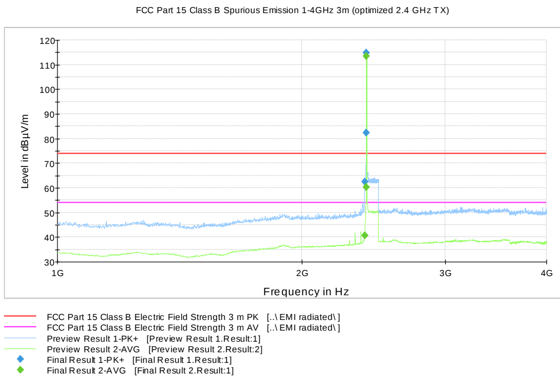
Figure 27: Channel 0 low 1 GHz – 4 GHz (N)
