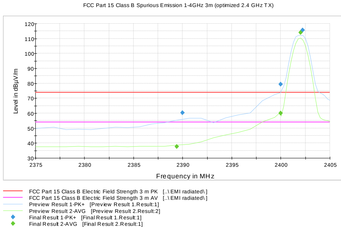
Figure 38: Radiated Band Edge measurement graph, Channel 0 low (N)
