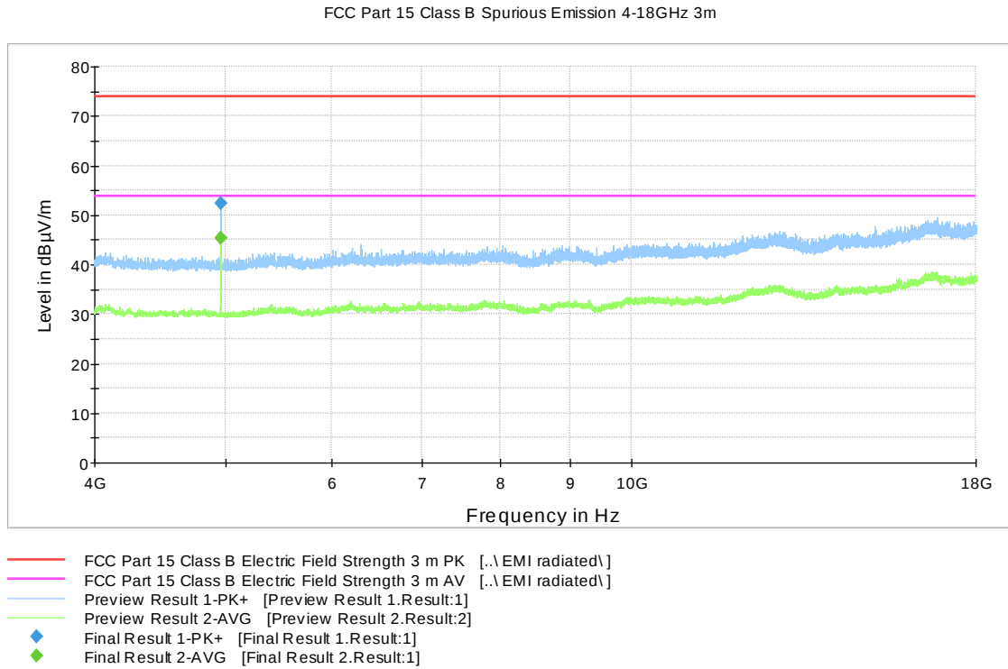
Figure 36: Channel 39 high 4 GHz – 18 GHz (N)
