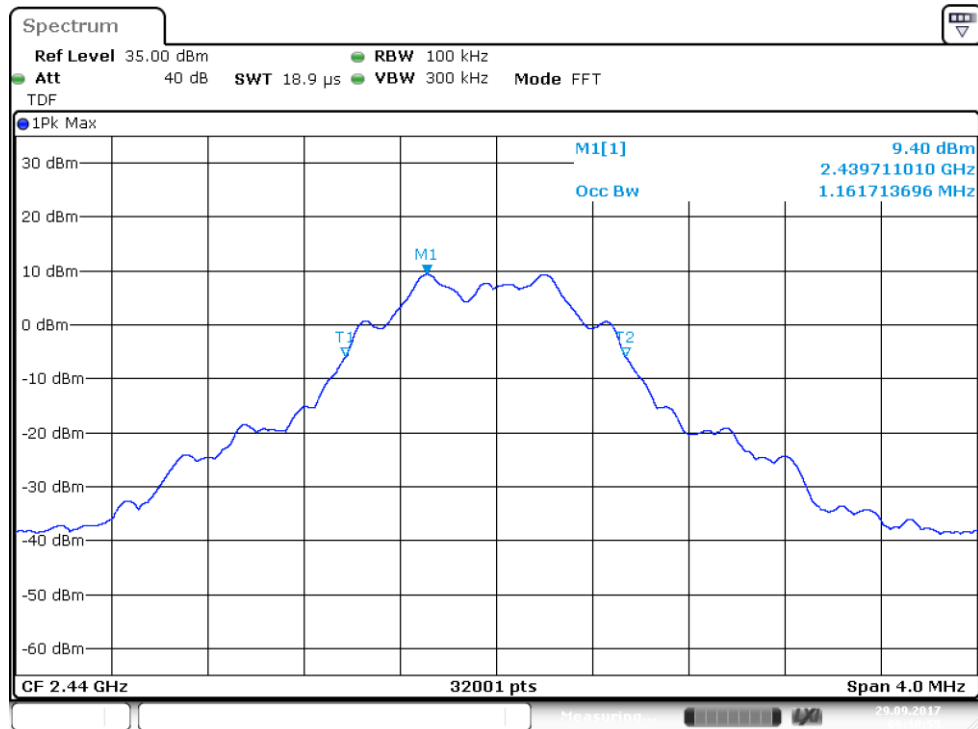
Figure 57: 99% OBW, Channel 19 mid, power setting 145, PHY 125k coded
