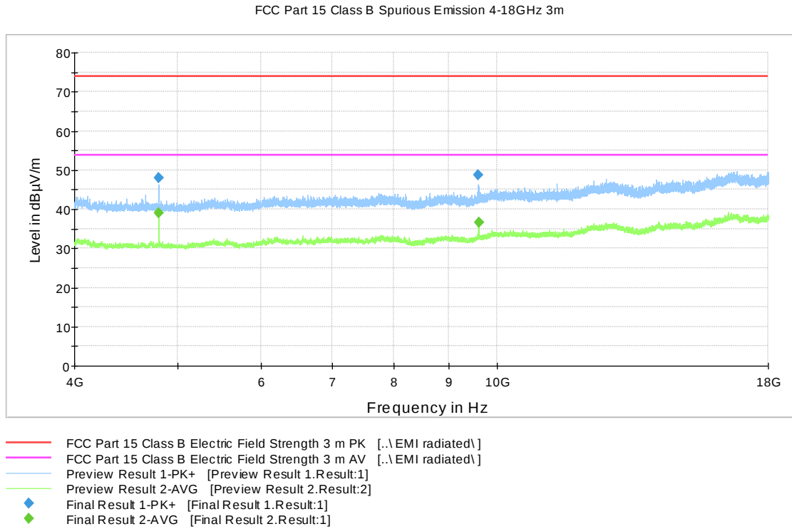
Figure 14: Channel 0 low 4 GHz – 18 GHz (A)
