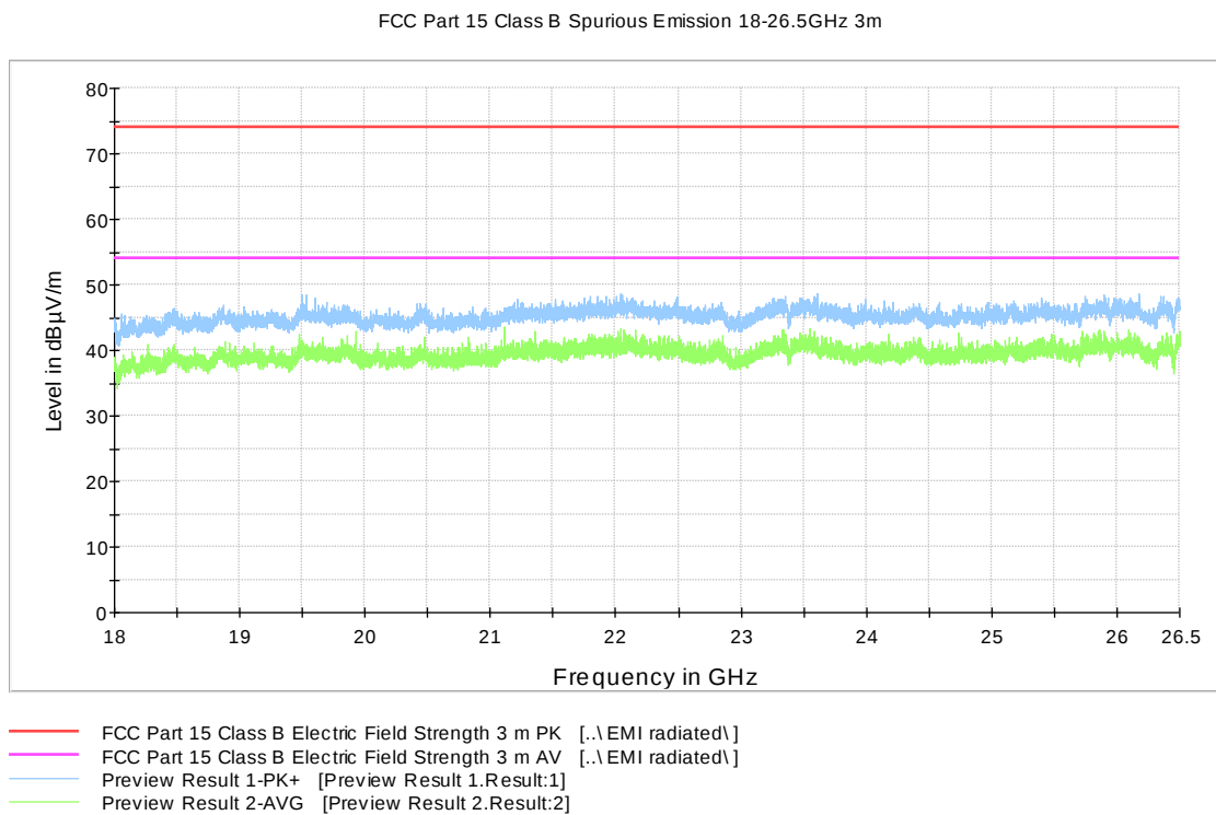
Figure 15: Channel 0 low 18 GHz – 26.5 GHz (A)
