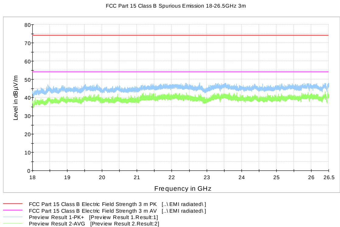
Figure 37: Channel 39 high 18 GHz – 26.5 GHz (N)
