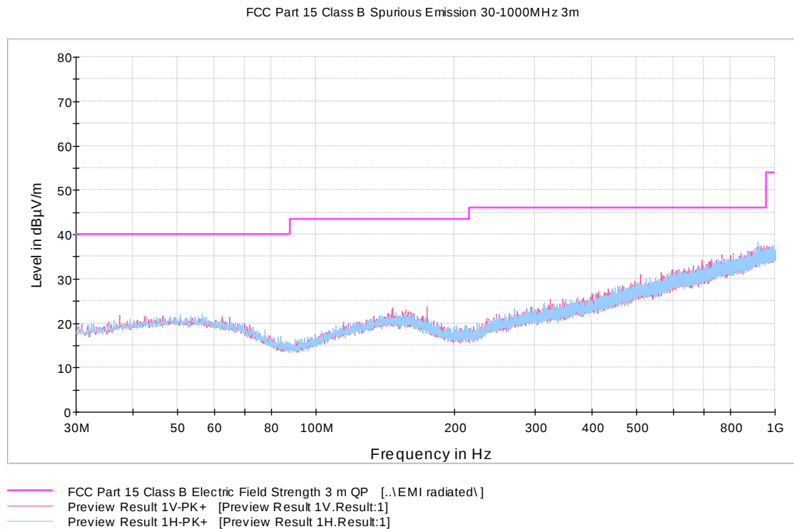
Figure 20: Channel 39 high 30 MHz – 1000 MHz (A)
