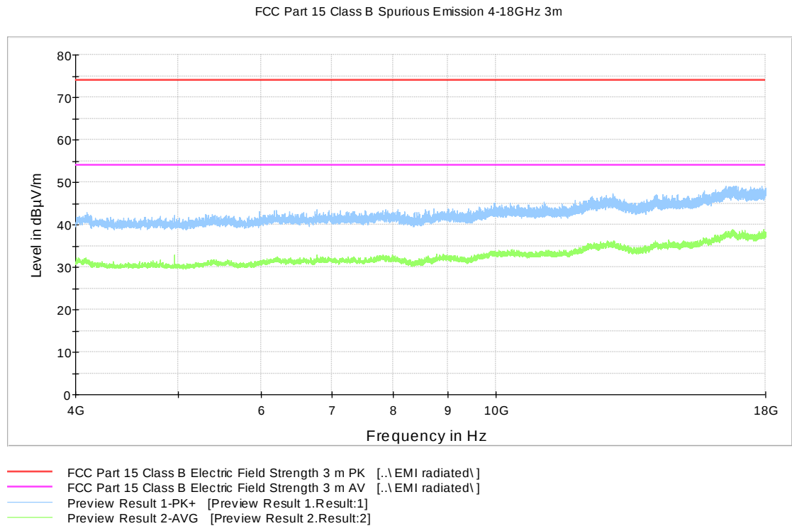
Figure 22: Channel 39 high 4 GHz – 18 GHz (A)
