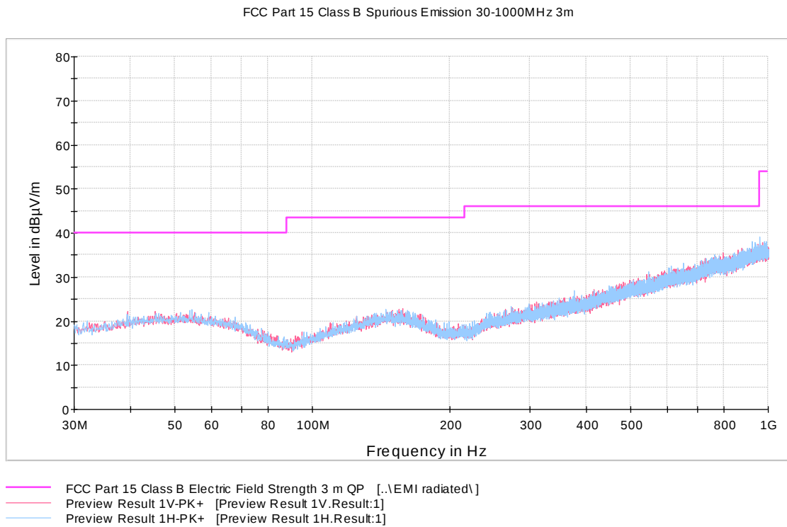
Figure 26: Channel 0 low 30 MHz – 1000 MHz (N)
