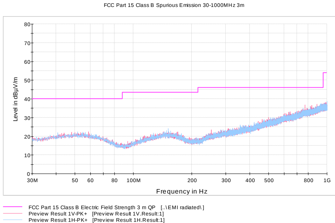
Figure 34: Channel 39 high 30 MHz – 1000 MHz (N)
