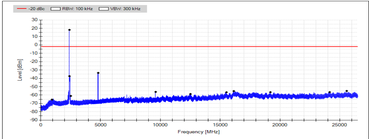
Figure 41: Conducted spurious emissions 30 - 26500 MHz channel 0, power setting 200, PHY 1M
