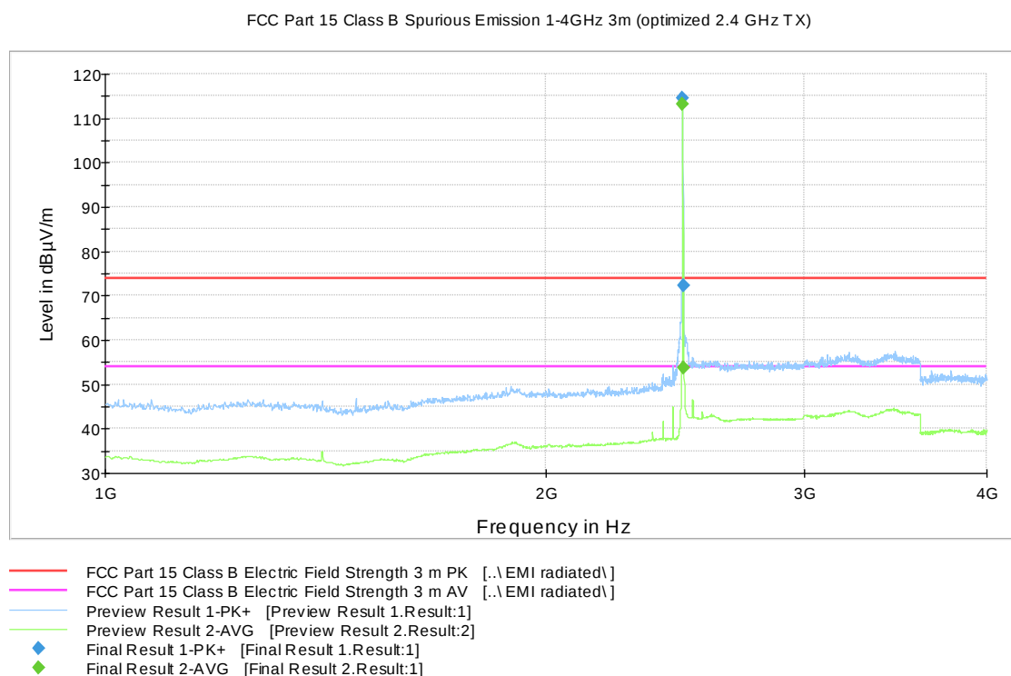
Figure 35: Channel 39 high 1 GHz – 4 GHz (N)
