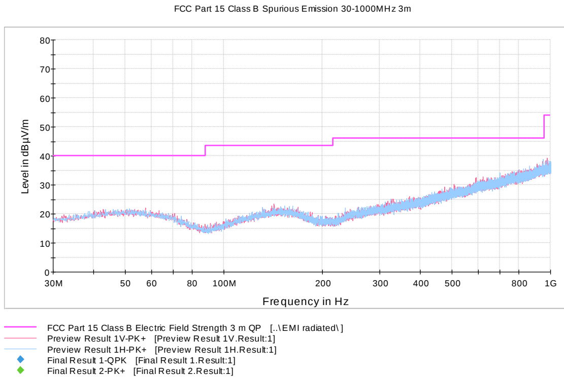
Figure 12: Channel 0 low 30 MHz – 1000 MHz (A)
