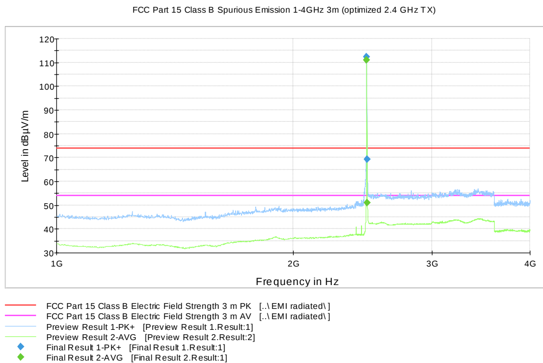
Figure 21: Channel 39 high 1 GHz – 4 GHz (A)
