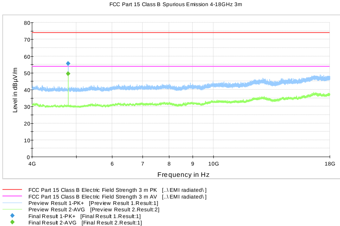
Figure 28: Channel 0 low 4 GHz – 18 GHz (N)
