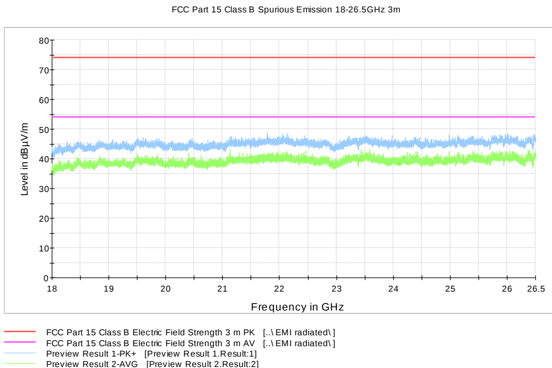
Figure 29: Channel 0 low 18 GHz – 26.5 GHz (N)
