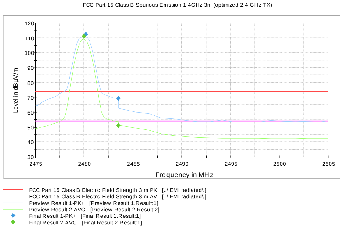
Figure 39: Radiated Band Edge measurement graph, Channel 39 high (N)
