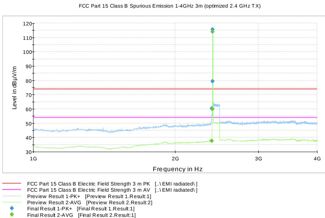
Figure 13: Channel 0 low 1 GHz – 4 GHz (A)
