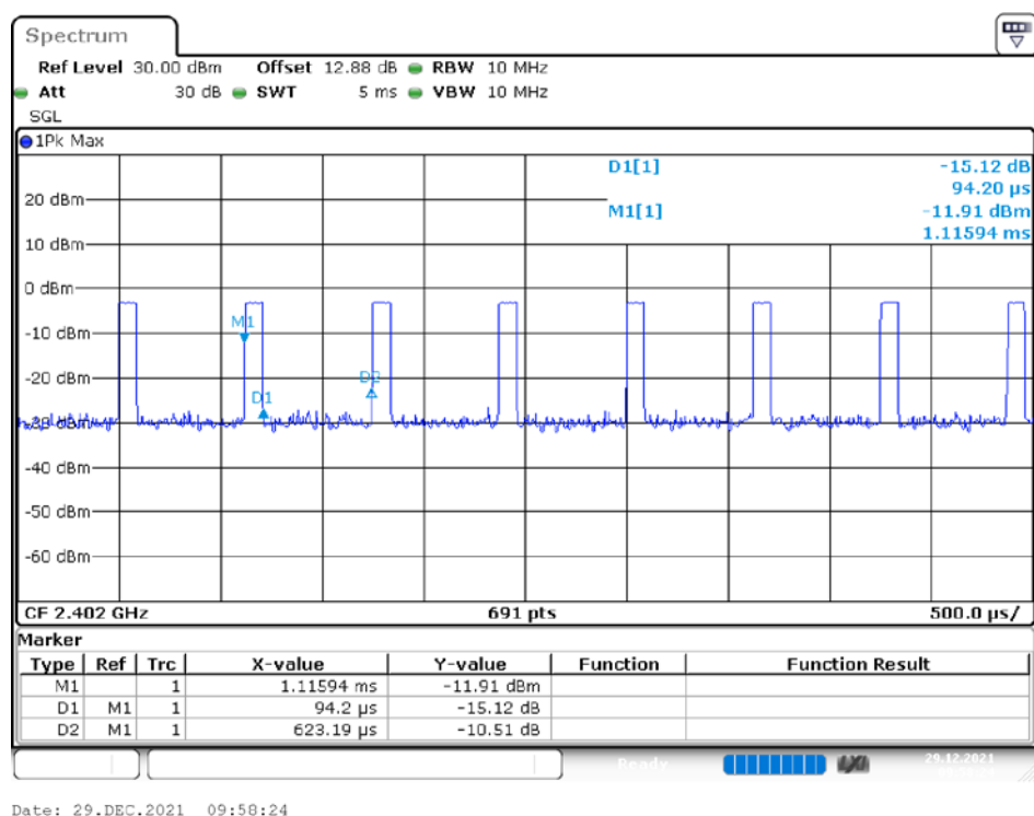
Duty Cycle, BLE_1M, Low Channel
