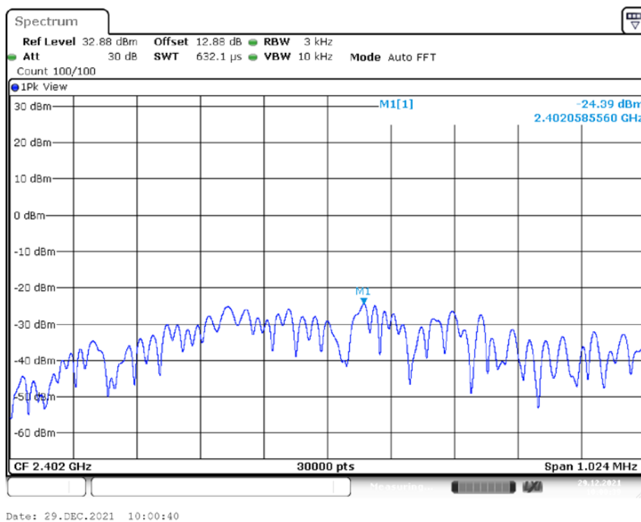
Power Spectral Density, BLE_1M Low Channel
