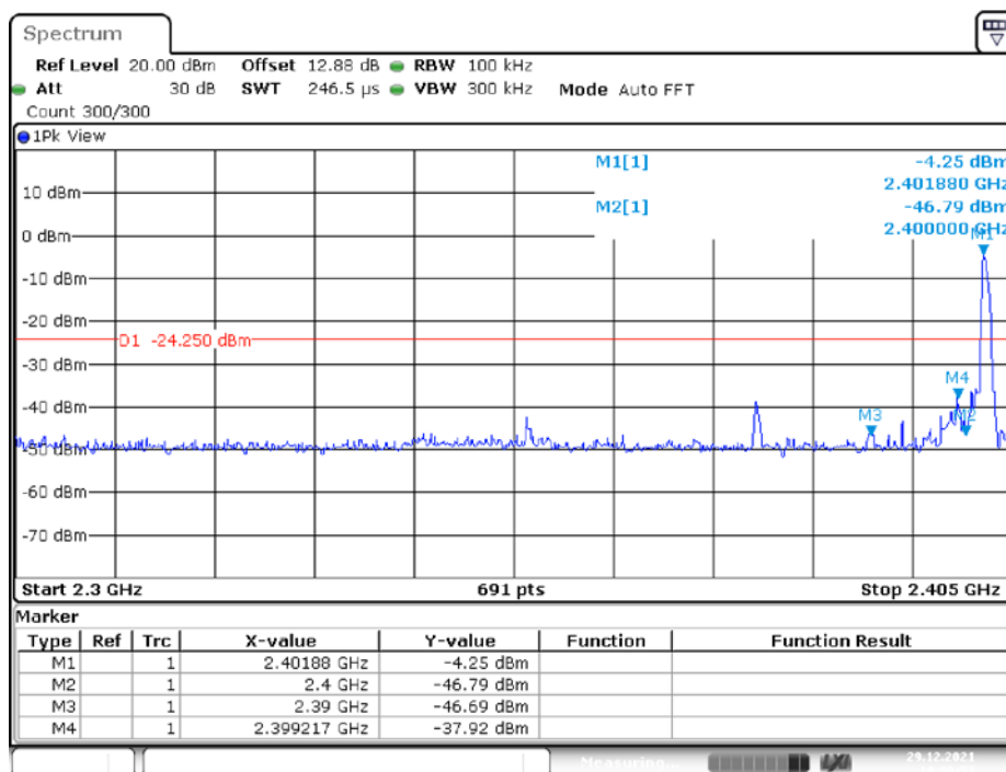
BLE_1M_Ant1_Low_2402MHz
