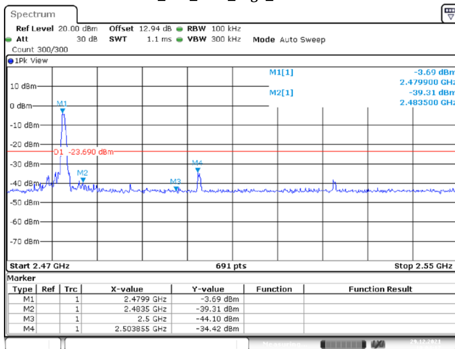
BLE_1M_Ant1_High_2480MHz
