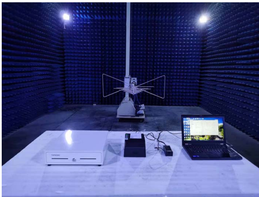
Photo of Radiated Emission Measurement Below 1GHz - Front View
