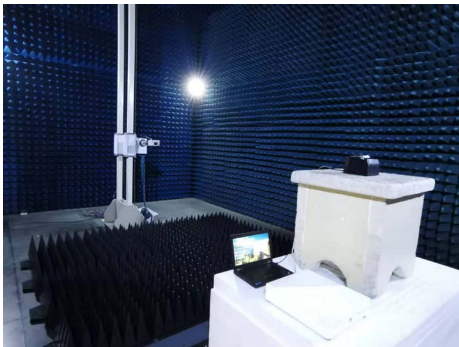
Photo of Radiated Emission Measurement 18-25GHz - Front View
