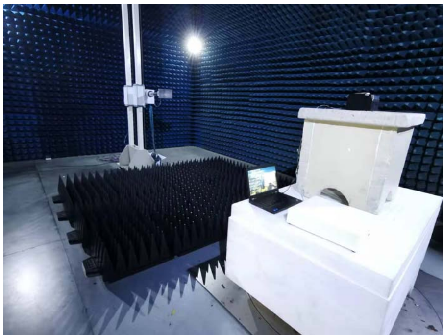
Photo of Radiated Emission Measurement 1-18GHz - Front View
