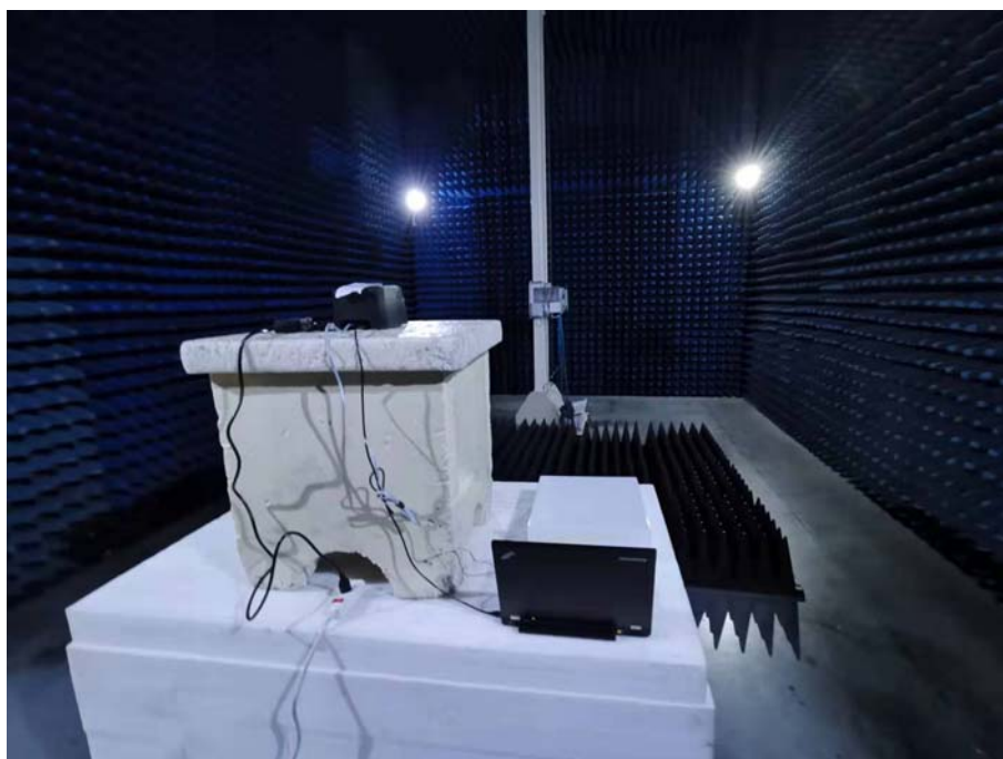
Photo of Radiated Emission Measurement 1-18GHz - Rear View
