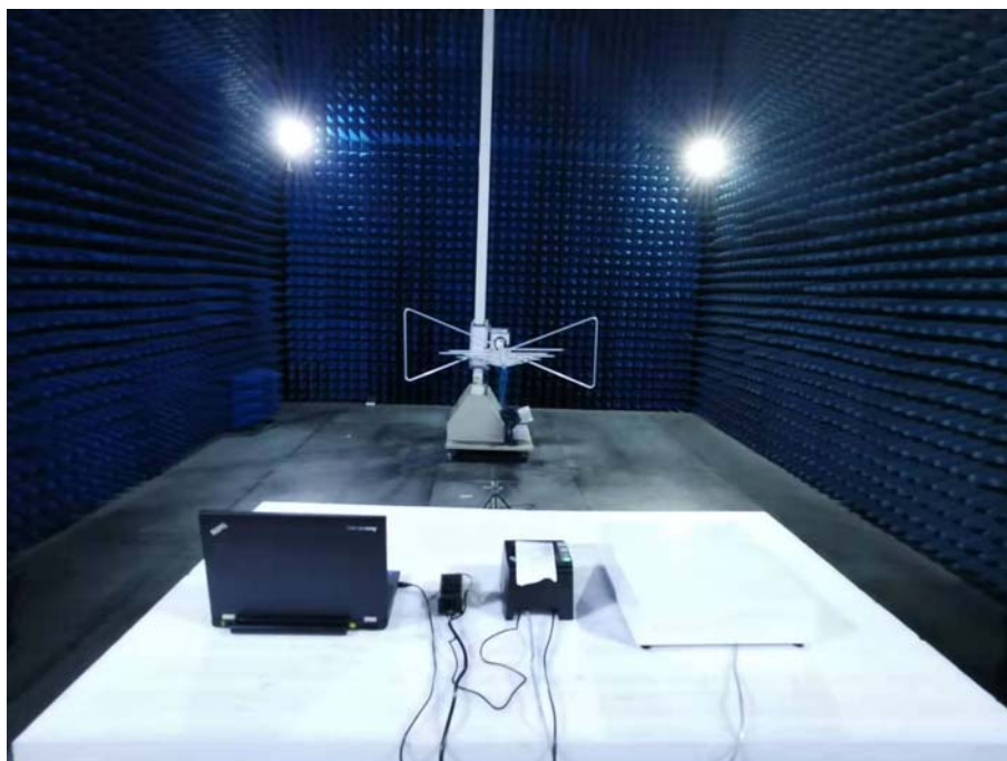
Photo of Radiated Emission Measurement Below 1GHz - Rear View
