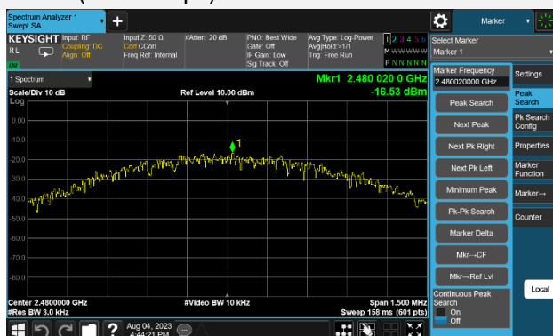
GFSK (BLE 1Mbps) HIGH CHANNEL
