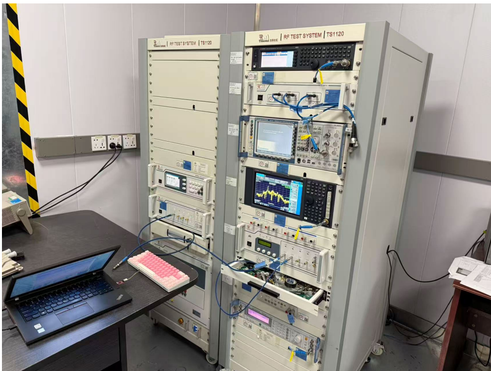
Connect EUT antenna terminal test
