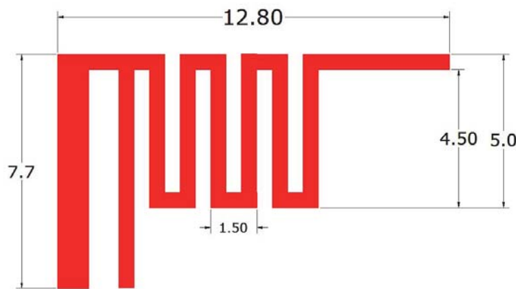
Antenna Photo & Length (mm)
