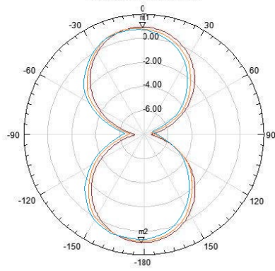
Radiation Pattern 3
