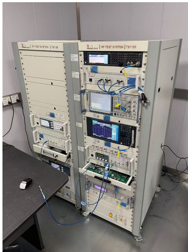
Connect EUT antenna terminal test
