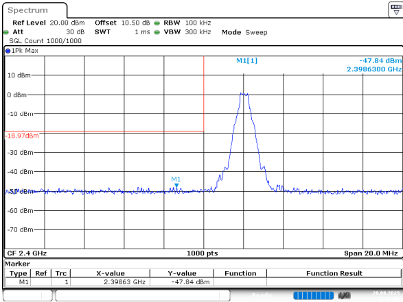
BDR_DH1_Low
