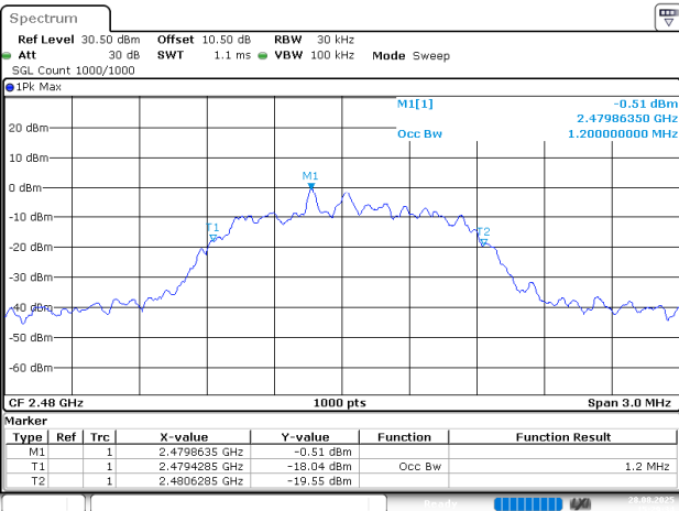
2EDR_DH1_High
