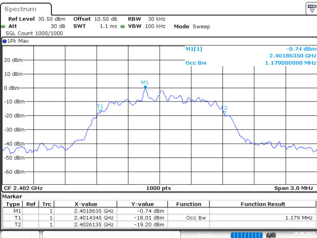
2EDR_DH1_Low
