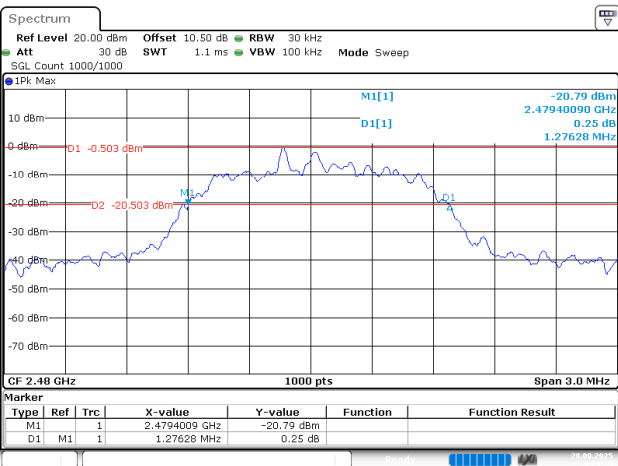
2EDR_DH1_High
