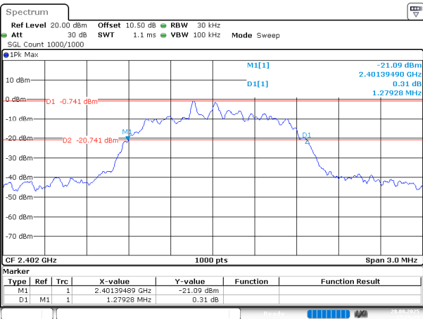
2EDR_DH1_Low
