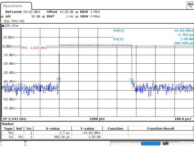
BDR_DH1_Hopping
