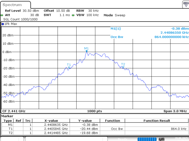
BDR_DH1_Middle
