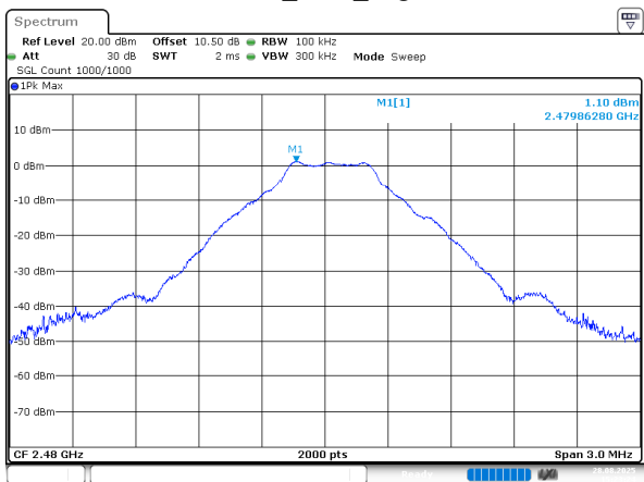
BDR_DH1_High
