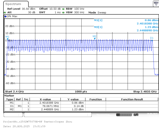
BDR_DH1_Hopping
