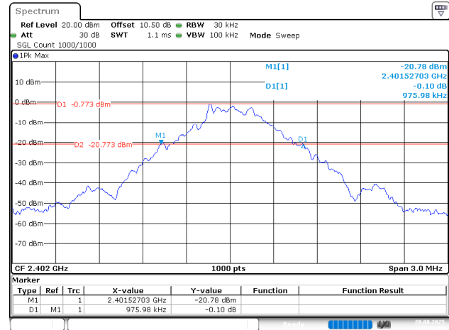
BDR_DH1_Low
