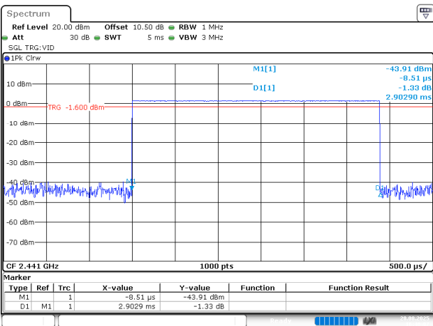
BDR_DH5_Hopping
