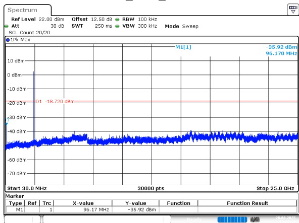
BDR_DH1_Middle
