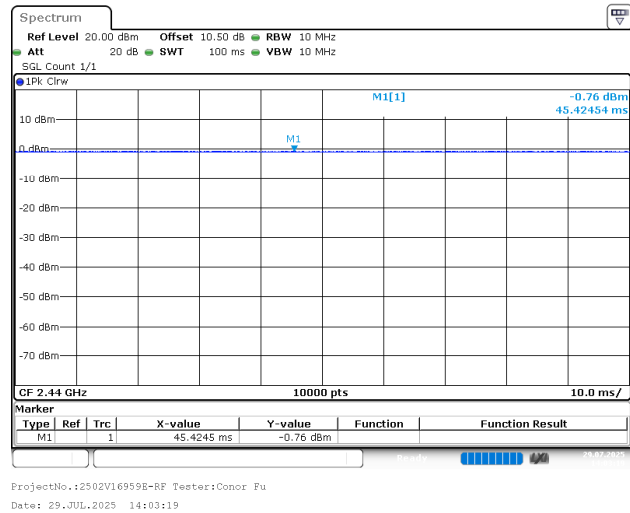
BLE_1M_Middle_Channel
