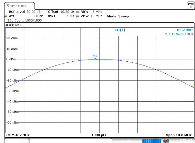
BLE_1M_Low_Channel
