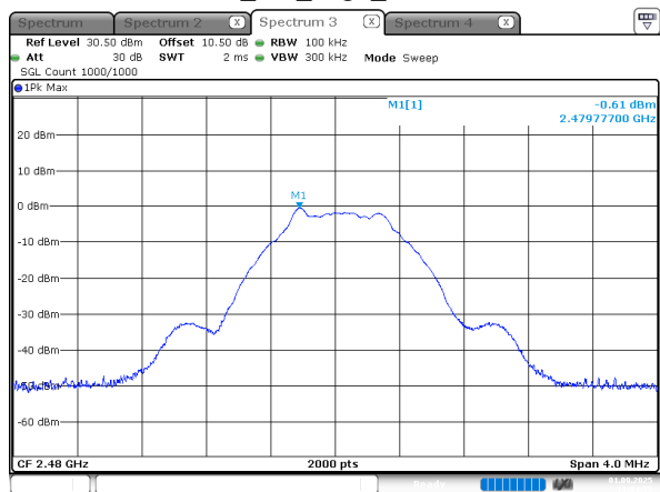
BLE_1M_High_Channel
