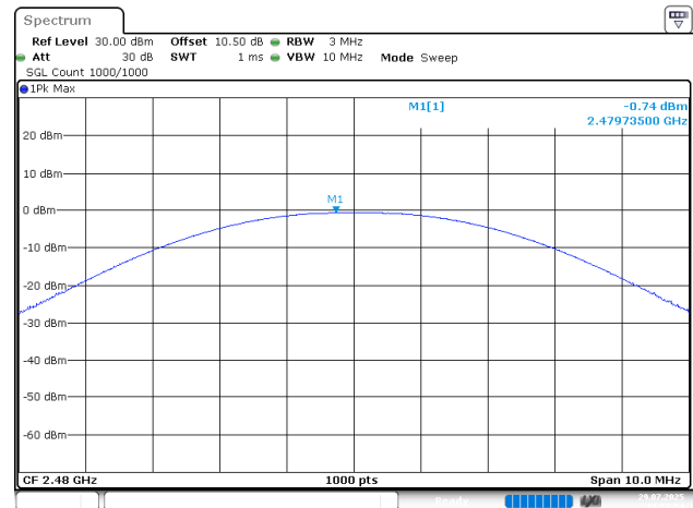
BLE_1M_High_Channel
