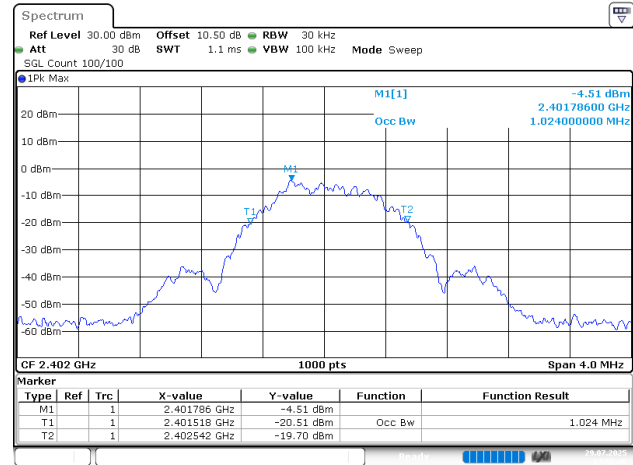
BLE_1M_Low_Channel
