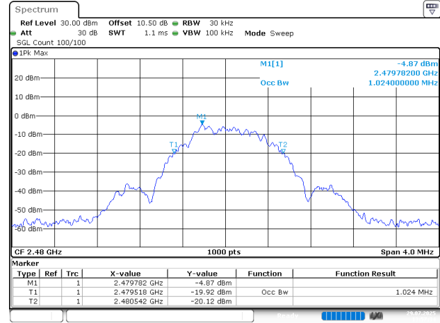
BLE_1M_High_Channel
