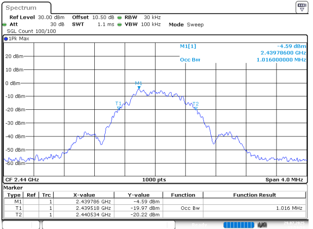
BLE_1M_Middle_Channel
