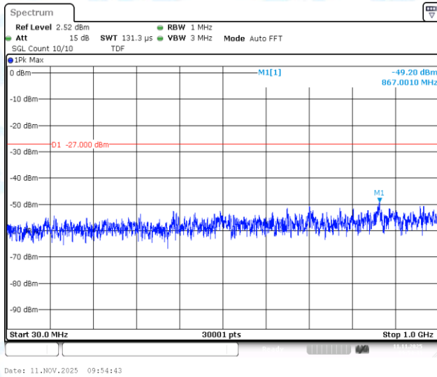
11AC20SISO-Ant1-5240-30~1000-PASS
