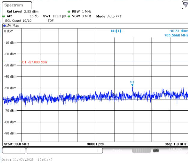
11AC20SISO-Ant1-5260-30~1000-PASS
