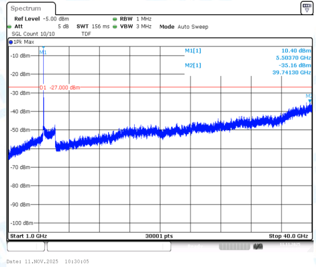
11AC20SISO-Ant1-5500-1000~40000-PASS
