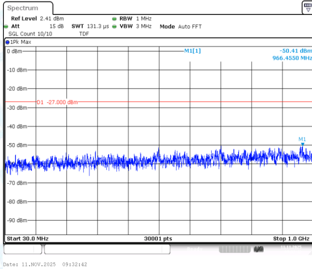
11N20SISO-Ant1-5580-30~1000-PASS
