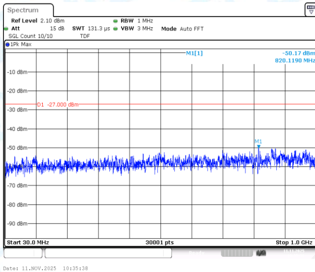
11AC20SISO-Ant1-5700-30~1000-PASS
