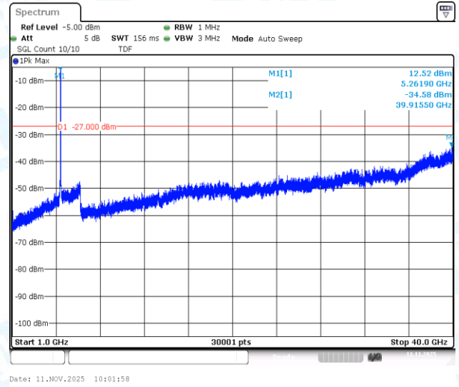
11AC20SISO-Ant1-5260-1000~40000-PASS
