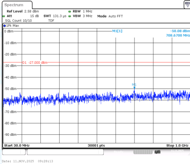
11N20SISO-Ant1-5280-30~1000-PASS
