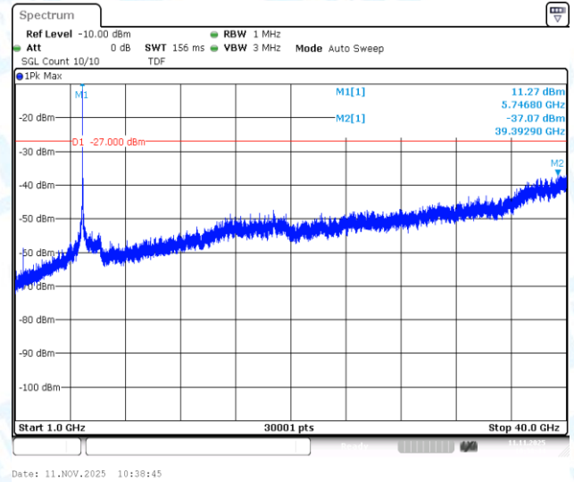
11AC20SISO-Ant1-5745-1000~40000-PASS
