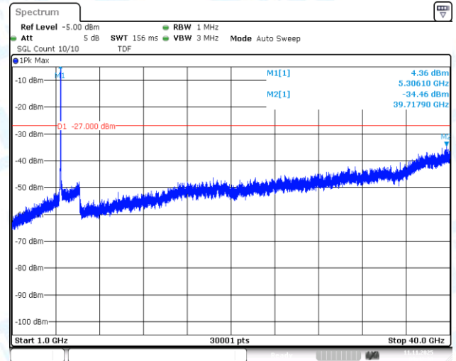
11N40SISO-Ant1-5310-1000~40000-PASS
