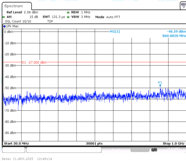
11AC40SISO-Ant1-5270-30~1000-PASS
