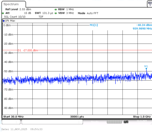
11AC20SISO-Ant1-5180-30~1000-PASS
