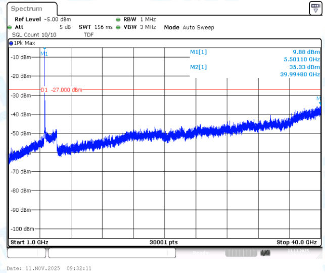
11N20SISO-Ant1-5500-1000~40000-PASS
