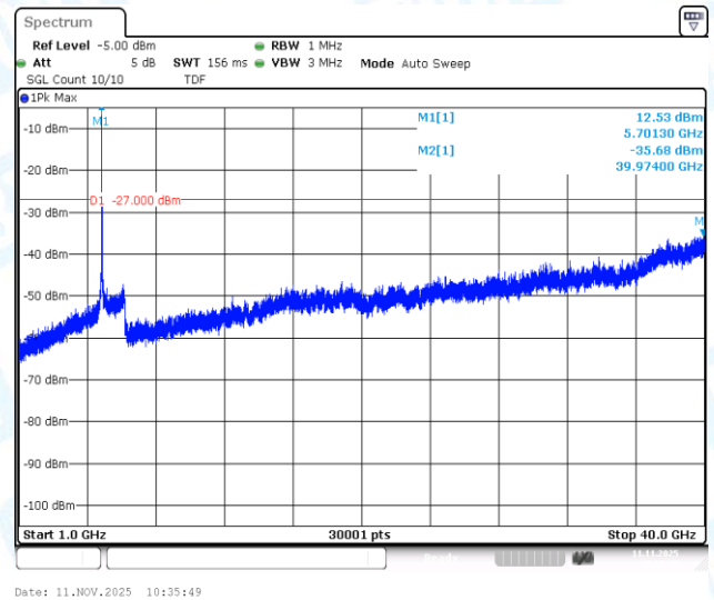
11AC20SISO-Ant1-5700-1000~40000-PASS
