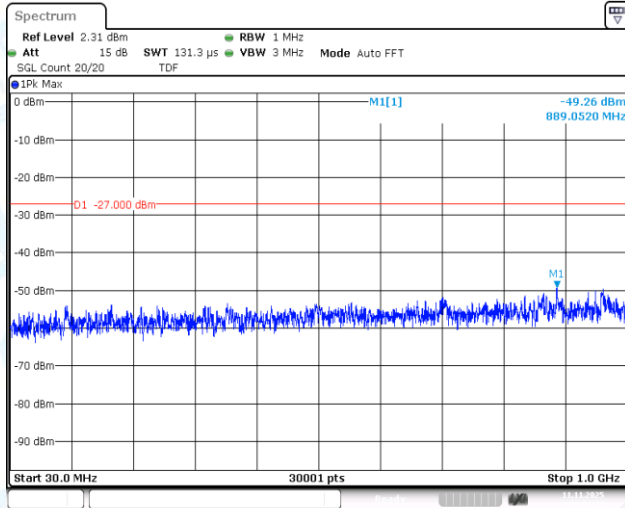
11N20SISO-Ant1-5745-30~1000-PASS
