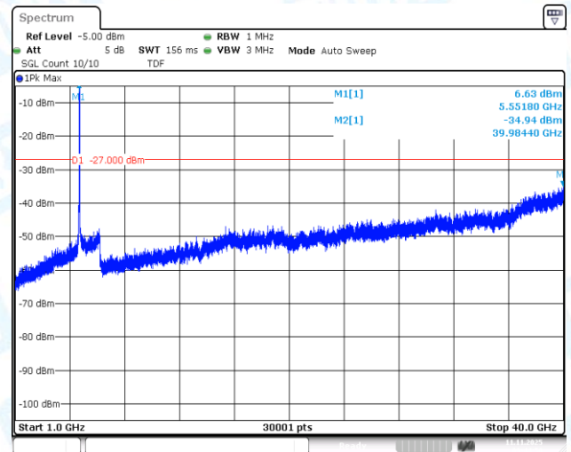
11N40SISO-Ant1-5510-1000~40000-PASS
