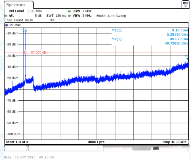
11N20SISO-Ant1-5280-1000~40000-PASS
