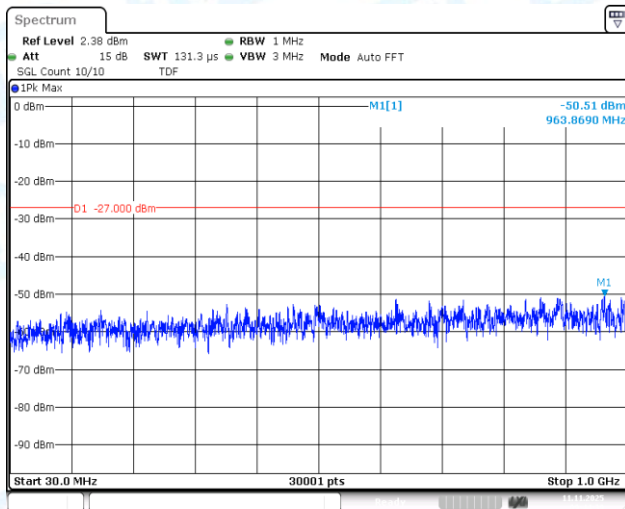
11N40SISO-Ant1-5510-30~1000-PASS
