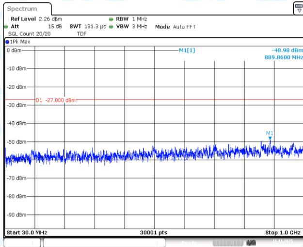
11N20SISO-Ant1-5785-30~1000-PASS
