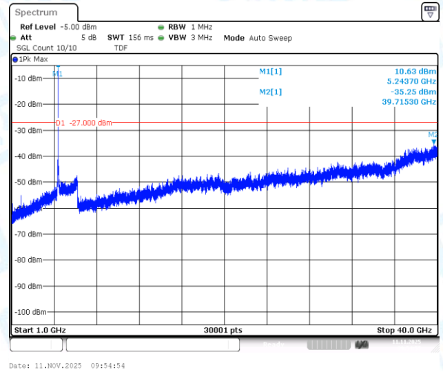
11AC20SISO-Ant1-5240-1000~40000-PASS
