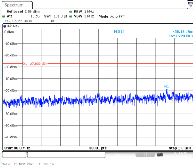
11AC20SISO-Ant1-5280-30~1000-PASS
