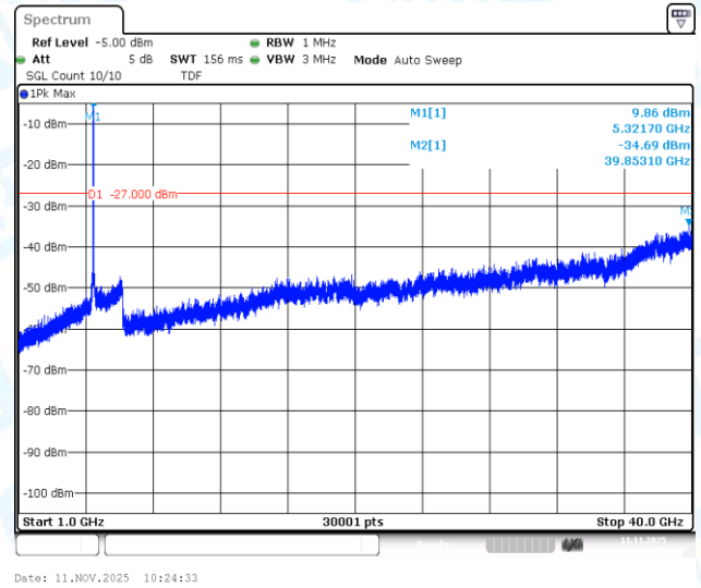
11AC20SISO-Ant1-5320-1000~40000-PASS
