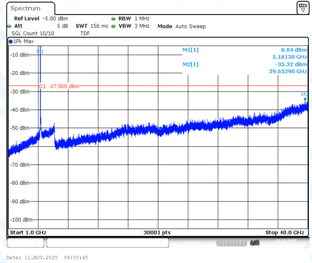
11AC20SISO-Ant1-5180-1000~40000-PASS
