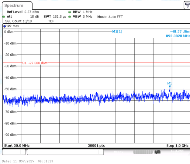
11N20SISO-Ant1-5320-30~1000-PASS
