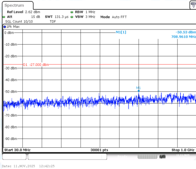
11AC40SISO-Ant1-5190-30~1000-PASS
