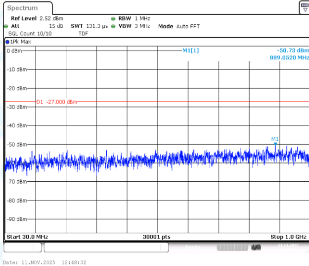
11AC40SISO-Ant1-5230-30~1000-PASS
