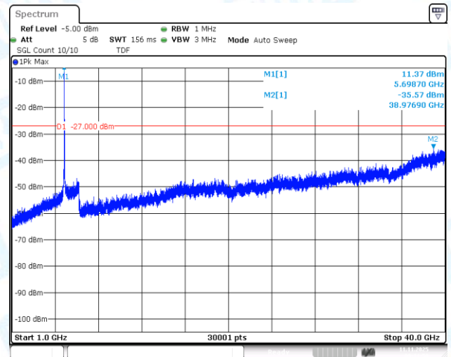
11A-Ant1-5700-1000~40000-PASS
