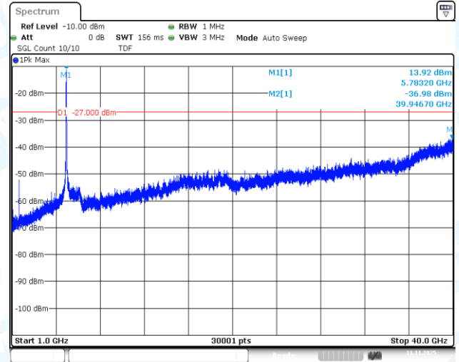
11N20SISO-Ant1-5745-1000~40000-PASS
