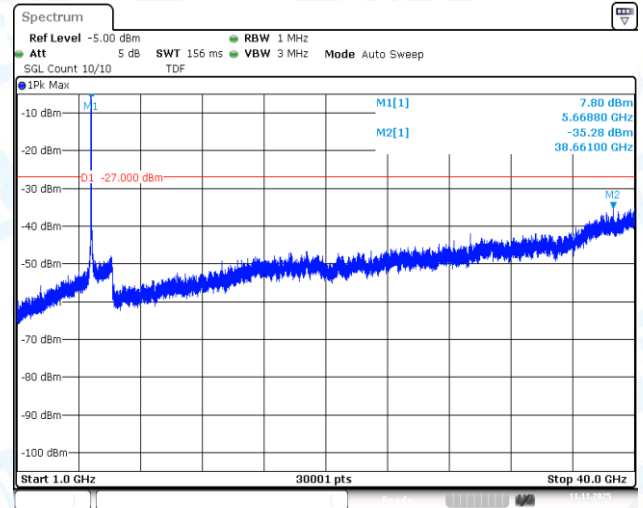
11N40SISO-Ant1-5670-1000~40000-PASS
