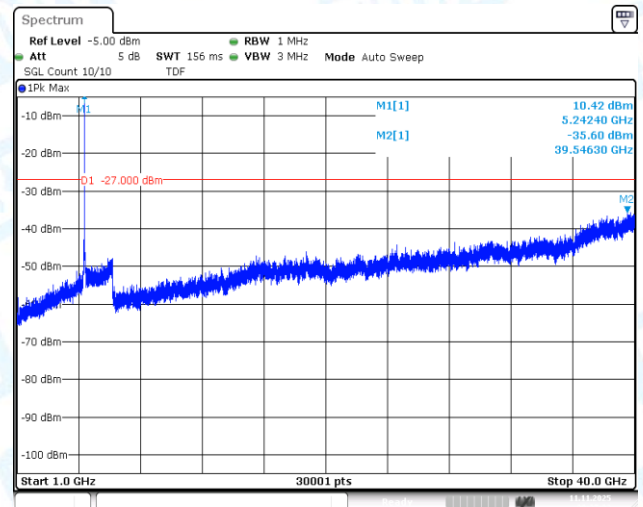
11N20SISO-Ant1-5240-1000~40000-PASS
