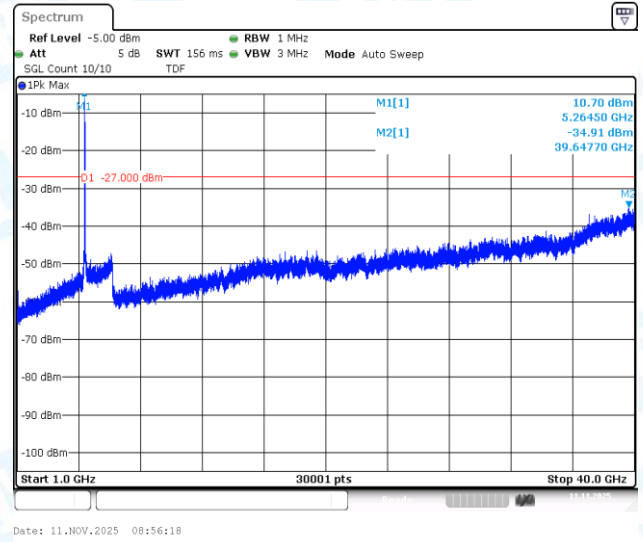
11A-Ant1-5260-1000~40000-PASS
