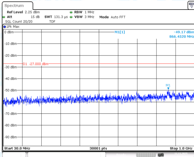
11N40SISO-Ant1-5670-30~1000-PASS
