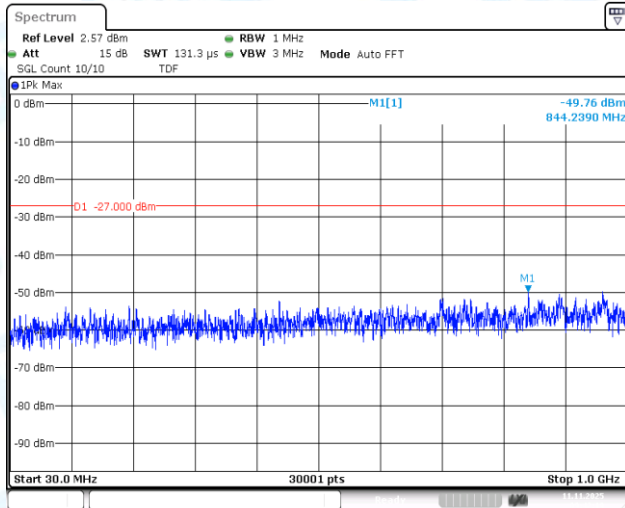
11N40SISO-Ant1-5310-30~1000-PASS
