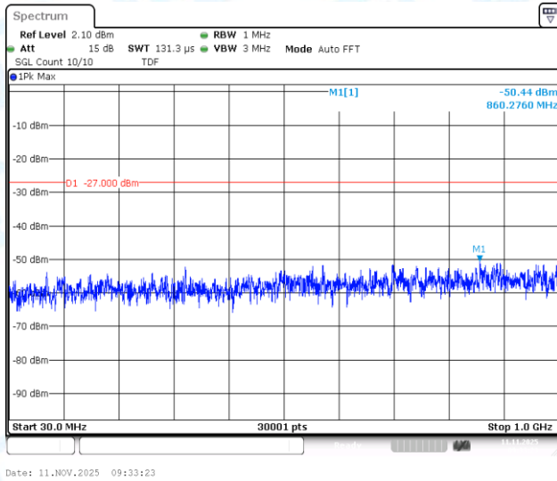
11N20SISO-Ant1-5700-30~1000-PASS
