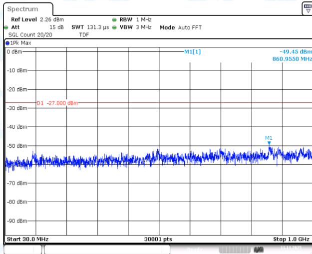
11A-Ant1-5785-30~1000-PASS
