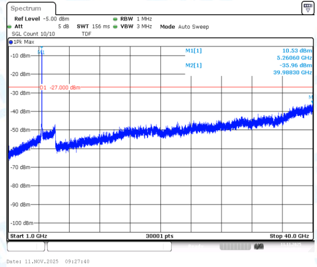
11N20SISO-Ant1-5260-1000~40000-PASS
