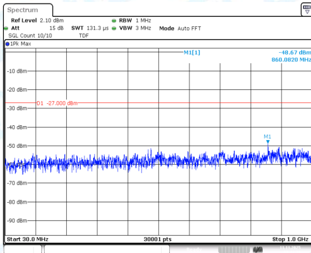
11A-Ant1-5580-30~1000-PASS
