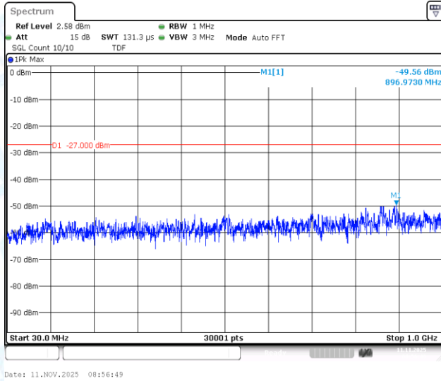
11A-Ant1-5280-30~1000-PASS
