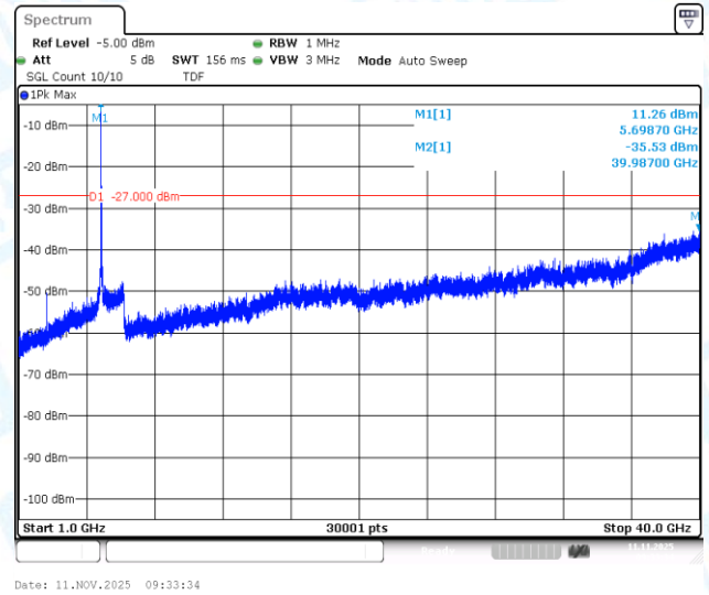
11N20SISO-Ant1-5700-1000~40000-PASS
