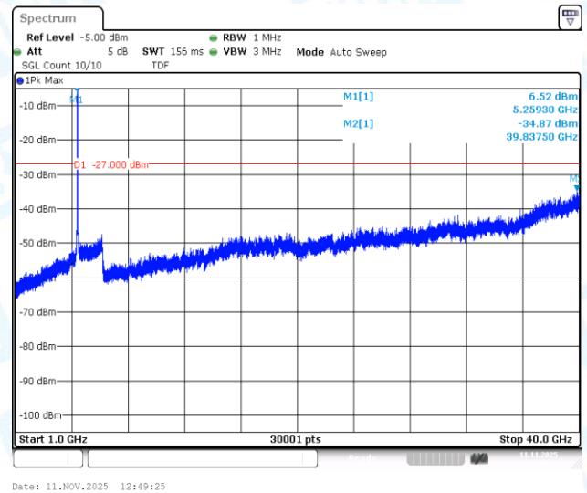
11AC40SISO-Ant1-5270-1000~40000-PASS
