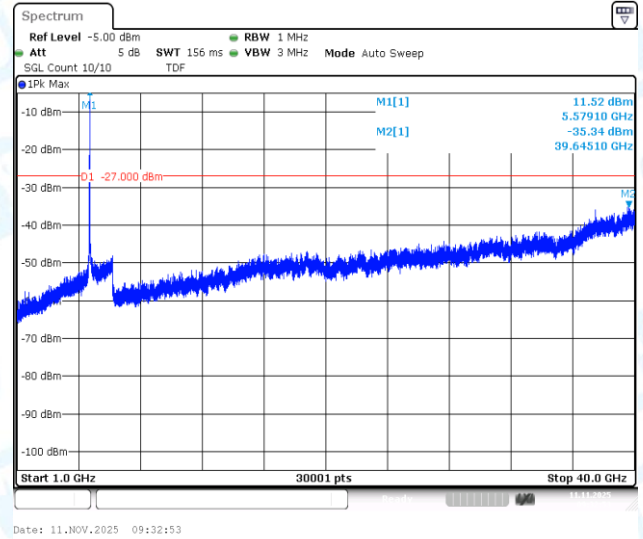
11N20SISO-Ant1-5580-1000~40000-PASS
