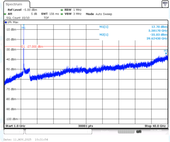
11AC20SISO-Ant1-5580-1000~40000-PASS
