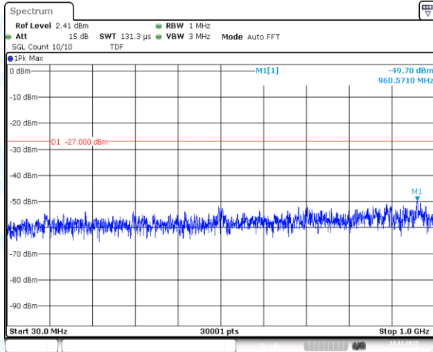
11A-Ant1-5500-30~1000-PASS
