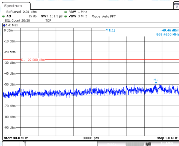
11N40SISO-Ant1-5755-30~1000-PASS
