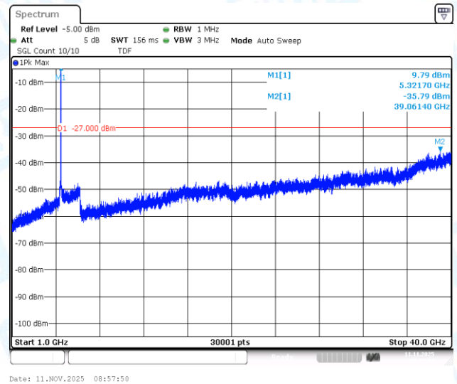
11A-Ant1-5320-1000~40000-PASS
