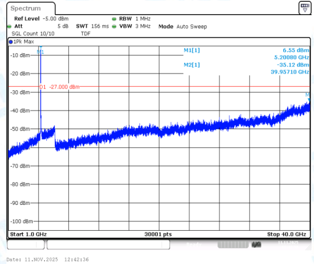
11AC40SISO-Ant1-5190-1000~40000-PASS
