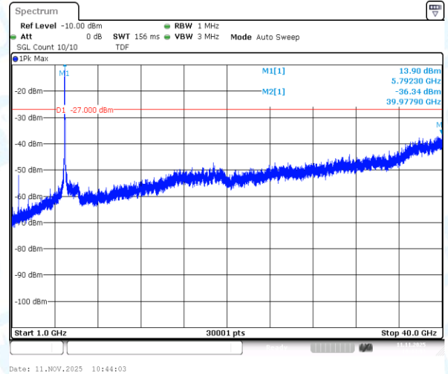
11AC20SISO-Ant1-5785-1000~40000-PASS
