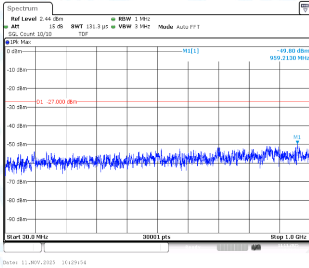
11AC20SISO-Ant1-5500-30~1000-PASS
