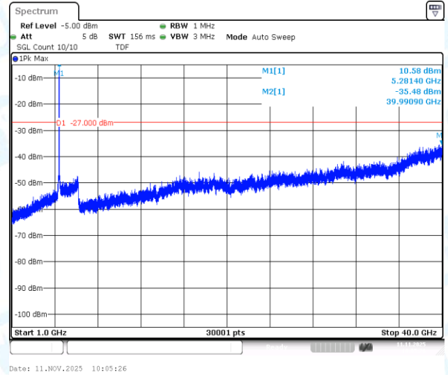
11AC20SISO-Ant1-5280-1000~40000-PASS
