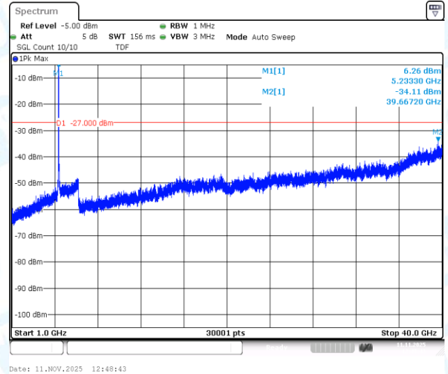
11AC40SISO-Ant1-5230-1000~40000-PASS
