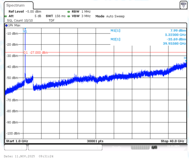
11N20SISO-Ant1-5320-1000~40000-PASS
