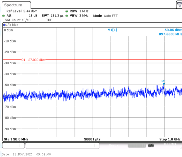
11N20SISO-Ant1-5500-30~1000-PASS
