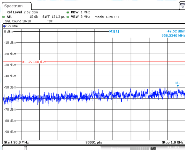
11N20SISO-Ant1-5200-30~1000-PASS
