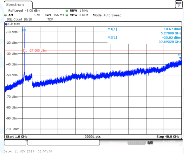
11A-Ant1-5280-1000~40000-PASS
