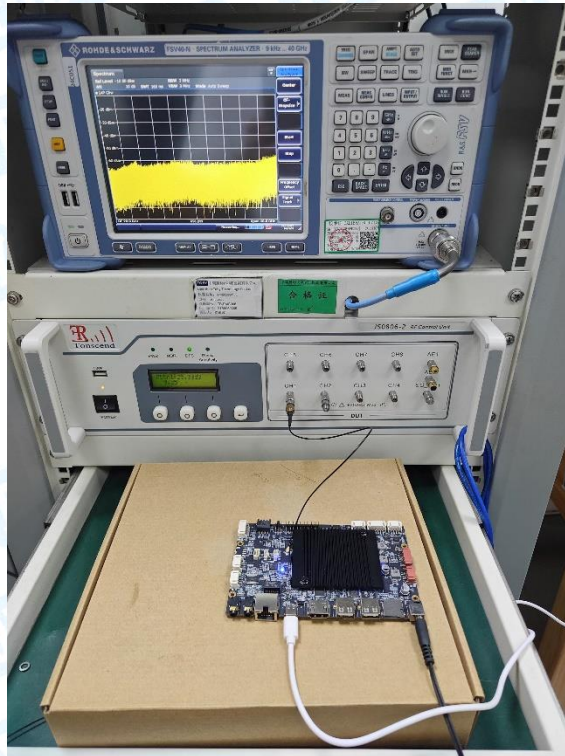
Photo of Setup for DFS
