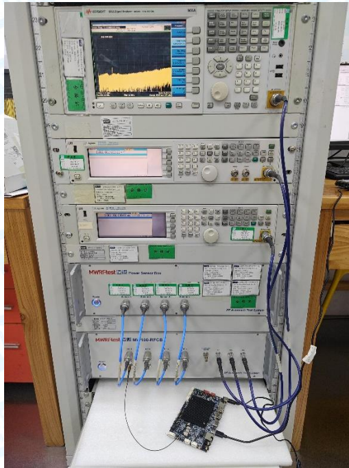
Photo of Setup for RF Conducted----BT
