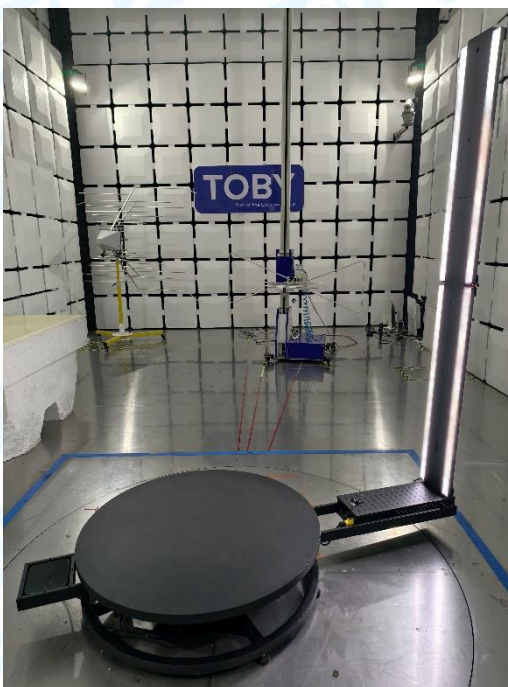
Radiated Emission Test Setup-Below 1G
