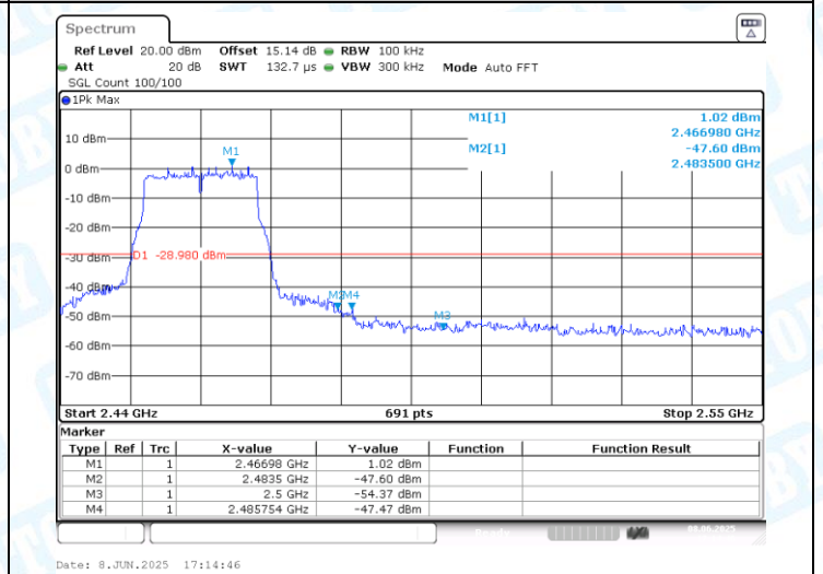
11N20SISO-Ant1-2462-PASS
