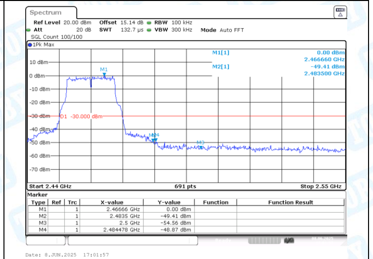
11G-Ant1-2462-PASS
