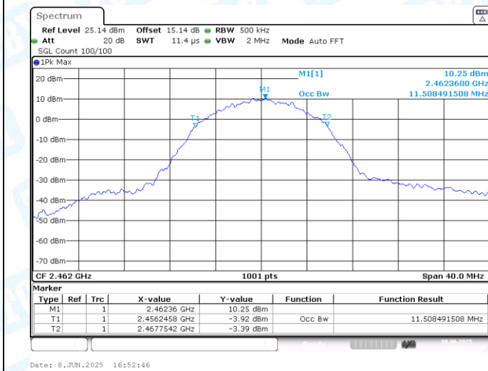
11B-Ant1-2462
