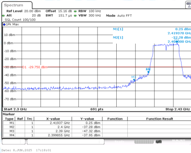
11AX20SISO-Ant1-2412-PASS
