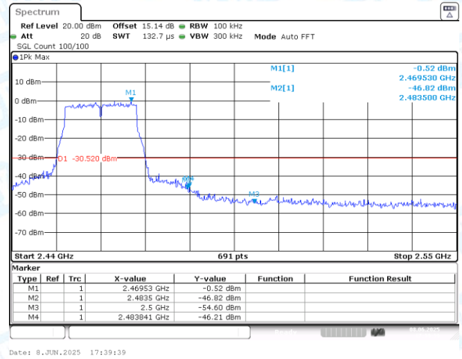
11AX20SISO-Ant1-2462-PASS
