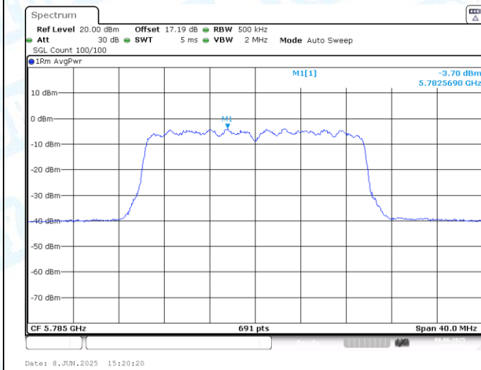
11AX20SISO-Ant1-5785-PASS
