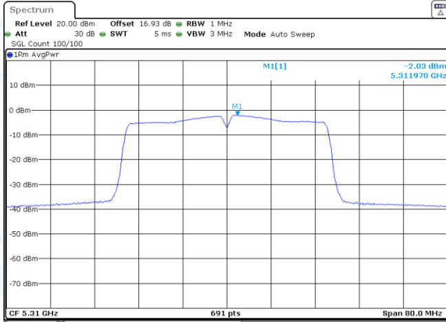
11AC40ISO-Ant1-5310-PASS
