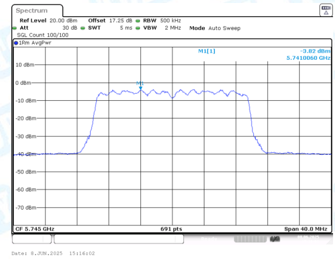
11AX20SISO-Ant1-5745-PASS
