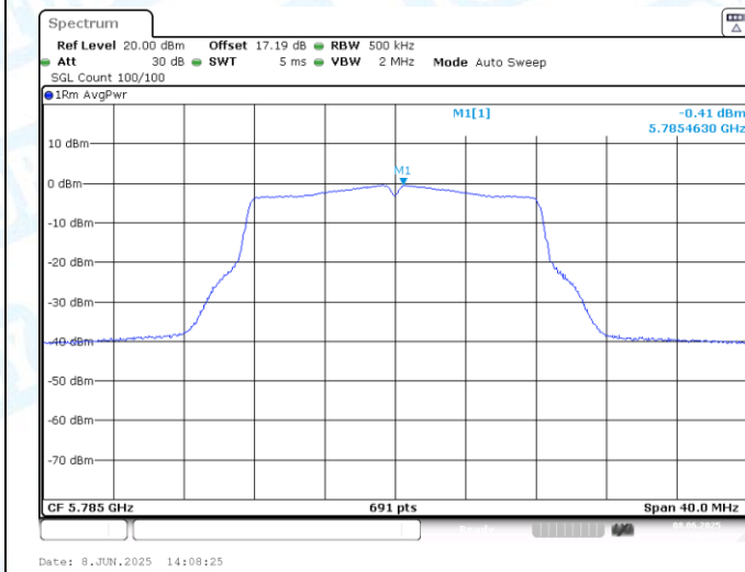
11A-Ant1-5785-PASS
