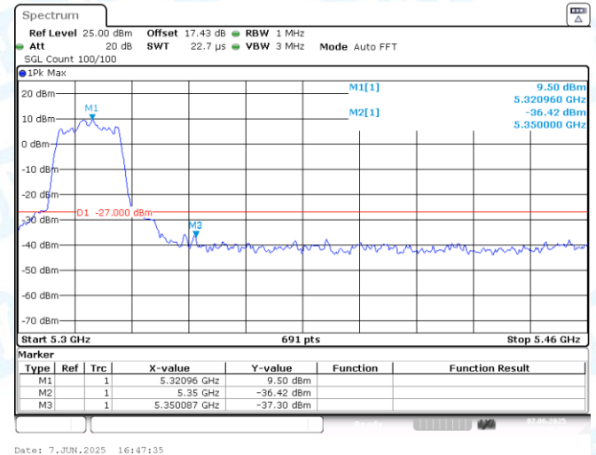
11N20SISO-Ant1-5320-PASS
