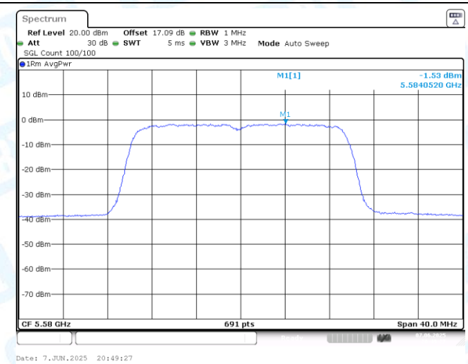
11AX20SISO-Ant1-5580-PASS
