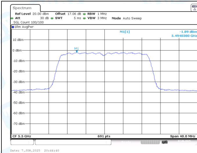
11AX20SISO-Ant1-5500-PASS
