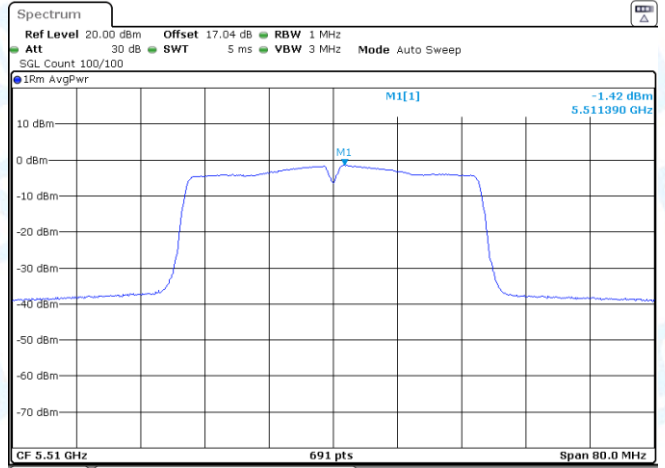
11AC40ISO-Ant1-5510-PASS
