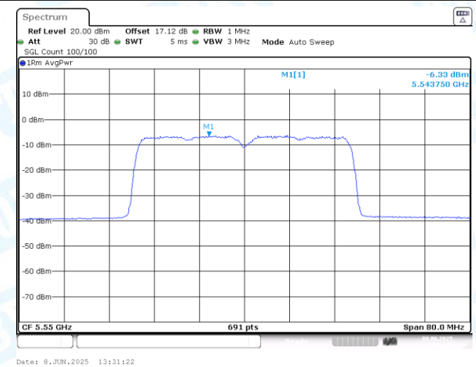
11AX40SISO-Ant1-5550-PASS
