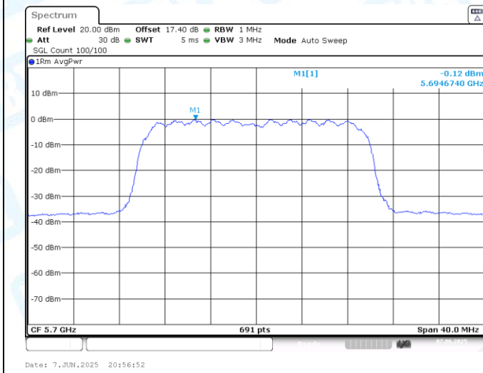
11AX20SISO-Ant1-5700-PASS
