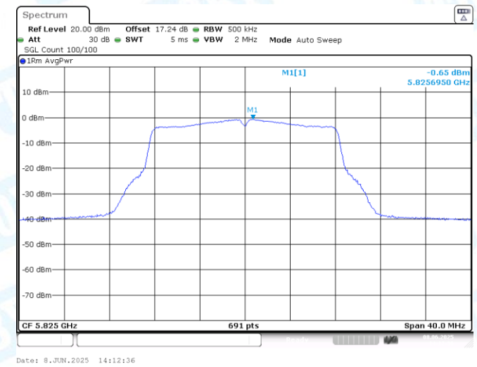
11A-Ant1-5825-PASS
