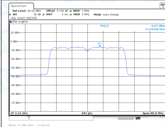
11AX40SISO-Ant1-5510-PASS
