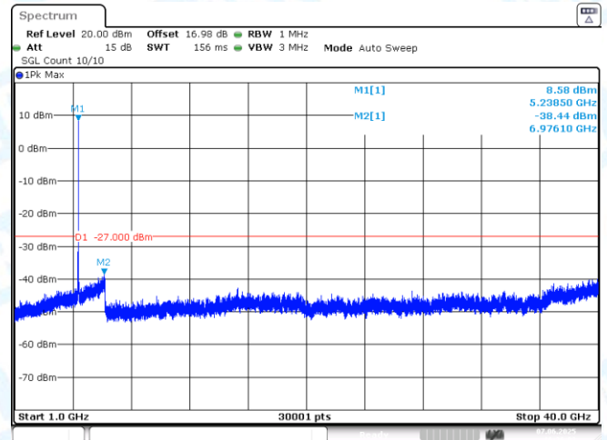
11N20SISO-Ant1-5200-1000~40000-PASS
