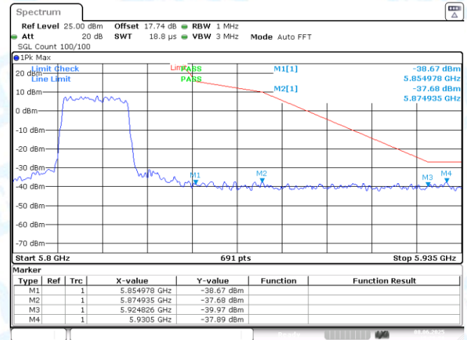
11AC40SISO-Ant1-5795-PASS
