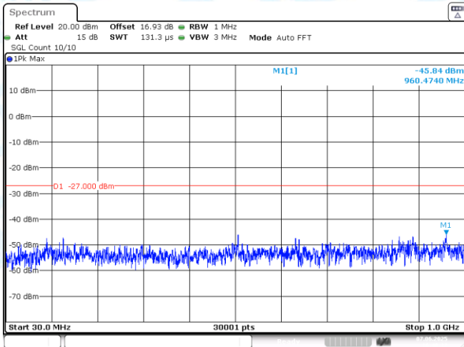
11N20SISO-Ant1-5280-30~1000-PASS
