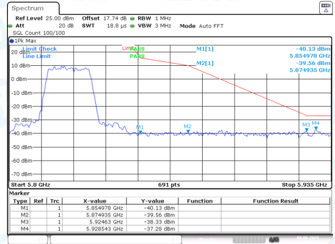
11AC20SISO-Ant1-5825-PASS
