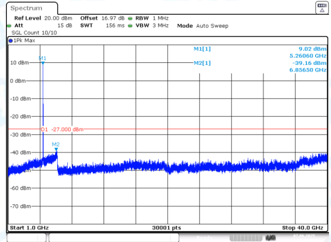
11A-Ant1-5260-1000~40000-PASS
