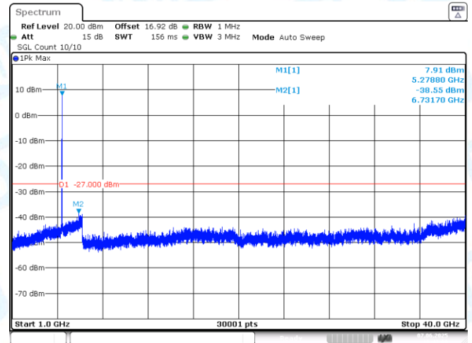
11N20SISO-Ant1-5260-1000~40000-PASS
