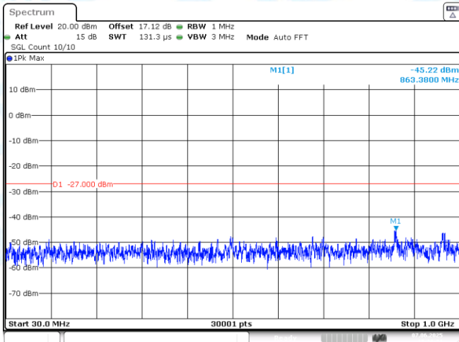
11N40SISO-Ant1-5510-30~1000-PASS
