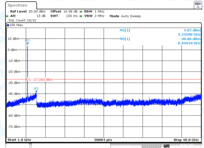
11AC40SISO-Ant1-5190-1000~40000-PASS
