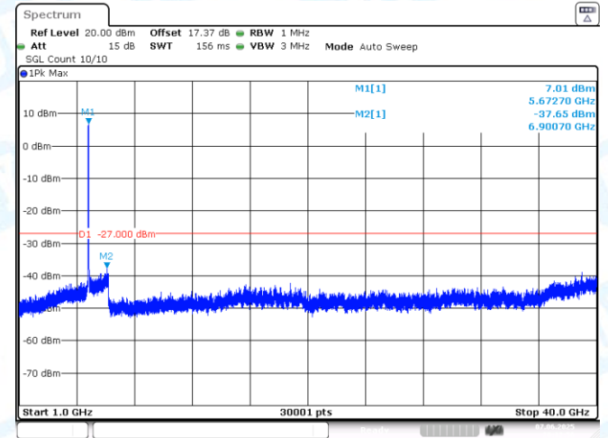
11AC40SISO-Ant1-5670-1000~40000-PASS
