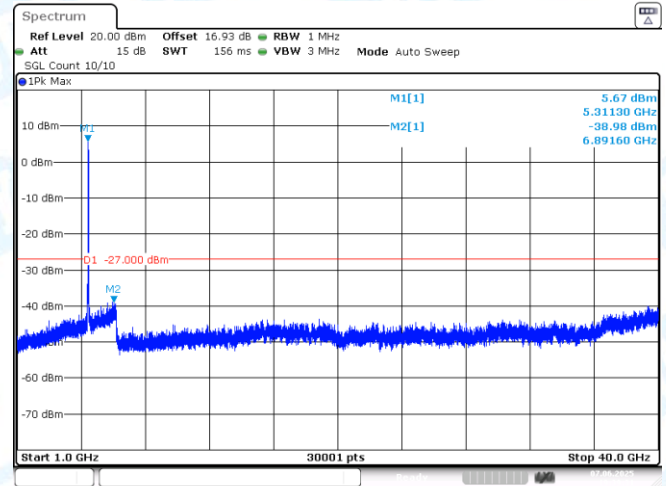
11AC40SISO-Ant1-5310-1000~40000-PASS
