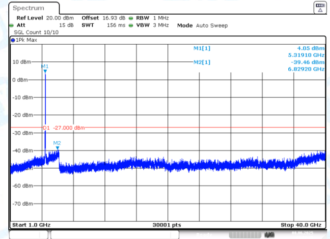
11AX40SISO-Ant1-5310-1000~40000-PASS
