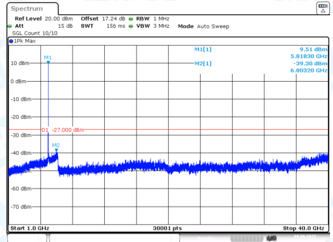
11AX20SISO-Ant1-5785-1000~40000-PASS
