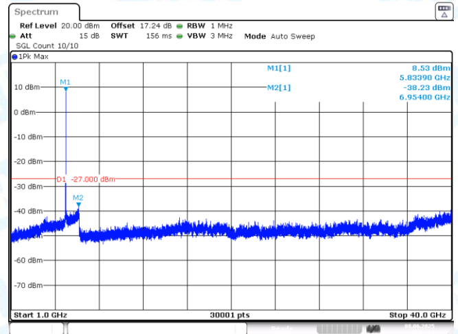
11AC20SISO-Ant1-5785-1000~40000-PASS
