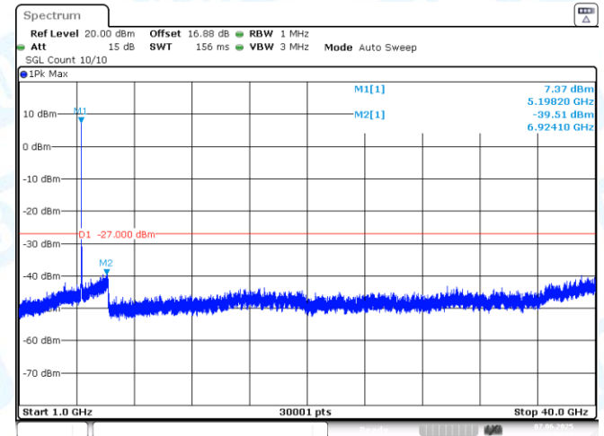
11AX20SISO-Ant1-5180-1000~40000-PASS
