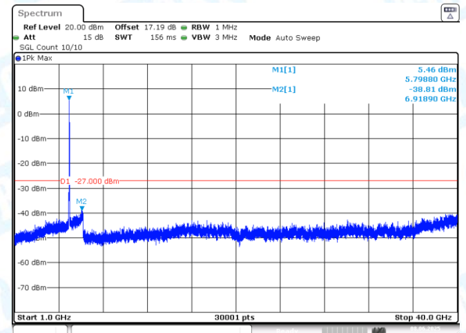
11AX40SISO-Ant1-5755-1000~40000-PASS
