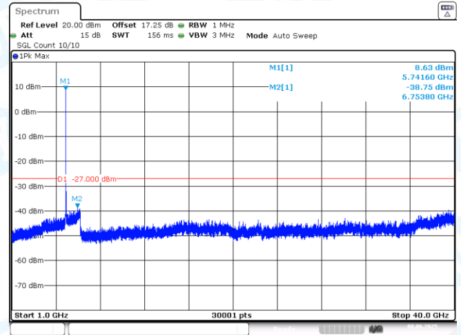
11AX20SISO-Ant1-5745-1000~40000-PASS
