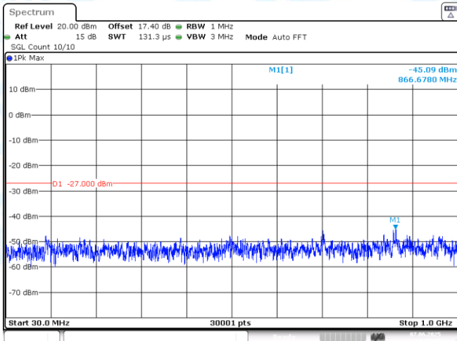
11AC20SISO-Ant1-5580-30~1000-PASS
