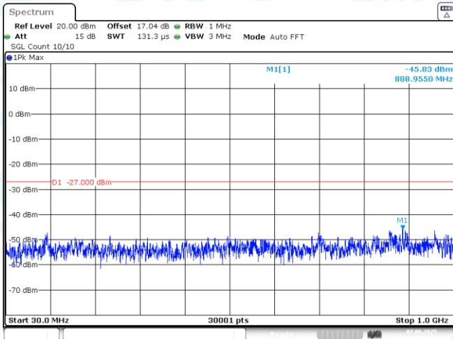
11AC40SISO-Ant1-5310-30~1000-PASS
