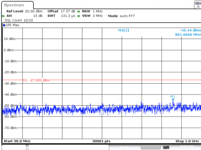
11AC40SISO-Ant1-5670-30~1000-PASS
