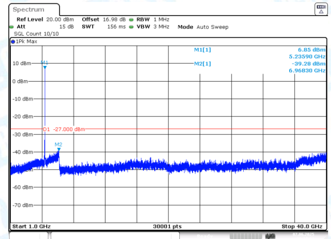
11AX20SISO-Ant1-5200-1000~40000-PASS
