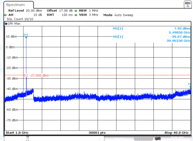
11AC20SISO-Ant1-5500-1000~40000-PASS
