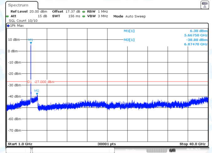
11AX40SISO-Ant1-5670-1000~40000-PASS
