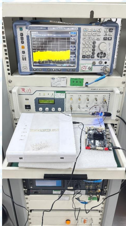
Photo of Setup for DFS
