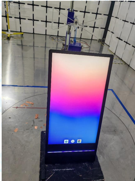
Photo of Setup for Radiated Emission (Below 1 GHz)
