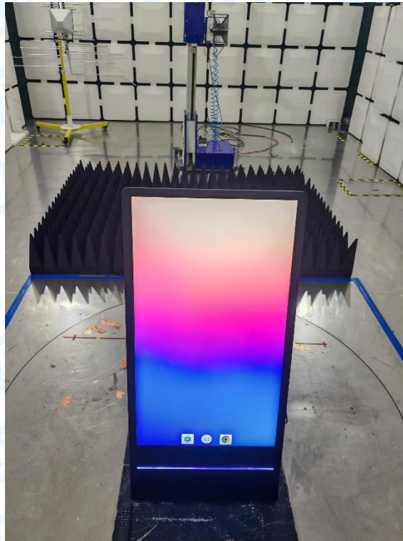
Photo of Setup for Radiated Emission (Above 1 GHz)
