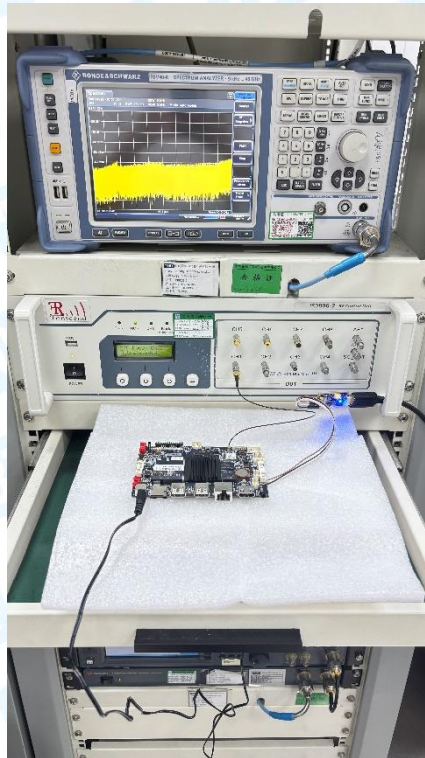
Photo of Setup for DFS
