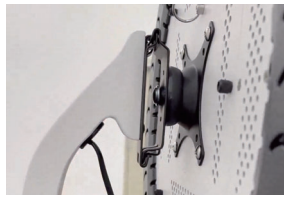
Step 13: Install Panel to Ring Light Bracket and screw it up
