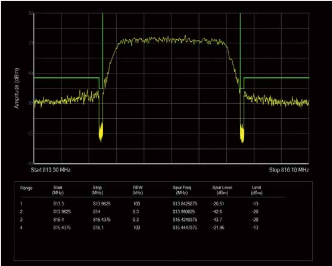
Band26a QPSK BW=1.4MHz Channel=26697 RB Size=1 Position=#Max
