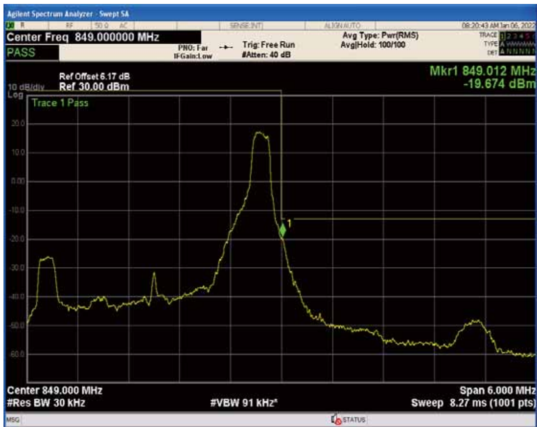
Band26b QAM16 BW=3MHz Channel=27025 RB Size=1 Position=#Max
