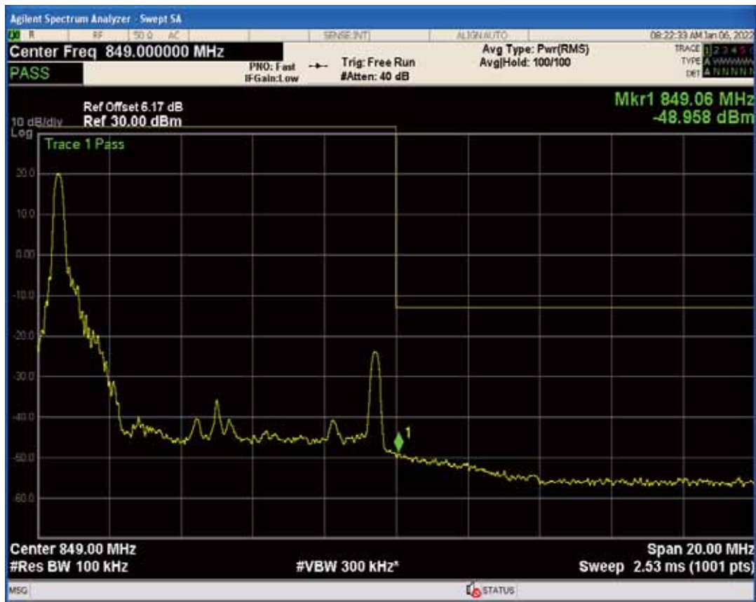
Band26b QAM16 BW=10MHz Channel=26990 RB Size=1 Position=#Max
