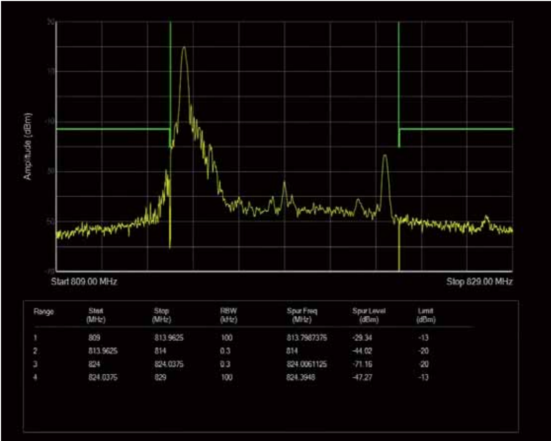
Band26a QAM16 BW=10MHz Channel=26740 RB Size=1 Position=#Max
