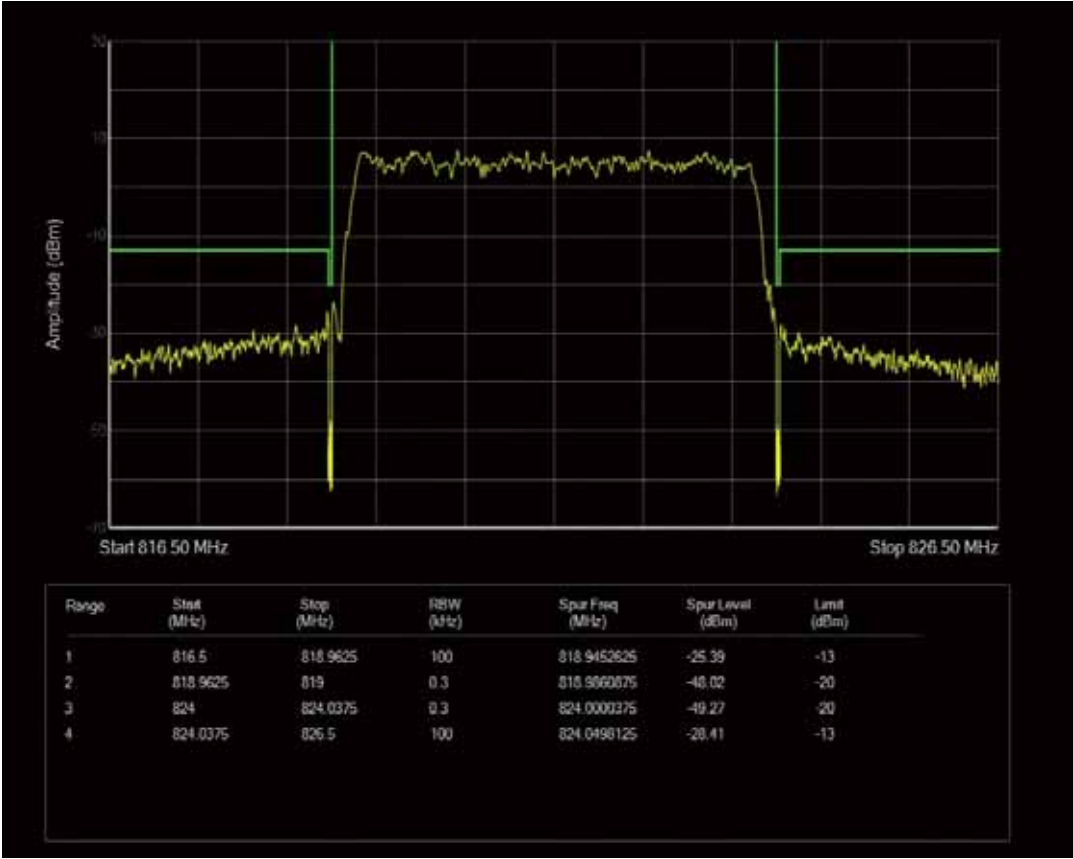
Band26a QAM16 BW=5MHz Channel=26765 RB Size=1 Position=#Max
