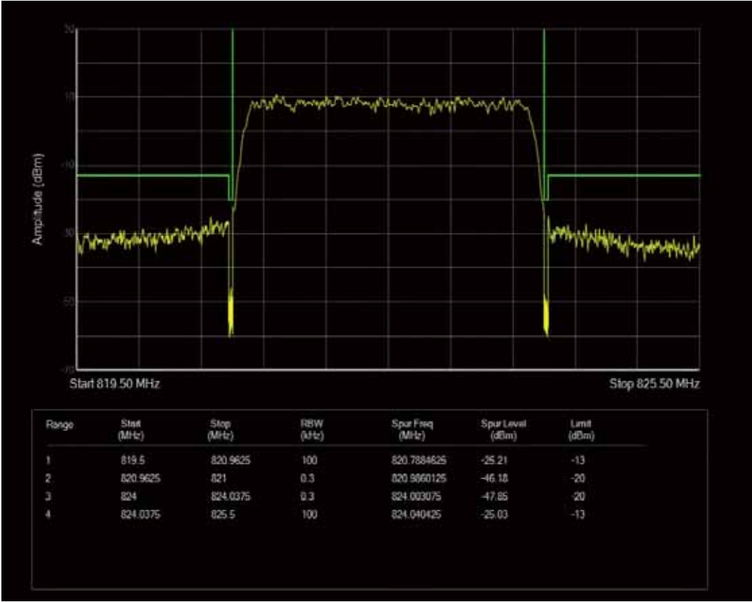
Band26a QAM16 BW=3MHz Channel=26775 RB Size=1 Position=#Max
