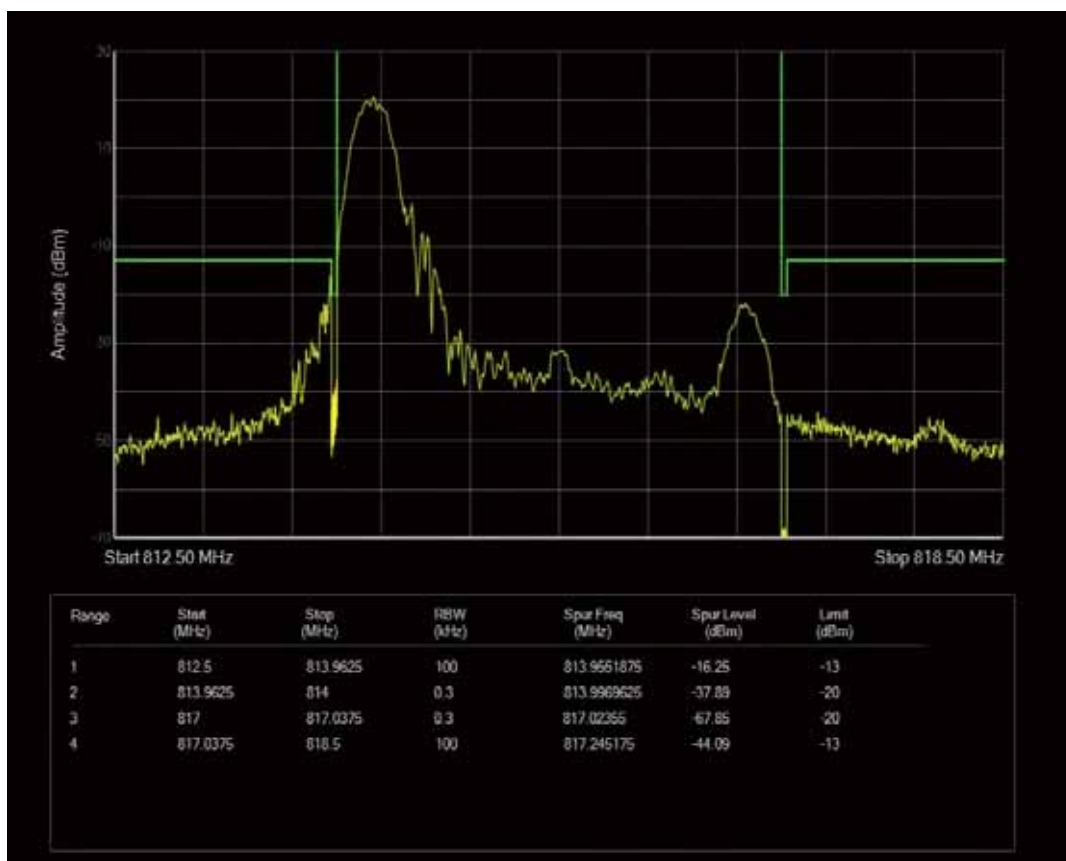
Band26a QAM16 BW=3MHz Channel=26705 RB Size=1 Position=#Max
