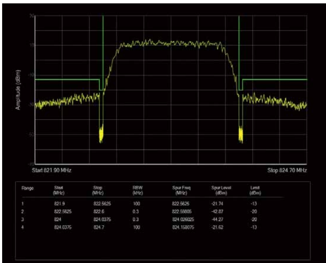
Band26a QPSK BW=3MHz Channel=26705 RB Size=1 Position=#Max
