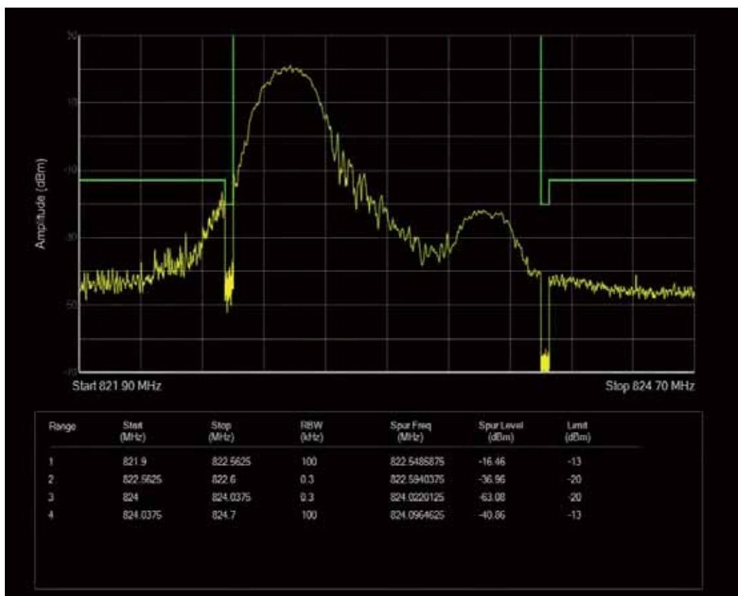
Band26a QAM16 BW=1.4MHz Channel=26783 RB Size=1 Position=#Max
