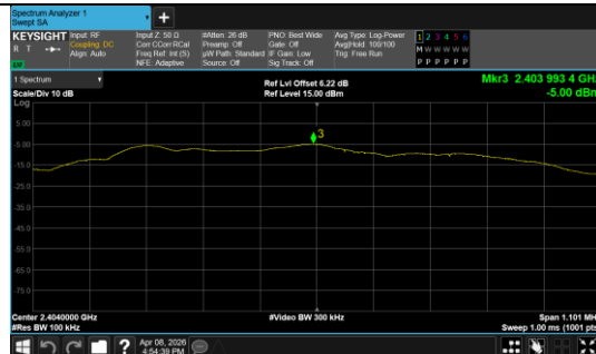
In-Band Reference Level BLE 2M_Channel 1
