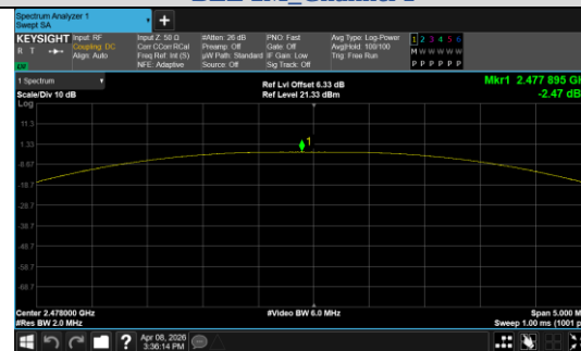
Peak Output Power BLE 2M_Channel 38
