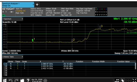
Out Of Band Emission(Left) 8DPSK_3-DH5_Channel Hopping
