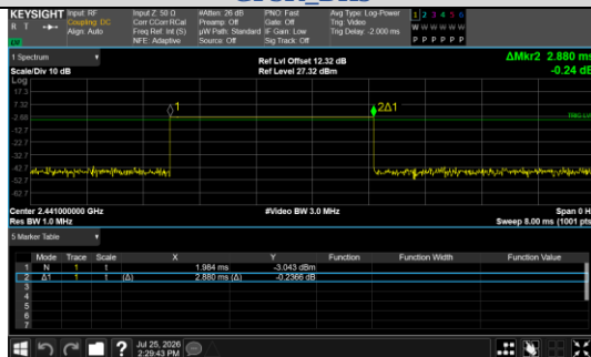
Pulse Width GFSK_DH5
