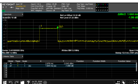
Pulse Width 8DPSK_3-DH3
