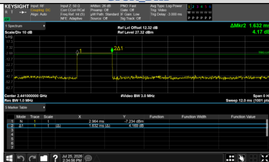
Pulse Width GFSK_DH3
