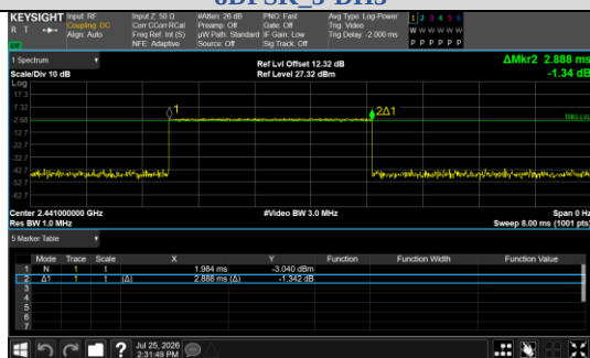
Pulse Width 8DPSK_3-DH5
