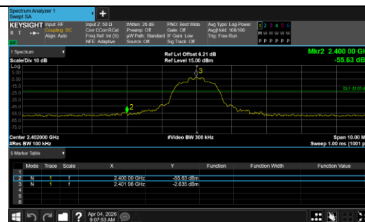
Out Of Band Emission \pi/4 DQPSK_2-DH5_Channel 0
