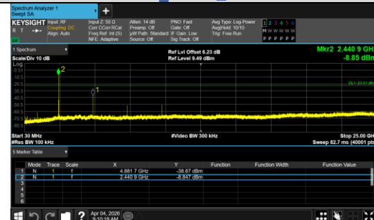
30.0 MHz - 25000.0 MHz π/4DQPSK 2-DH5 Channel 39
