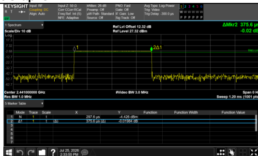
Pulse Width GFSK_DH1
