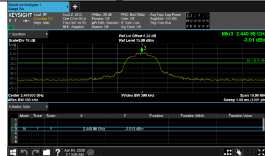
Out Of Band Emission π/4DQPSK 2-DH5 Channel 39
