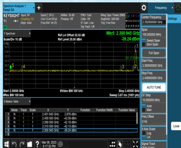
Lowest channel
