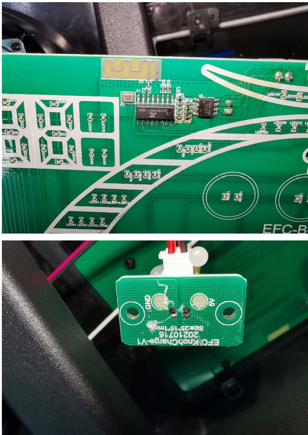
Inside view
